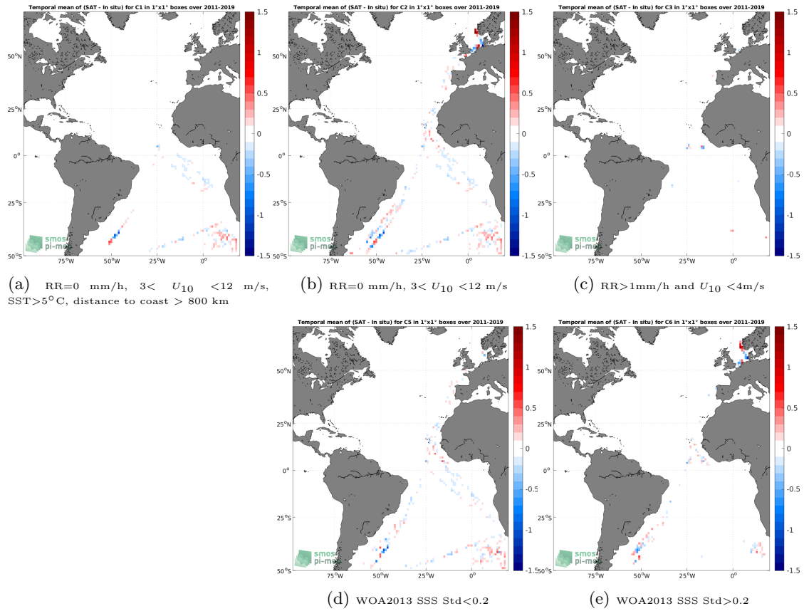
Figure 12: Temporal mean gridded over spatial boxes of size 1^\circ \times 1^\circ of \Delta SSS (SMAP SSS L4 OI v2 - 7 Days (ESR) - TSG (Polarstern)) for 5 different subdatasets corresponding to:RR=0 mm/h, 3 < U_{10} < 12 m/s, SST >5^\circ\text{C} , distance to coast > 800 km (a), RR=0 mm/h, 3 < U_{10} < 12 m/s (b), RR >1 mm/h and U_{10} < 4 m/s (c), WOA2013 SSS Std <0.2 (d), WOA2013 SSS Std >0.2 (e).
