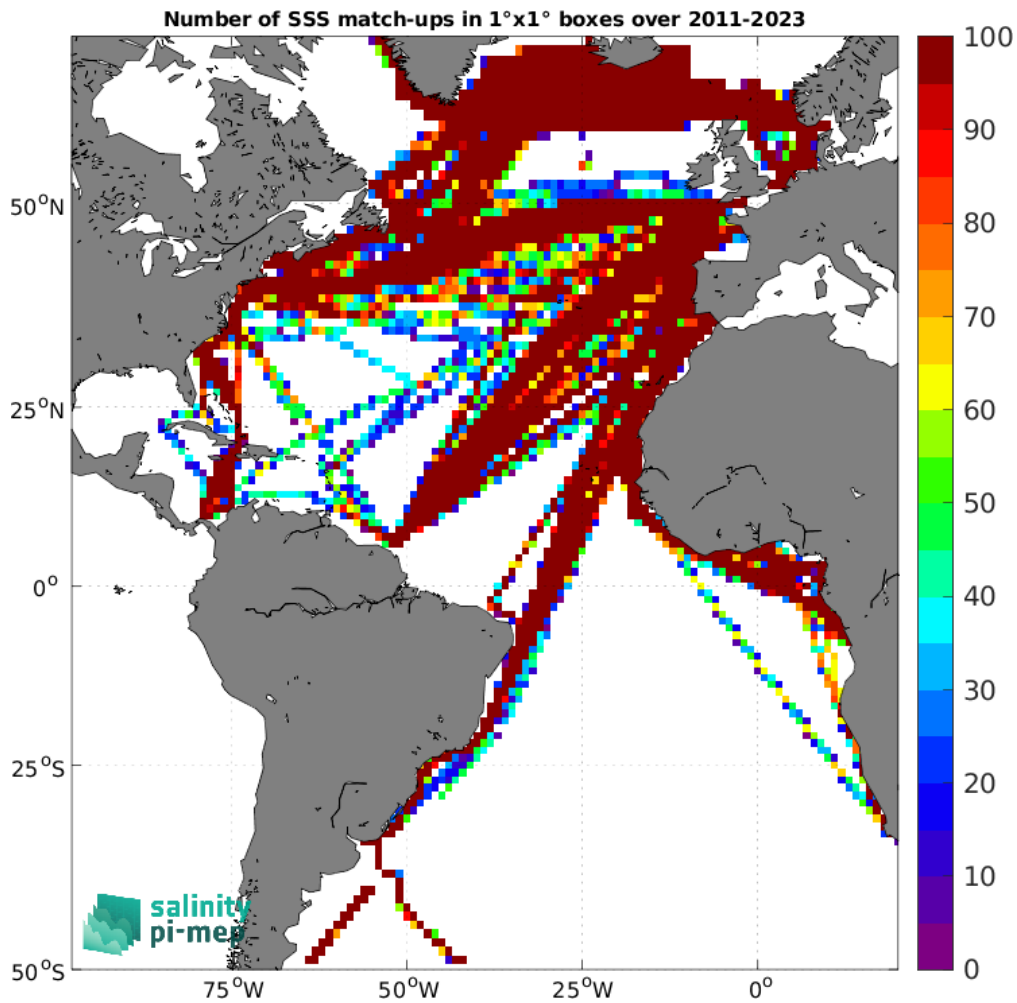
Figure 4: Number of SSS match-ups between TSG (LEGOS-DM) SSS and the SMAP SSS L4 OI v2 - 7 Days (ESR) SSS product for the Atlantic Ocean Pi-MEP region over 1^{\circ} \times 1^{\circ} boxes and for the full satellite product period.
