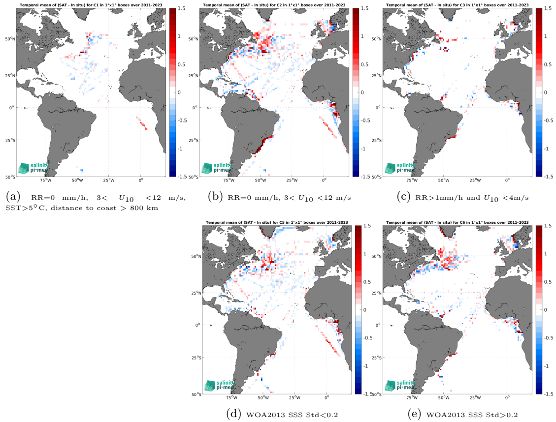
Figure 12: Temporal mean gridded over spatial boxes of size 1^\circ \times 1^\circ of \Delta\text{SSS} (SMAP SSS L4 OI v2 - 7 Days (ESR) - TSG (LEGOS-DM)) for 5 different subdatasets corresponding to:RR=0 mm/h, 3 < U_{10} < 12 m/s, SST >5^\circ\text{C} , distance to coast > 800 km (a), RR=0 mm/h, 3 < U_{10} < 12 m/s (b), RR >1 mm/h and U_{10} < 4 m/s (c), WOA2013 SSS Std <0.2 (d), WOA2013 SSS Std >0.2 (e).
