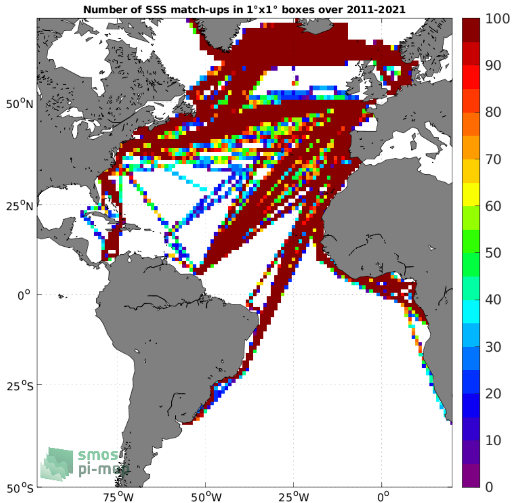
Figure 4: Number of SSS match-ups between TSG (LEGOS-DM) SSS and the SMAP SSS L4 OI v2 - 7 Days (ESR) SSS product for the Atlantic Ocean Pi-MEP region over 1°x1° boxes and for the full satellite product period.
