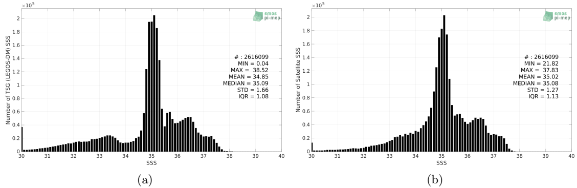
Figure 2: Histograms of SSS from TSG (LEGOS-DM) (a) and SMAP SSS L4 OI v2 - 7 Days (ESR) (b) considering all match-up pairs per bins of 0.1 over the Atlantic Ocean Pi-MEP region and for the full satellite product period.
