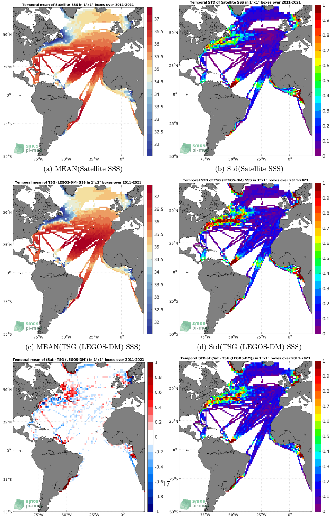
(e) MEAN( \Delta SSS) (Satellite - TSG (LEGOS-DM)) (f) Std( \Delta SSS) (Satellite - TSG (LEGOS-DM)) Figure 6: Temporal mean (left) and Std (right) of SSS from SMAP SSS L4 OI v2 - 7 Days (ESR) (top), TSG (LEGOS-DM) (middle), and of \Delta SSS (Satellite - TSG (LEGOS-DM)). Only match-up pairs are used to generate these maps.
