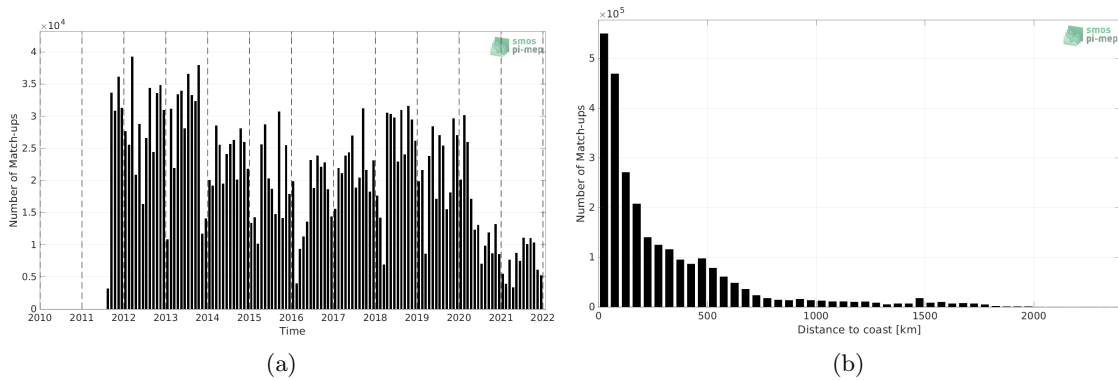
Figure 1: Number of match-ups between TSG (LEGOS-DM) and SMAP SSS L4 OI v2 - 7 Days (ESR) SSS as a function of time (a) and as function of the distance to coast (b) over the Atlantic Ocean Pi-MEP region and for the full satellite product period.
