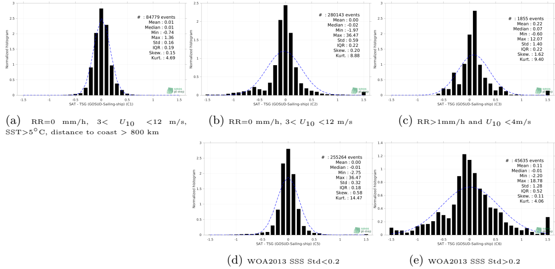
Figure 13: Normalized histogram of \Delta\text{SSS} (SMAP SSS L4 OI v2 - 7 Days (ESR) - TSG (GOSUD-Sailing-ship)) for 5 different subdatasets corresponding to: RR=0 mm/h, 3 < U_{10} < 12 m/s, SST>5°C, distance to coast > 800 km (a), RR=0 mm/h, 3 < U_{10} < 12 m/s (b), RR>1mm/h and U_{10} < 4 m/s (c), WOA2013 SSS Std<0.2 (d), WOA2013 SSS Std>0.2 (e).
