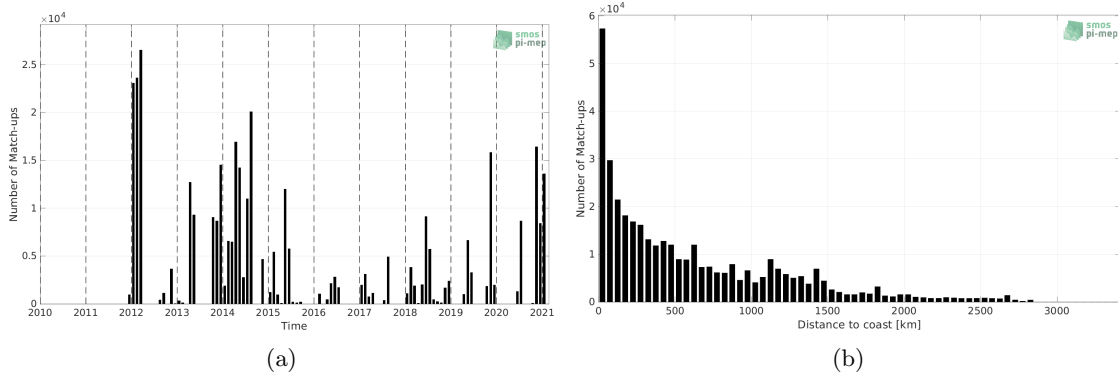
Figure 1: Number of match-ups between TSG (GOSUD-Sailing-ship) and SMAP SSS L4 OI v2 - 7 Days (ESR) SSS as a function of time (a) and as function of the distance to coast (b) over the Atlantic Ocean Pi-MEP region and for the full satellite product period.
