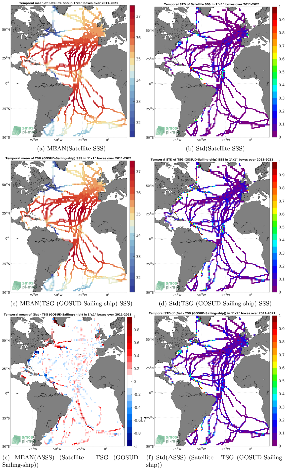
Figure 6: Temporal mean (left) and Std (right) of SSS from SMAP SSS L4 OI v2 - 7 Days (ESR) (top), TSG (GOSUD-Sailing-ship) (middle), and of \Delta SSS (Satellite - TSG (GOSUD-Sailing-ship)). Only match-up pairs are used to generate these maps.
