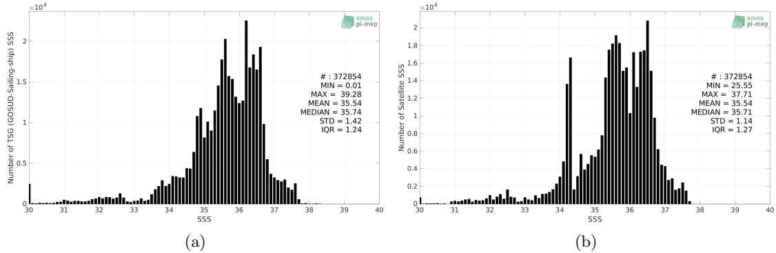
Figure 2: Histograms of SSS from TSG (GOSUD-Sailing-ship) (a) and SMAP SSS L4 OI v2 - 7 Days (ESR) (b) considering all match-up pairs per bins of 0.1 over the Atlantic Ocean Pi-MEP region and for the full satellite product period.
