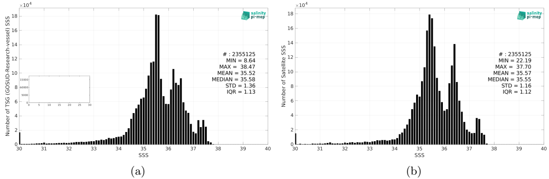
Figure 2: Histograms of SSS from TSG (GOSUD-Research-vessel) (a) and SMAP SSS L4 OI v2 - 7 Days (ESR) (b) considering all match-up pairs per bins of 0.1 over the Atlantic Ocean Pi-MEP region and for the full satellite product period.
