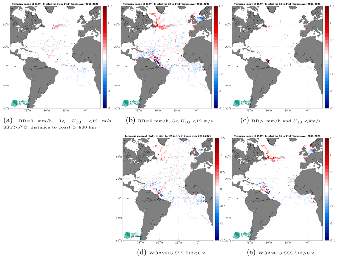
Figure 12: Temporal mean gridded over spatial boxes of size 1^\circ \times 1^\circ of \Delta SSS (SMAP SSS L4 OI v2 - 7 Days (ESR) - TSG (GOSUD-Research-vessel)) for 5 different subdatasets corresponding to:RR=0 mm/h, 3 < U_{10} < 12 m/s, SST>5°C, distance to coast > 800 km (a), RR=0 mm/h, 3 < U_{10} < 12 m/s (b), RR>1mm/h and U_{10} < 4 m/s (c), WOA2013 SSS Std<0.2 (d), WOA2013 SSS Std>0.2 (e).
