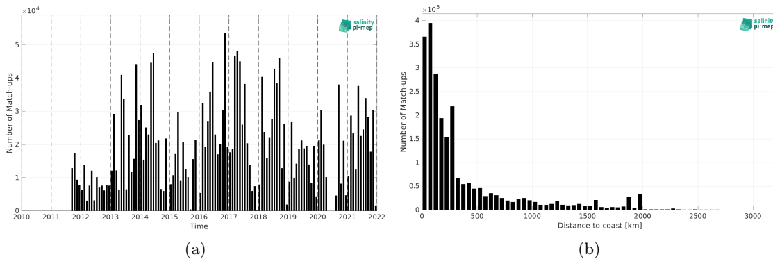
Figure 1: Number of match-ups between TSG (GOSUD-Research-vessel) and SMAP SSS L4 OI v2 - 7 Days (ESR) SSS as a function of time (a) and as function of the distance to coast (b) over the Atlantic Ocean Pi-MEP region and for the full satellite product period.
