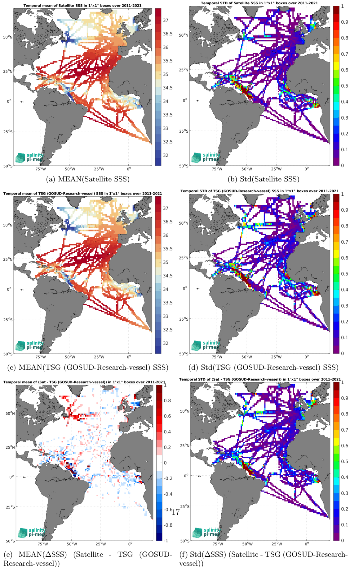
Figure 6: Temporal mean (left) and Std (right) of SSS from SMAP SSS L4 OI v2 - 7 Days (ESR) (top), TSG (GOSUD-Research-vessel) (middle), and of \Delta SSS (Satellite - TSG (GOSUD-Research-vessel)). Only match-up pairs are used to generate these maps.
