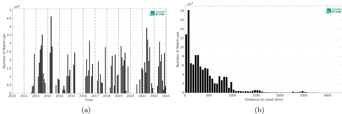
Figure 1: Number of match-ups between TSG (CSIC-UTM) and SMAP SSS L4 OI v2 - 7 Days (ESR) SSS as a function of time (a) and as function of the distance to coast (b) over the Atlantic Ocean Pi-MEP region and for the full satellite product period.
