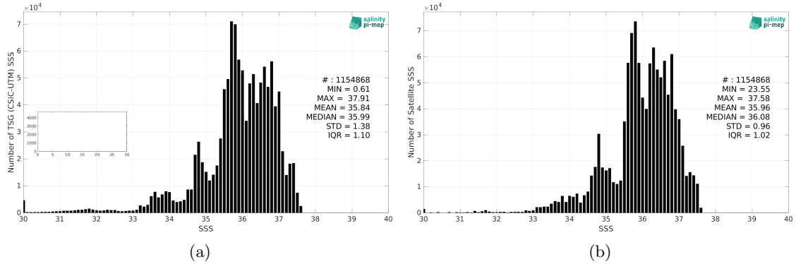
Figure 2: Histograms of SSS from TSG (CSIC-UTM) (a) and SMAP SSS L4 OI v2 - 7 Days (ESR) (b) considering all match-up pairs per bins of 0.1 over the Atlantic Ocean Pi-MEP region and for the full satellite product period.
