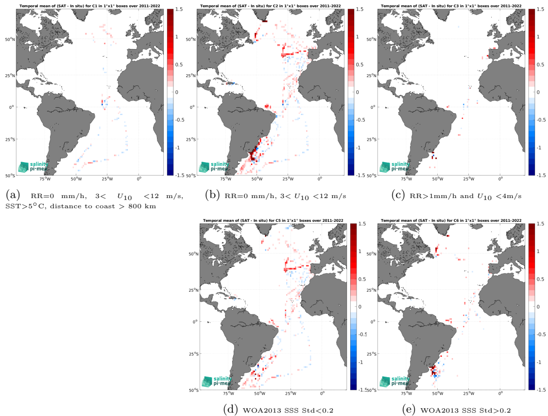
Figure 12: Temporal mean gridded over spatial boxes of size 1^\circ \times 1^\circ of \Delta SSS (SMAP SSS L4 OI v2 - 7 Days (ESR) - TSG (CSIC-UTM)) for 5 different subdatasets corresponding to:RR=0 mm/h, 3 < U_{10} < 12 m/s, SST >5^\circ\text{C} , distance to coast > 800 km (a), RR=0 mm/h, 3 < U_{10} < 12 m/s (b), RR >1 mm/h and U_{10} < 4 m/s (c), WOA2013 SSS Std <0.2 (d), WOA2013 SSS Std >0.2 (e).
