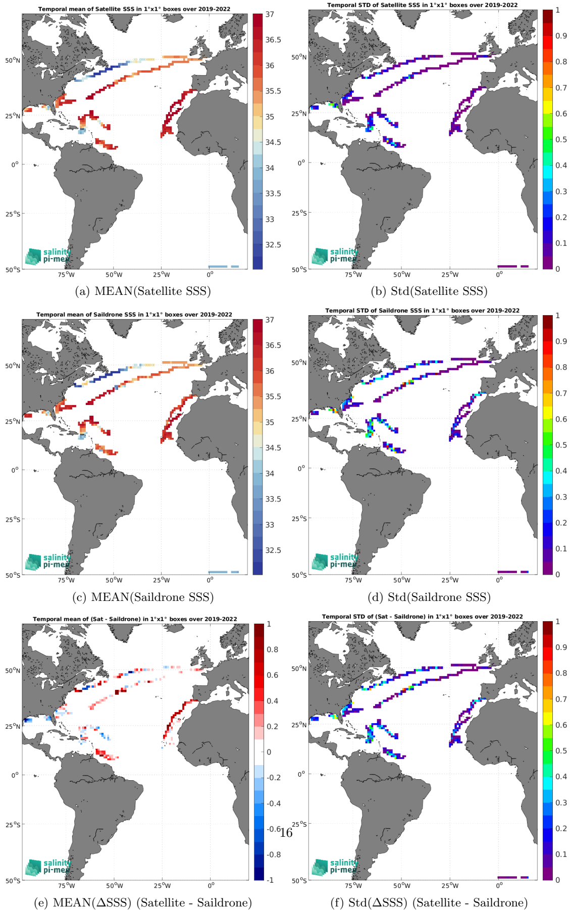
Figure 6: Temporal mean (left) and Std (right) of SSS from SMAP SSS L4 OI v2 - 7 Days (ESR) (top), Saildrone (middle), and of \Delta SSS (Satellite - Saildrone). Only match-up pairs are used to generate these maps.
