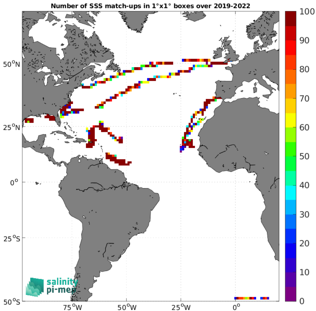
Figure 4: Number of SSS match-ups between Saildrone SSS and the SMAP SSS L4 OI v2 - 7 Days (ESR) SSS product for the Atlantic Ocean Pi-MEP region over 1^\circ \times 1^\circ boxes and for the full satellite product period.
