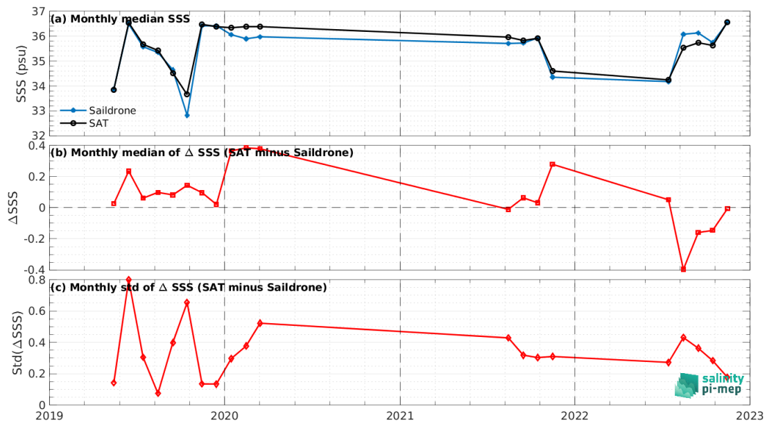
Figure 7: Time series of the monthly median SSS (top), median of \Delta SSS (Satellite - Sairdrone) and Std of \Delta SSS (Satellite - Sairdrone) over the Atlantic Ocean Pi-MEP region considering all match-ups collected by the Pi-MEP.
