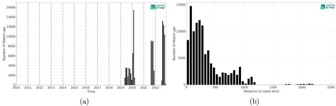
Figure 1: Number of match-ups between Saildrone and SMAP SSS L4 OI v2 - 7 Days (ESR) SSS as a function of time (a) and as function of the distance to coast (b) over the Atlantic Ocean Pi-MEP region and for the full satellite product period.
