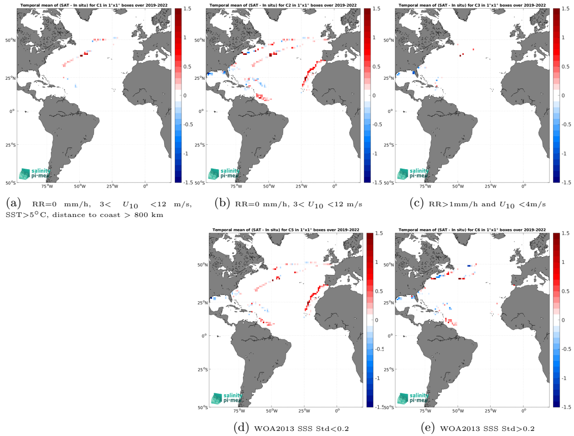
Figure 12: Temporal mean gridded over spatial boxes of size 1^\circ \times 1^\circ of \Delta SSS (SMAP SSS L4 OI v2 - 7 Days (ESR) - Saildrone) for 5 different subdatasets corresponding to:RR=0 mm/h, 3 < U_{10} < 12 m/s, SST >5^\circ\text{C} , distance to coast > 800 km (a), RR=0 mm/h, 3 < U_{10} < 12 m/s (b), RR >1 mm/h and U_{10} < 4 m/s (c), WOA2013 SSS Std <0.2 (d), WOA2013 SSS Std >0.2 (e).
