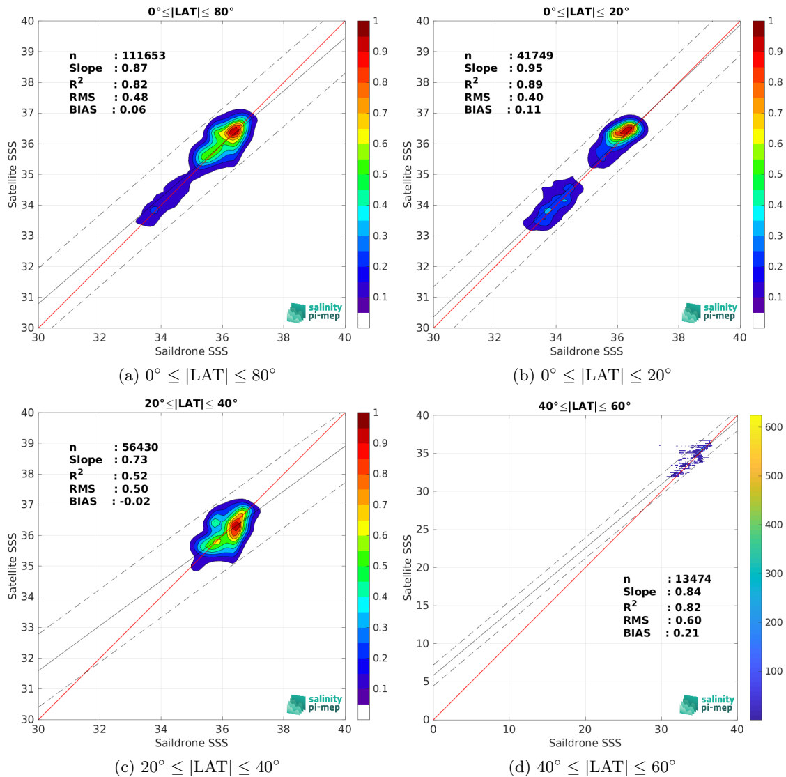
Figure 9: Contour maps of the concentration of SMAP SSS L4 OI v2 - 7 Days (ESR) SSS (y-axis) versus Saildrone SSS (x-axis) at match-up pairs for different latitude bands. For each plot, the red line shows x=y . The black thin and dashed lines indicate a linear fit through the data cloud and the \pm 95\% confidence levels, respectively. The number match-up pairs n , the slope and R^2 coefficient of the linear fit, the root mean square (RMS) and the mean bias between satellite and in situ data are indicated for each latitude band in each plots.
