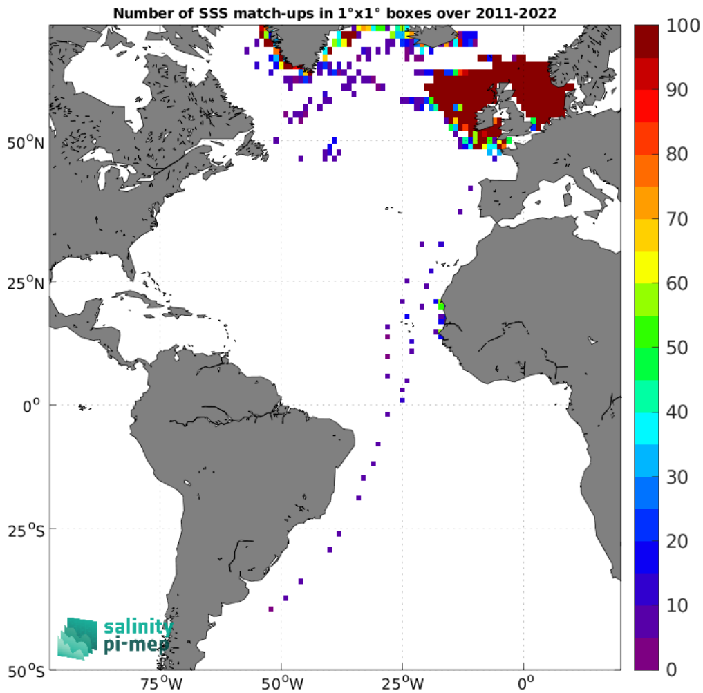
Figure 4: Number of SSS match-ups between ICES SSS and the SMAP SSS L4 OI v2 - 7 Days (ESR) SSS product for the Atlantic Ocean Pi-MEP region over 1^\circ \times 1^\circ boxes and for the full satellite product period.
