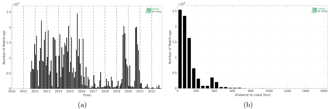
Figure 1: Number of match-ups between ICES and SMAP SSS L4 OI v2 - 7 Days (ESR) SSS as a function of time (a) and as function of the distance to coast (b) over the Atlantic Ocean Pi-MEP region and for the full satellite product period.
