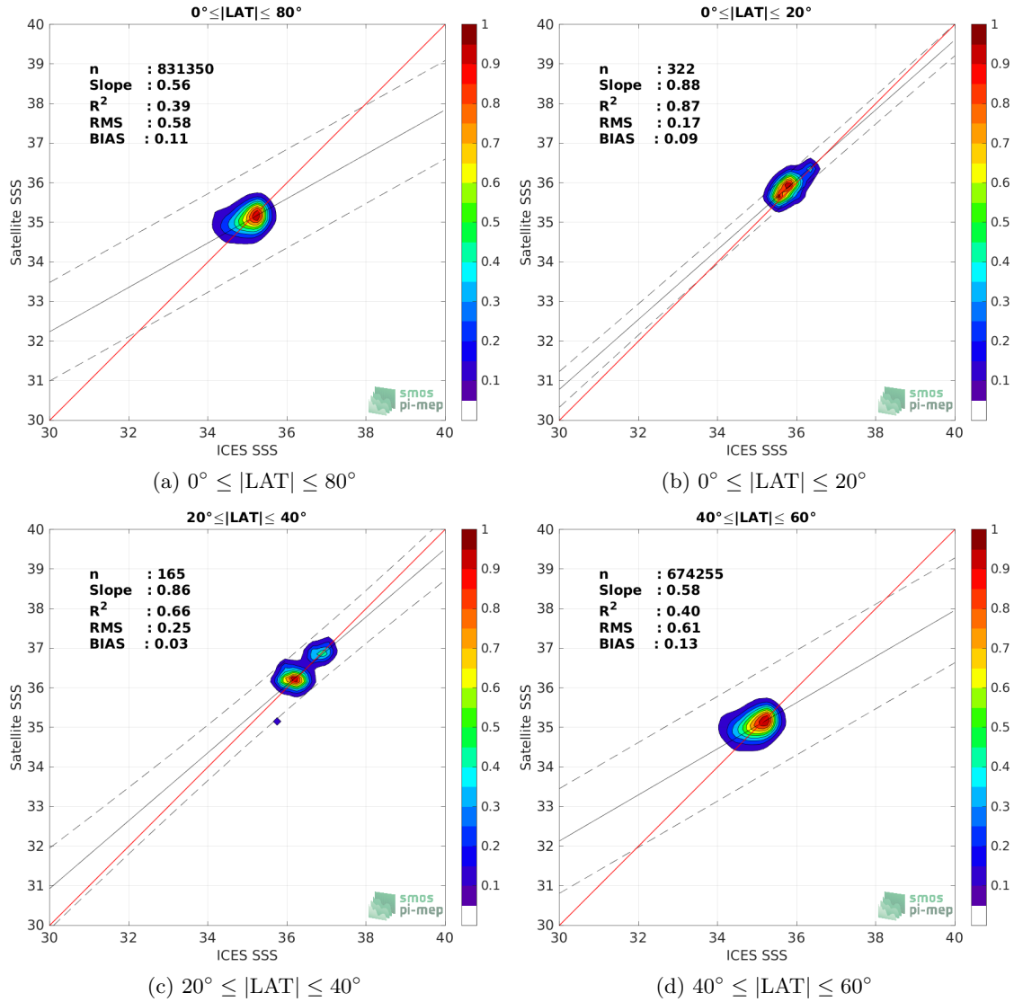
Figure 9: Contour maps of the concentration of SMAP SSS L4 OI v2 - 7 Days (ESR) SSS (y-axis) versus ICES SSS (x-axis) at match-up pairs for different latitude bands. For each plot, the red line shows x=y . The black thin and dashed lines indicate a linear fit through the data cloud and the \pm 95\% confidence levels, respectively. The number match-up pairs n , the slope and R^2 coefficient of the linear fit, the root mean square (RMS) and the mean bias between satellite and in situ data are indicated for each latitude band in each plots.
