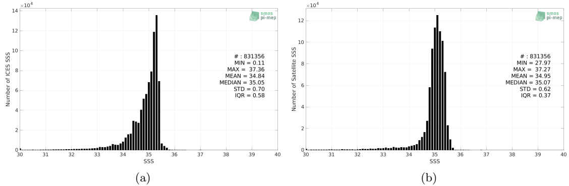
Figure 2: Histograms of SSS from ICES (a) and SMAP SSS L4 OI v2 - 7 Days (ESR) (b) considering all match-up pairs per bins of 0.1 over the Atlantic Ocean Pi-MEP region and for the full satellite product period.
