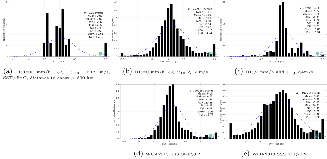
Figure 13: Normalized histogram of \Delta SSS (SMAP SSS L4 OI v2 - 7 Days (ESR) - ICES) for 5 different subdatasets corresponding to: RR=0 mm/h, 3 < U_{10} < 12 m/s, SST > 5°C, distance to coast > 800 km (a), RR=0 mm/h, 3 < U_{10} < 12 m/s (b), RR > 1mm/h and U_{10} < 4 m/s (c), WOA2013 SSS Std < 0.2 (d), WOA2013 SSS Std > 0.2 (e).
