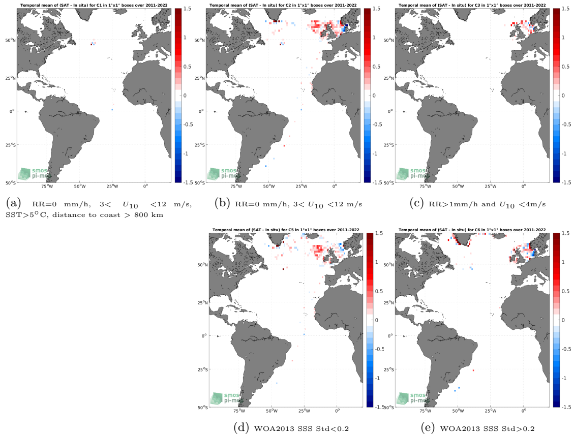
Figure 12: Temporal mean gridded over spatial boxes of size 1^\circ \times 1^\circ of \Delta SSS (SMAP SSS L4 OI v2 - 7 Days (ESR) - ICES) for 5 different subdatasets corresponding to:RR=0 mm/h, 3 < U_{10} < 12 m/s, SST >5^\circ\text{C} , distance to coast > 800 km (a), RR=0 mm/h, 3 < U_{10} < 12 m/s (b), RR >1 mm/h and U_{10} < 4 m/s (c), WOA2013 SSS Std <0.2 (d), WOA2013 SSS Std >0.2 (e).
