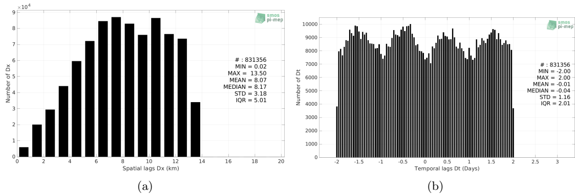
Figure 5: Histograms of the spatial (a) and temporal (b) lags between the location/time of the ICES measurement and the date of the corresponding SMAP SSS L4 OI v2 - 7 Days (ESR) SSS pixel.
