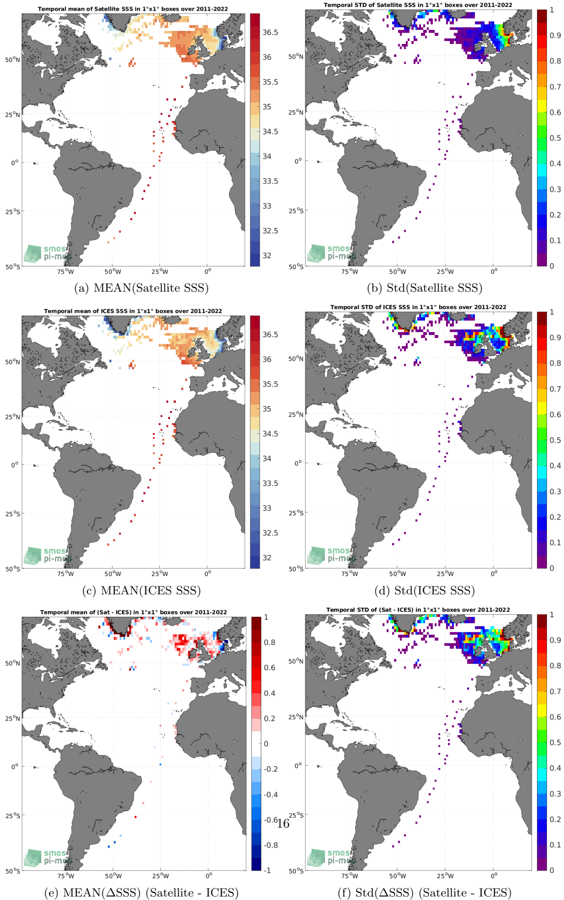
Figure 6: Temporal mean (left) and Std (right) of SSS from SMAP SSS L4 OI v2 - 7 Days (ESR) (top), ICES (middle), and of \Delta SSS (Satellite - ICES). Only match-up pairs are used to generate these maps.
