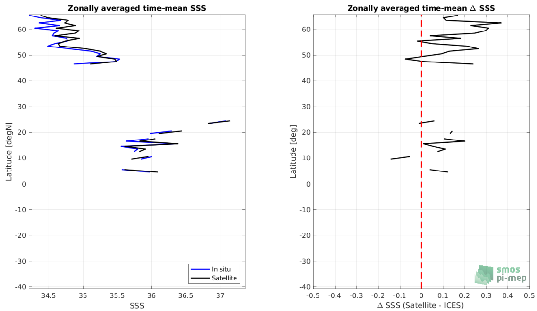
Figure 8: Left panel: Zonal mean SSS from SMAP SSS L4 OI v2 - 7 Days (ESR) satellite product (black) and from ICES (blue). Right panel: Zonal mean of \Delta SSS (Satellite - ICES) for all the collected Pi-MEP match-up pairs estimated over the full satellite product period.
