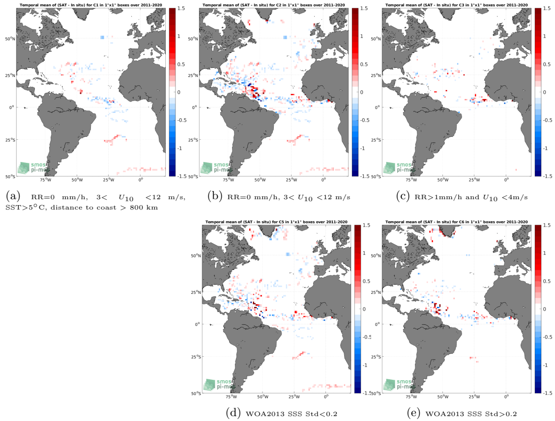
Figure 11: Temporal mean gridded over spatial boxes of size 1^\circ \times 1^\circ of \Delta SSS (SMAP SSS L4 OI v2 - 7 Days (ESR) - Surface drifters) for 5 different subdatasets corresponding to:RR=0 mm/h, 3 < U_{10} < 12 m/s, SST >5^\circ\text{C} , distance to coast > 800 km (a), RR=0 mm/h, 3 < U_{10} < 12 m/s (b), RR >1 mm/h and U_{10} < 4 m/s (c), WOA2013 SSS Std <0.2 (d), WOA2013 SSS Std >0.2 (e).
