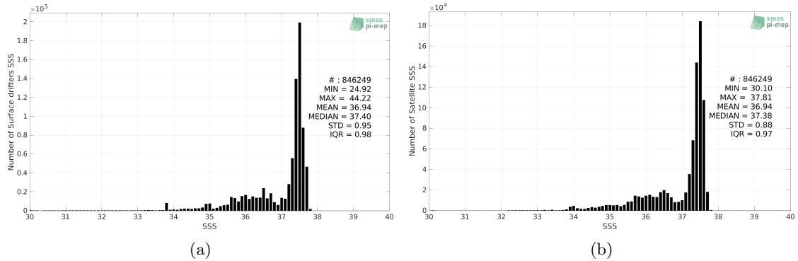
Figure 2: Histograms of SSS from Surface drifters (a) and SMAP SSS L4 OI v2 - 7 Days (ESR) (b) considering all match-up pairs per bins of 0.1 over the Atlantic Ocean Pi-MEP region and for the full satellite product period.
