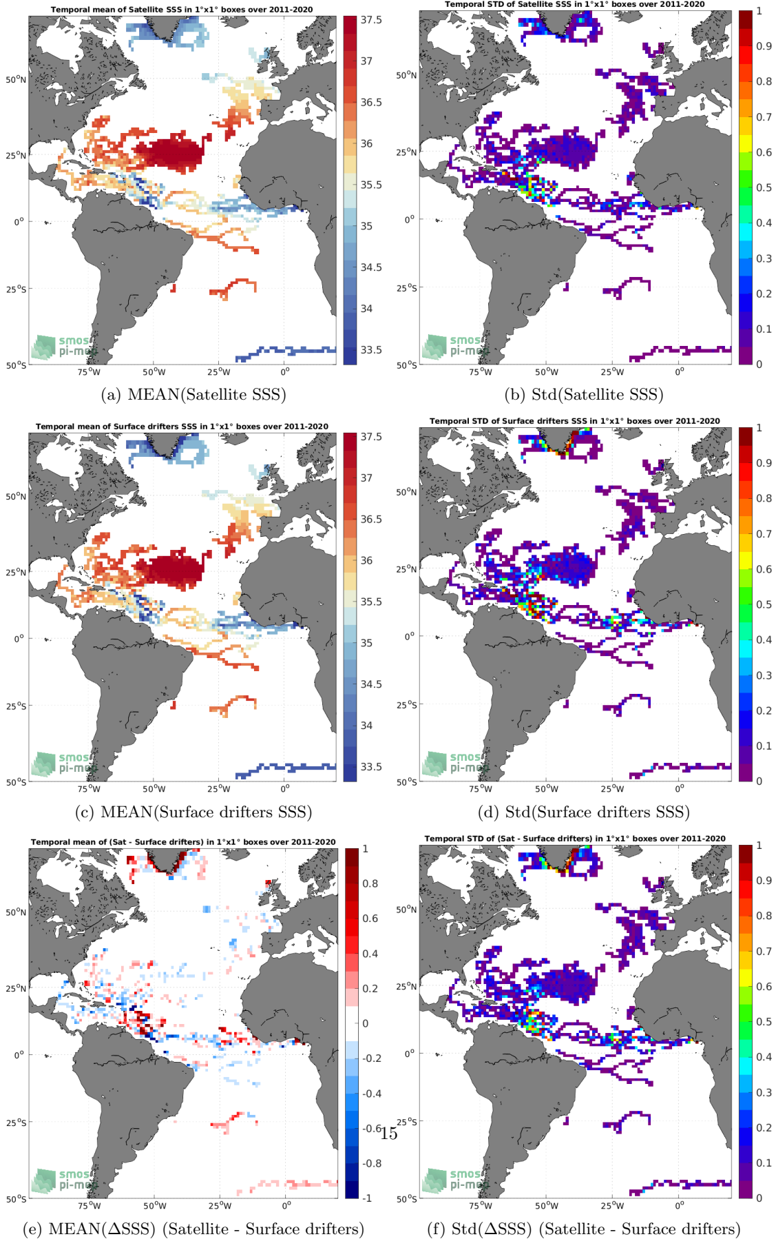
Figure 5: Temporal mean (left) and Std (right) of SSS from SMAP SSS L4 OI v2 - 7 Days (ESR) (top), Surface drifters (middle), and of \Delta SSS (Satellite - Surface drifters). Only match-up pairs are used to generate these maps.
