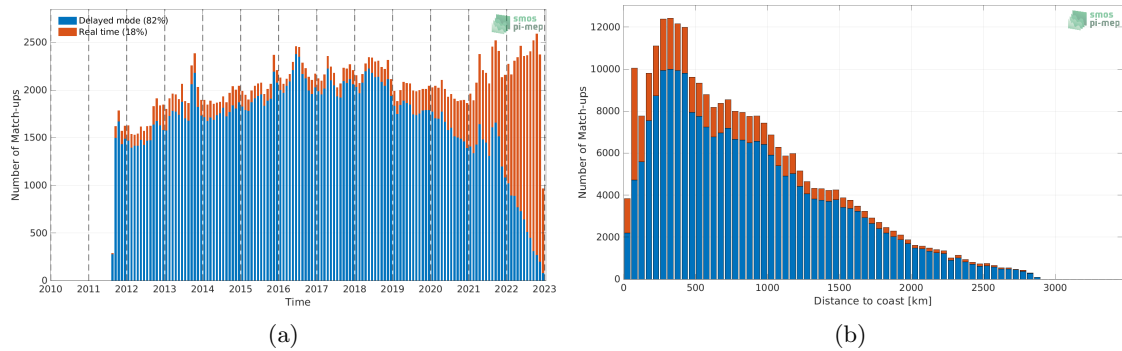
Figure 1: Number of match-ups between Argo and SMAP SSS L4 OI v2 - 7 Days (ESR) SSS as a function of time (a) and as function of the distance to coast (b) over the Atlantic Ocean Pi-MEP region and for the full satellite product period.
