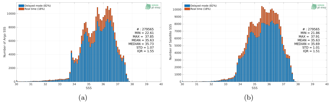
Figure 2: Histograms of SSS from Argo (a) and SMAP SSS L4 OI v2 - 7 Days (ESR) (b) considering all match-up pairs per bins of 0.1 over the Atlantic Ocean Pi-MEP region and for the full satellite product period.
