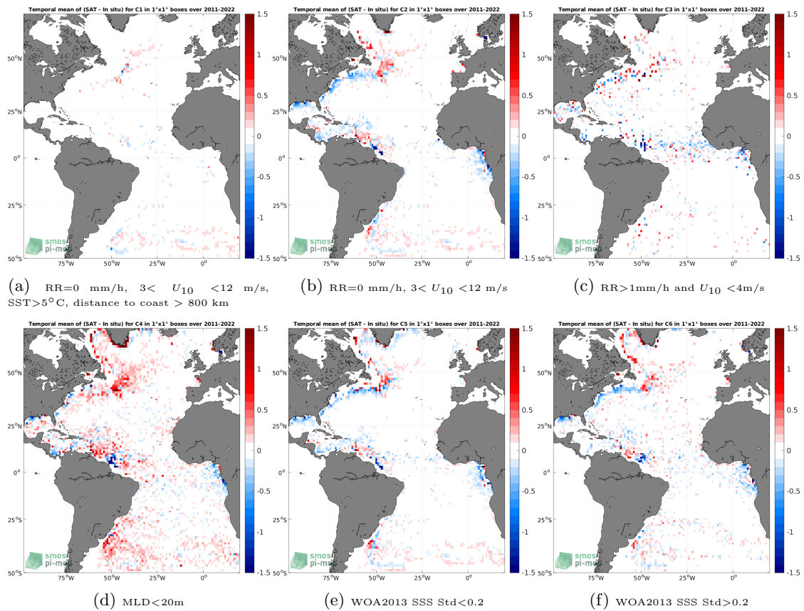
Figure 12: Temporal mean gridded over spatial boxes of size 1^\circ \times 1^\circ of \Delta SSS (SMAP SSS L4 OI v2 - 7 Days (ESR) - Argo) for 6 different subdatasets corresponding to:RR=0 mm/h, 3 < U_{10} < 12 m/s, SST >5^\circ C, distance to coast > 800 km (a), RR=0 mm/h, 3 < U_{10} < 12 m/s (b), RR >1 mm/h and U_{10} < 4 m/s (c),MLD <20 m (d),WOA2013 SSS Std <0.2 (e),WOA2013 SSS Std >0.2 (f).
