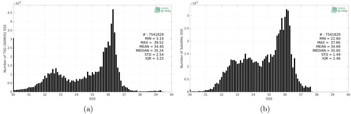
Figure 2: Histograms of SSS from TSG (SAMOS) (a) and SMAP SSS L4 OI v2 - Monthly (IPRC) (b) considering all match-up pairs per bins of 0.1 over the Atlantic Ocean Pi-MEP region and for the full satellite product period.
