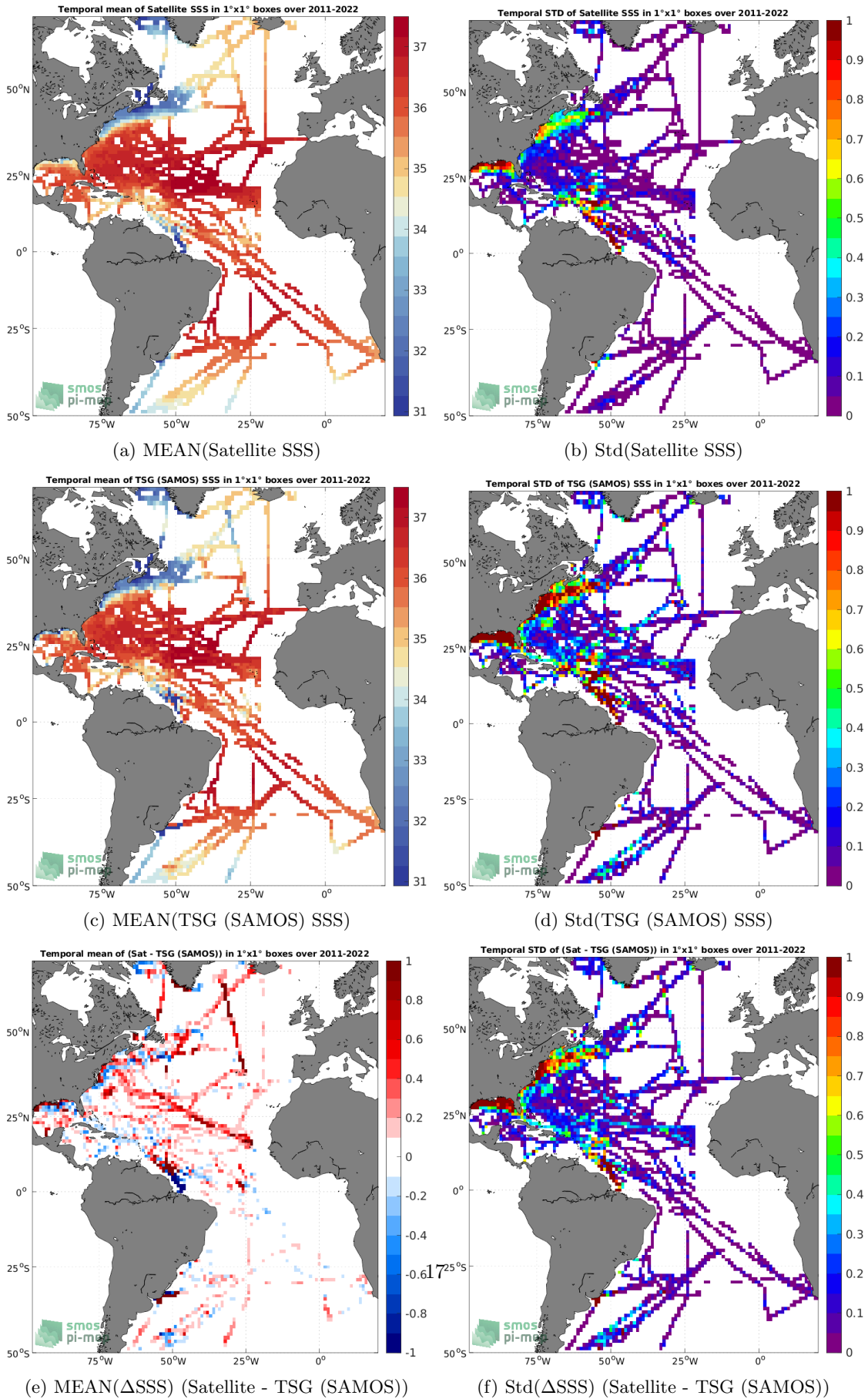
Figure 6: Temporal mean (left) and Std (right) of SSS from SMAP SSS L4 OI v2 - Monthly (IPRC) (top), TSG (SAMOS) (middle), and of \Delta SSS (Satellite - TSG (SAMOS)). Only match-up pairs are used to generate these maps.
