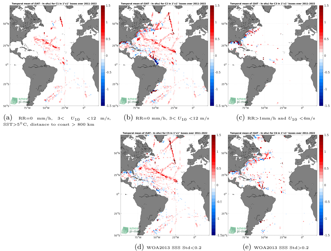
Figure 12: Temporal mean gridded over spatial boxes of size 1^\circ \times 1^\circ of \Delta SSS (SMAP SSS L4 OI v2 - Monthly (IPRC) - TSG (SAMOS)) for 5 different subdatasets corresponding to:RR=0 mm/h, 3 < U_{10} < 12 m/s, SST >5^\circ\text{C} , distance to coast > 800 km (a), RR=0 mm/h, 3 < U_{10} < 12 m/s (b), RR >1 mm/h and U_{10} < 4 m/s (c), WOA2013 SSS Std <0.2 (d), WOA2013 SSS Std >0.2 (e).
