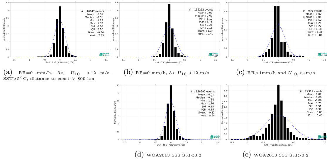
Figure 13: Normalized histogram of \Delta\text{SSS} (SMAP SSS L4 OI v2 - Monthly (IPRC) - TSG (Polarstern)) for 5 different subdatasets corresponding to: RR=0 mm/h, 3 < U_{10} < 12 m/s, SST>5°C, distance to coast > 800 km (a), RR=0 mm/h, 3 < U_{10} < 12 m/s (b), RR>1mm/h and U_{10} < 4 m/s (c), WOA2013 SSS Std<0.2 (d), WOA2013 SSS Std>0.2 (e).
