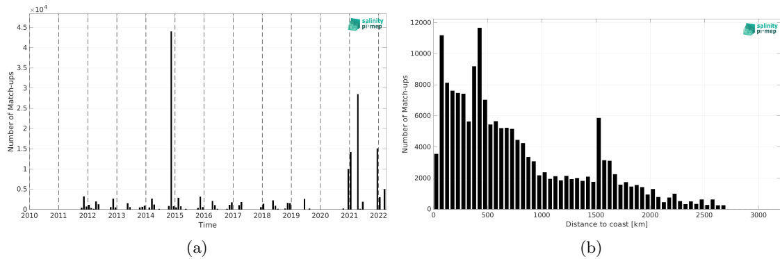
Figure 1: Number of match-ups between TSG (Polarstern) and SMAP SSS L4 OI v2 - Monthly (IPRC) SSS as a function of time (a) and as function of the distance to coast (b) over the Atlantic Ocean Pi-MEP region and for the full satellite product period.
