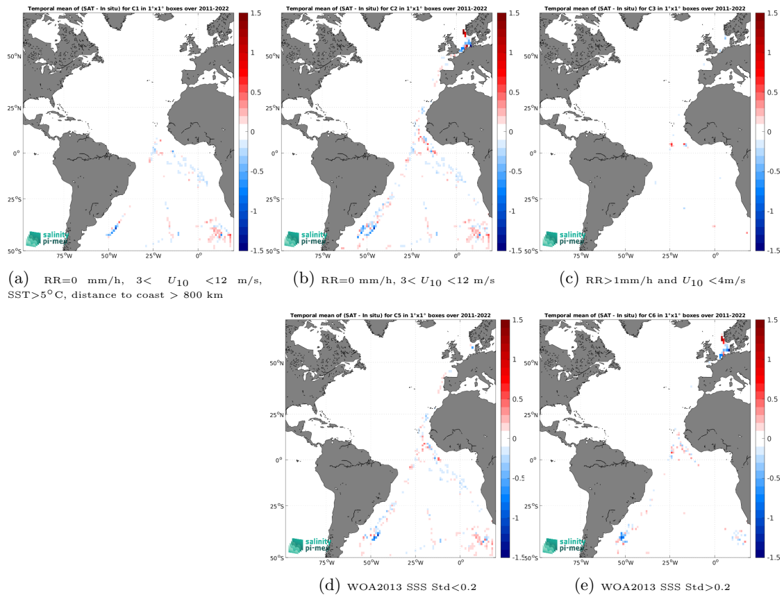
Figure 12: Temporal mean gridded over spatial boxes of size 1^\circ \times 1^\circ of \Delta SSS (SMAP SSS L4 OI v2 - Monthly (IPRC) - TSG (Polarstern)) for 5 different subdatasets corresponding to:RR=0 mm/h, 3 < U_{10} < 12 m/s, SST >5^\circ\text{C} , distance to coast > 800 km (a), RR=0 mm/h, 3 < U_{10} < 12 m/s (b), RR >1 mm/h and U_{10} < 4 m/s (c), WOA2013 SSS Std <0.2 (d), WOA2013 SSS Std >0.2 (e).
