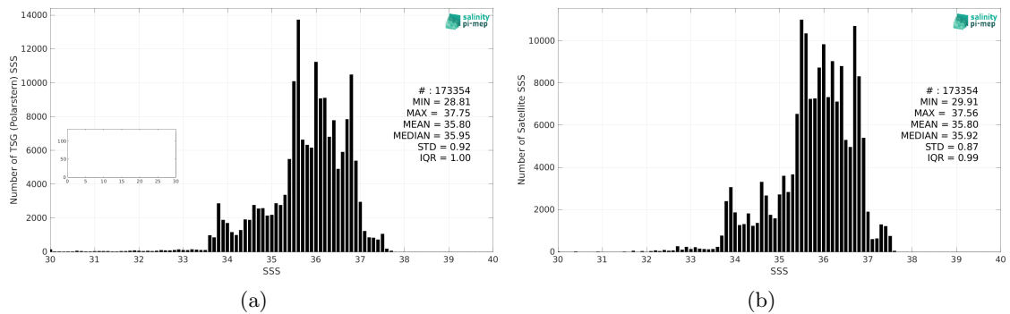
Figure 2: Histograms of SSS from TSG (Polarstern) (a) and SMAP SSS L4 OI v2 - Monthly (IPRC) (b) considering all match-up pairs per bins of 0.1 over the Atlantic Ocean Pi-MEP region and for the full satellite product period.
