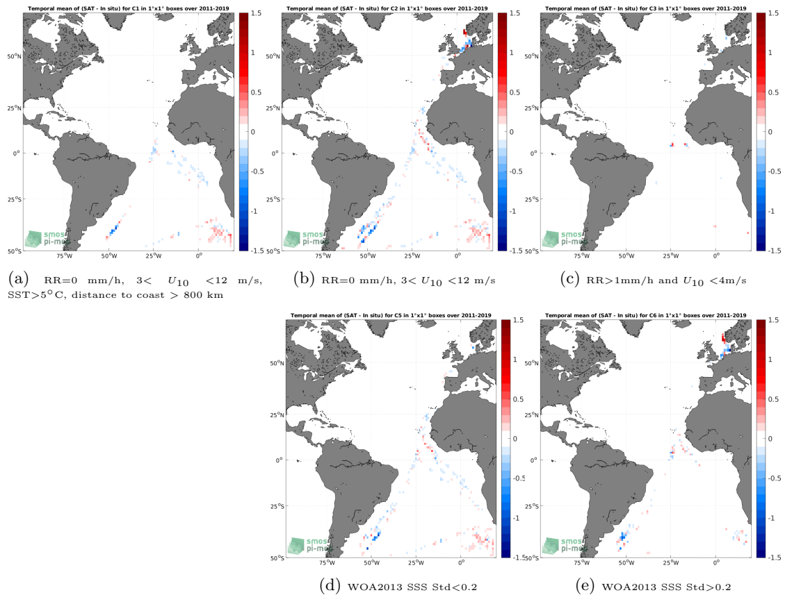
Figure 12: Temporal mean gridded over spatial boxes of size 1^\circ \times 1^\circ of \Delta SSS (SMAP SSS L4 OI v2 - Monthly (IPRC) - TSG (Polarstern)) for 5 different subdatasets corresponding to:RR=0 mm/h, 3 < U_{10} < 12 m/s, SST >5^\circ\text{C} , distance to coast > 800 km (a), RR=0 mm/h, 3 < U_{10} < 12 m/s (b), RR >1 mm/h and U_{10} < 4 m/s (c), WOA2013 SSS Std <0.2 (d), WOA2013 SSS Std >0.2 (e).
