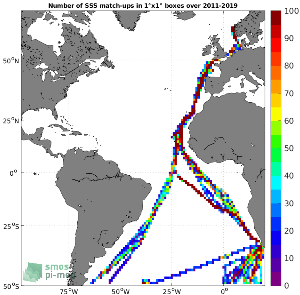
Figure 4: Number of SSS match-ups between TSG (Polarstern) SSS and the SMAP SSS L4 OI v2 - Monthly (IPRC) SSS product for the Atlantic Ocean Pi-MEP region over 1°x1° boxes and for the full satellite product period.
