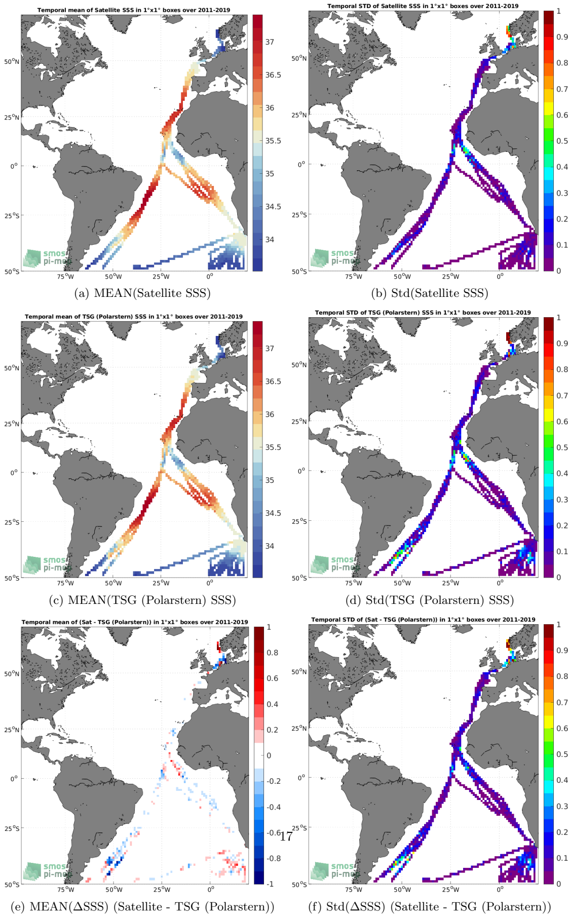
Figure 6: Temporal mean (left) and Std (right) of SSS from SMAP SSS L4 OI v2 - Monthly (IPRC) (top), TSG (Polarstern) (middle), and of \Delta SSS (Satellite - TSG (Polarstern)). Only match-up pairs are used to generate these maps.
