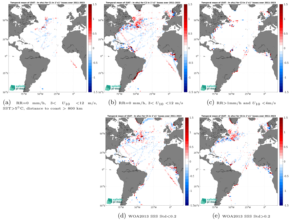
Figure 12: Temporal mean gridded over spatial boxes of size 1^\circ \times 1^\circ of \Delta SSS (SMAP SSS L4 OI v2 - Monthly (IPRC) - TSG (LEGOS-DM)) for 5 different subdatasets corresponding to:RR=0 mm/h, 3 < U_{10} < 12 m/s, SST >5^\circ\text{C} , distance to coast > 800 km (a), RR=0 mm/h, 3 < U_{10} < 12 m/s (b), RR >1 mm/h and U_{10} < 4 m/s (c), WOA2013 SSS Std <0.2 (d), WOA2013 SSS Std >0.2 (e).
