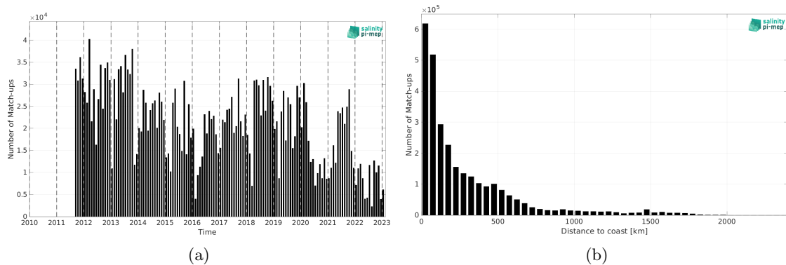
Figure 1: Number of match-ups between TSG (LEGOS-DM) and SMAP SSS L4 OI v2 - Monthly (IPRC) SSS as a function of time (a) and as function of the distance to coast (b) over the Atlantic Ocean Pi-MEP region and for the full satellite product period.
