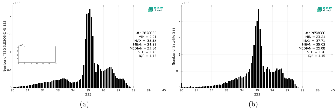
Figure 2: Histograms of SSS from TSG (LEGOS-DM) (a) and SMAP SSS L4 OI v2 - Monthly (IPRC) (b) considering all match-up pairs per bins of 0.1 over the Atlantic Ocean Pi-MEP region and for the full satellite product period.
