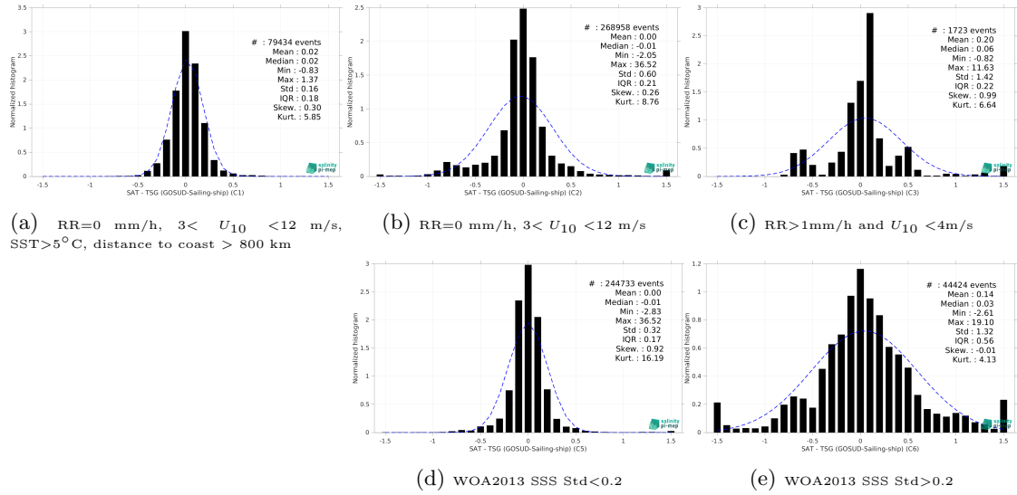
Figure 13: Normalized histogram of \Delta\text{SSS} (SMAP SSS L4 OI v2 - Monthly (IPRC) - TSG (GOSUD-Sailing-ship)) for 5 different subdatasets corresponding to: RR=0 mm/h, 3 < U_{10} < 12 m/s, SST>5°C, distance to coast > 800 km (a), RR=0 mm/h, 3 < U_{10} < 12 m/s (b), RR>1mm/h and U_{10} < 4 m/s (c), WOA2013 SSS Std<0.2 (d), WOA2013 SSS Std>0.2 (e).
