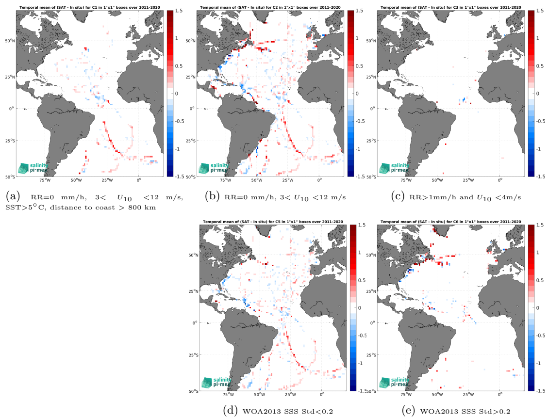
Figure 12: Temporal mean gridded over spatial boxes of size 1^\circ \times 1^\circ of \Delta\text{SSS} (SMAP SSS L4 OI v2 - Monthly (IPRC) - TSG (GOSUD-Sailing-ship)) for 5 different subdatasets corresponding to:RR=0 mm/h, 3 < U_{10} < 12 m/s, SST>5°C, distance to coast > 800 km (a), RR=0 mm/h, 3 < U_{10} < 12 m/s (b), RR>1mm/h and U_{10} < 4 m/s (c), WOA2013 SSS Std<0.2 (d), WOA2013 SSS Std>0.2 (e).
