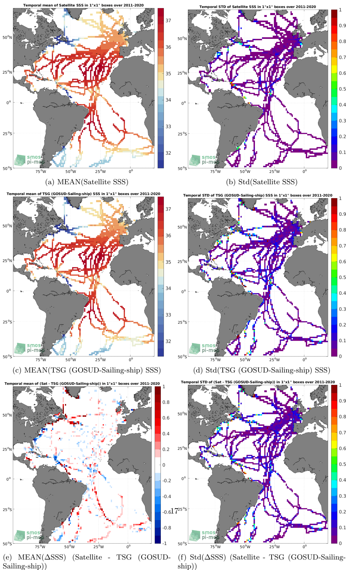
Figure 6: Temporal mean (left) and Std (right) of SSS from SMAP SSS L4 OI v2 - Monthly (IPRC) (top), TSG (GOSUD-Sailing-ship) (middle), and of \Delta SSS (Satellite - TSG (GOSUD-Sailing-ship)). Only match-up pairs are used to generate these maps.
