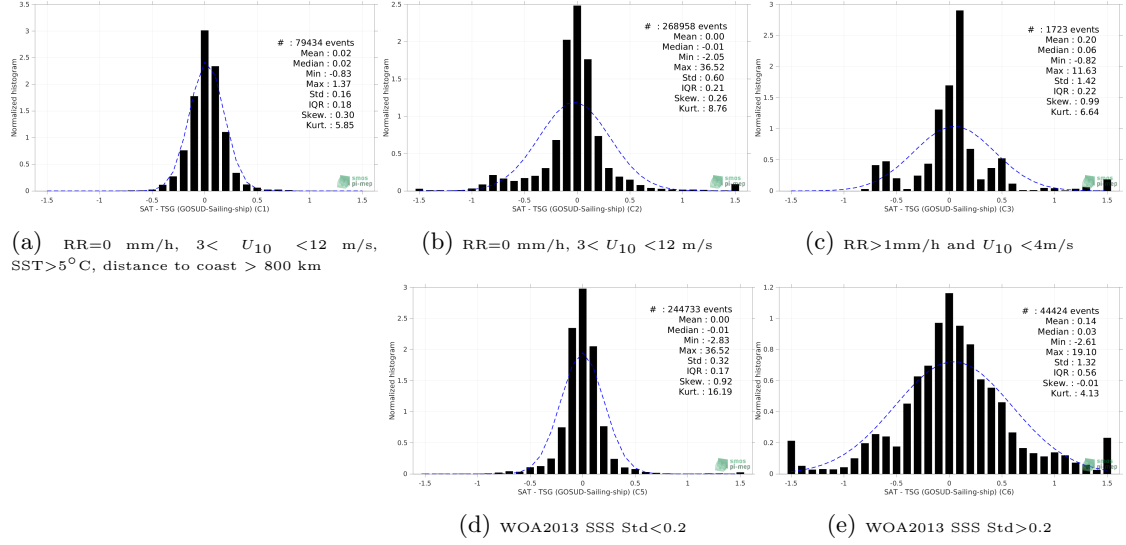
Figure 13: Normalized histogram of \Delta\text{SSS} (SMAP SSS L4 OI v2 - Monthly (IPRC) - TSG (GOSUD-Sailing-ship)) for 5 different subdatasets corresponding to: RR=0 mm/h, 3 < U_{10} < 12 m/s, SST>5°C, distance to coast > 800 km (a), RR=0 mm/h, 3 < U_{10} < 12 m/s (b), RR>1mm/h and U_{10} < 4 m/s (c), WOA2013 SSS Std<0.2 (d), WOA2013 SSS Std>0.2 (e).
