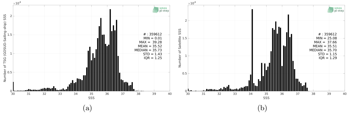
Figure 2: Histograms of SSS from TSG (GOSUD-Sailing-ship) (a) and SMAP SSS L4 OI v2 - Monthly (IPRC) (b) considering all match-up pairs per bins of 0.1 over the Atlantic Ocean Pi-MEP region and for the full satellite product period.
