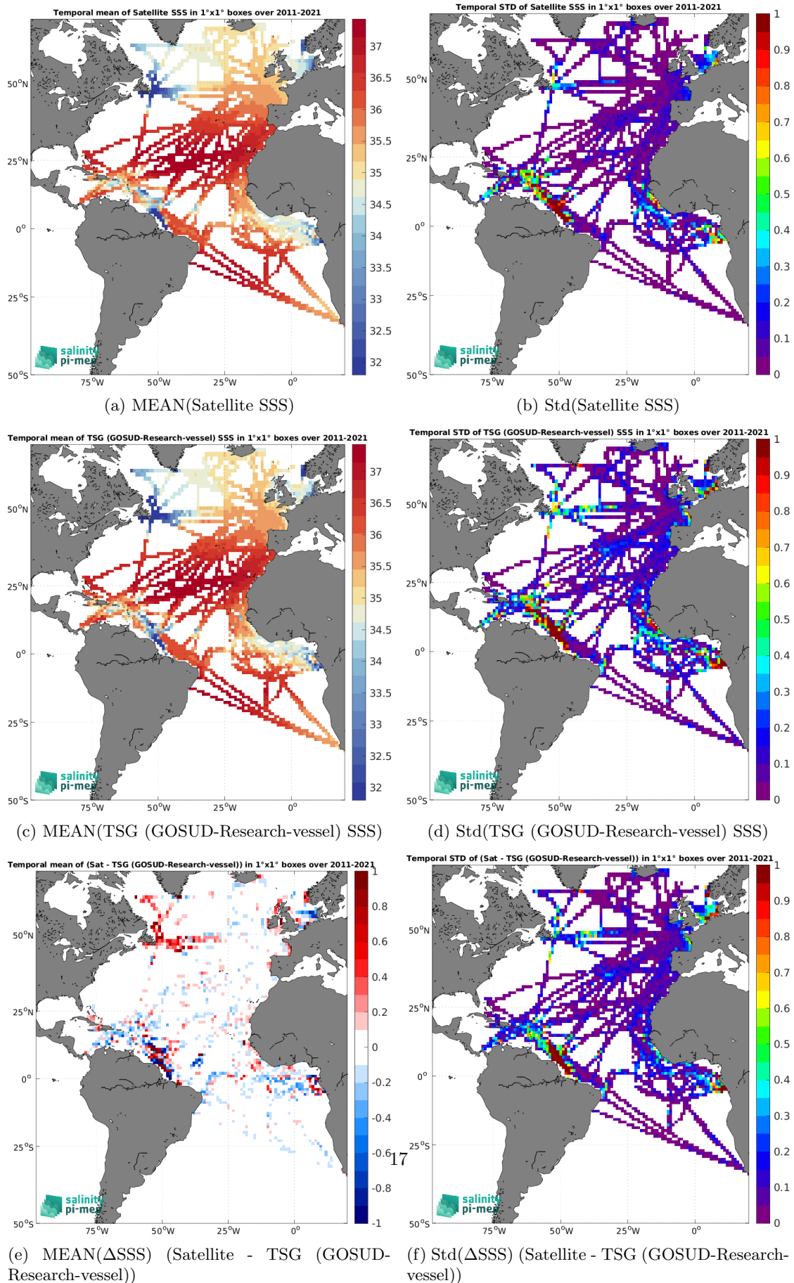
Figure 6: Temporal mean (left) and Std (right) of SSS from SMAP SSS L4 OI v2 - Monthly (IPRC) (top), TSG (GOSUD-Research-vessel) (middle), and of \Delta SSS (Satellite - TSG (GOSUD-Research-vessel)). Only match-up pairs are used to generate these maps.
