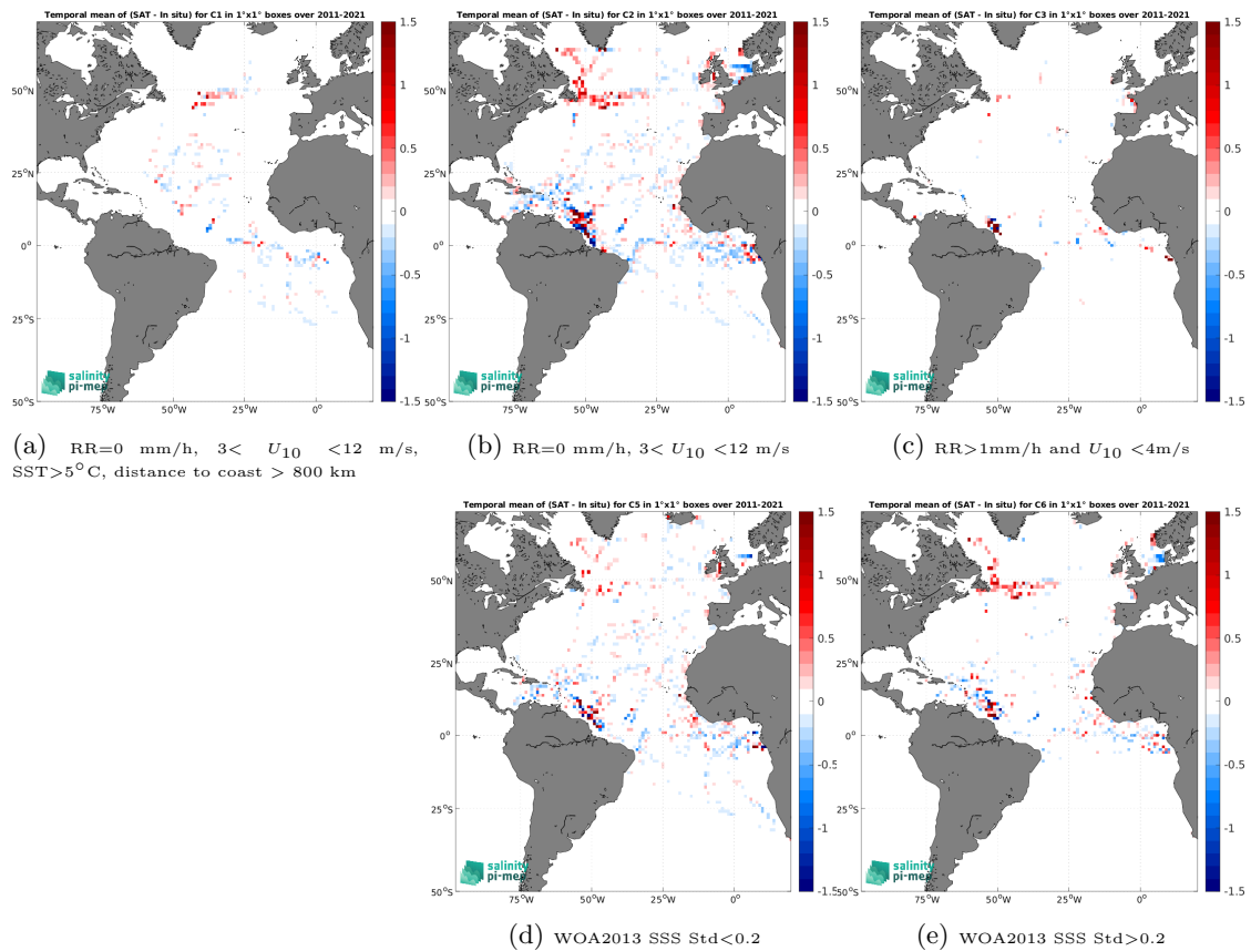
Figure 12: Temporal mean gridded over spatial boxes of size 1^\circ \times 1^\circ of \Delta\text{SSS} (SMAP SSS L4 OI v2 - Monthly (IPRC) - TSG (GOSUD-Research-vessel)) for 5 different subdatasets corresponding to:RR=0 mm/h, 3 < U_{10} < 12 m/s, SST>5°C, distance to coast > 800 km (a), RR=0 mm/h, 3 < U_{10} < 12 m/s (b), RR>1mm/h and U_{10} < 4 m/s (c), WOA2013 SSS Std<0.2 (d), WOA2013 SSS Std>0.2 (e).
