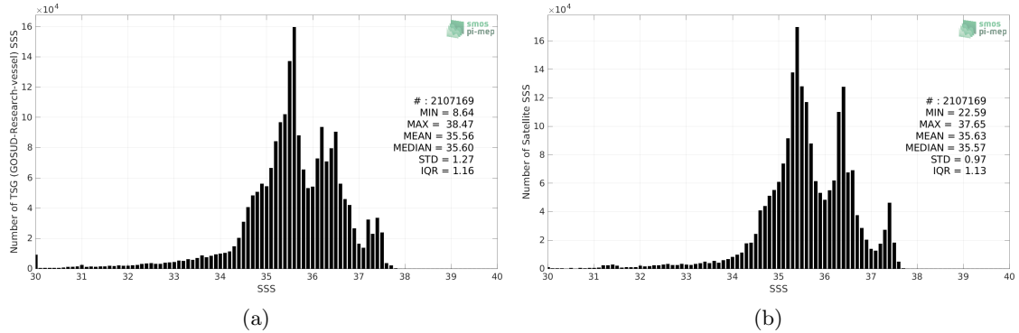
Figure 2: Histograms of SSS from TSG (GOSUD-Research-vessel) (a) and SMAP SSS L4 OI v2 - Monthly (IPRC) (b) considering all match-up pairs per bins of 0.1 over the Atlantic Ocean Pi-MEP region and for the full satellite product period.
