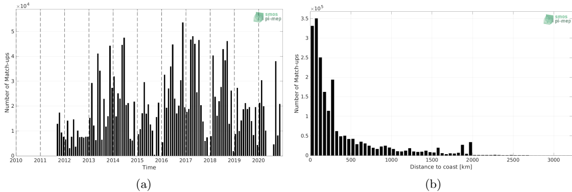
Figure 1: Number of match-ups between TSG (GOSUD-Research-vessel) and SMAP SSS L4 OI v2 - Monthly (IPRC) SSS as a function of time (a) and as function of the distance to coast (b) over the Atlantic Ocean Pi-MEP region and for the full satellite product period.
