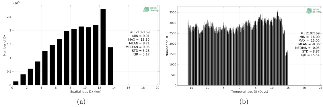
Figure 5: Histograms of the spatial (a) and temporal (b) lags between the location/time of the TSG (GOSUD-Research-vessel) measurement and the date of the corresponding SMAP SSS L4 OI v2 - Monthly (IPRC) SSS pixel.
