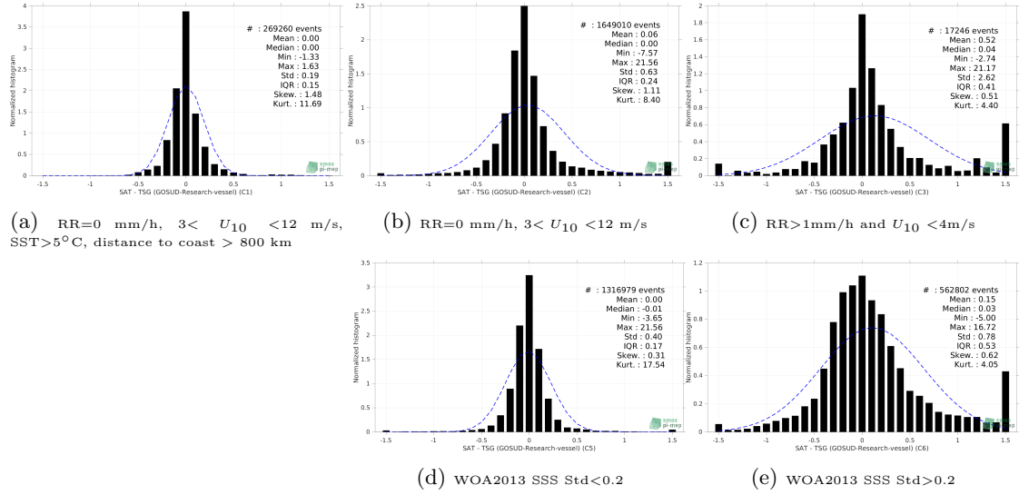
Figure 13: Normalized histogram of \Delta SSS (SMAP SSS L4 OI v2 - Monthly (IPRC) - TSG (GOSUD-Research-vessel)) for 5 different subdatasets corresponding to: RR=0 mm/h, 3 < U_{10} < 12 m/s, SST>5°C, distance to coast > 800 km (a), RR=0 mm/h, 3 < U_{10} < 12 m/s (b), RR>1mm/h and U_{10} < 4 m/s (c), WOA2013 SSS Std<0.2 (d), WOA2013 SSS Std>0.2 (e).
