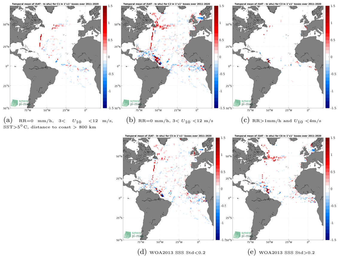
Figure 12: Temporal mean gridded over spatial boxes of size 1^\circ \times 1^\circ of \Delta\text{SSS} (SMAP SSS L4 OI v2 - Monthly (IPRC) - TSG (GOSUD-Research-vessel)) for 5 different subdatasets corresponding to:RR=0 mm/h, 3 < U_{10} < 12 m/s, SST>5°C, distance to coast > 800 km (a), RR=0 mm/h, 3 < U_{10} < 12 m/s (b), RR>1mm/h and U_{10} < 4 m/s (c), WOA2013 SSS Std<0.2 (d), WOA2013 SSS Std>0.2 (e).
