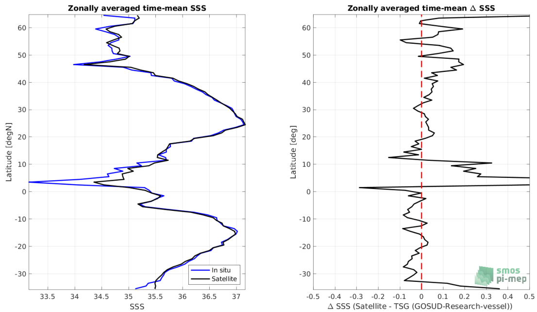
Figure 8: Left panel: Zonal mean SSS from SMAP SSS L4 OI v2 - Monthly (IPRC) satellite product (black) and from TSG (GOSUD-Research-vessel) (blue). Right panel: Zonal mean of \Delta SSS (Satellite - TSG (GOSUD-Research-vessel)) for all the collected Pi-MEP match-up pairs estimated over the full satellite product period.
