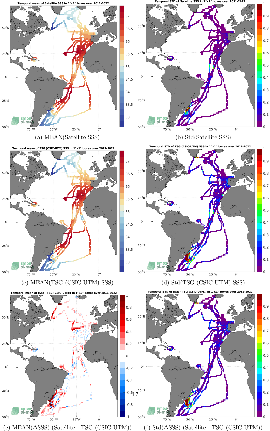
Figure 6: Temporal mean (left) and Std (right) of SSS from SMAP SSS L4 OI v2 - Monthly (IPRC) (top), TSG (CSIC-UTM) (middle), and of \Delta SSS (Satellite - TSG (CSIC-UTM)). Only match-up pairs are used to generate these maps.
