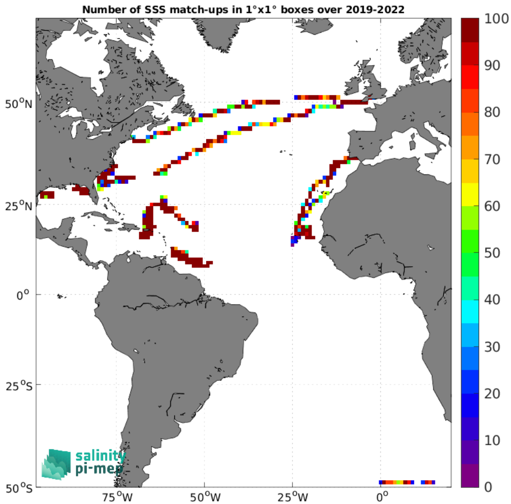
Figure 4: Number of SSS match-ups between Saildrone SSS and the SMAP SSS L4 OI v2 - Monthly (IPRC) SSS product for the Atlantic Ocean Pi-MEP region over 1^{\circ} \times 1^{\circ} boxes and for the full satellite product period.
