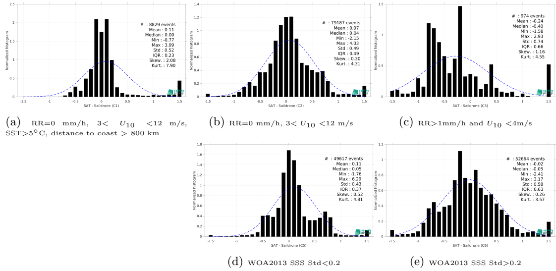
Figure 13: Normalized histogram of \Delta SSS (SMAP SSS L4 OI v2 - Monthly (IPRC) - Saildrone) for 5 different subdatasets corresponding to: RR=0 mm/h, 3 < U_{10} < 12 m/s, SST > 5°C, distance to coast > 800 km (a), RR=0 mm/h, 3 < U_{10} < 12 m/s (b), RR > 1mm/h and U_{10} < 4 m/s (c), WOA2013 SSS Std < 0.2 (d), WOA2013 SSS Std > 0.2 (e).
