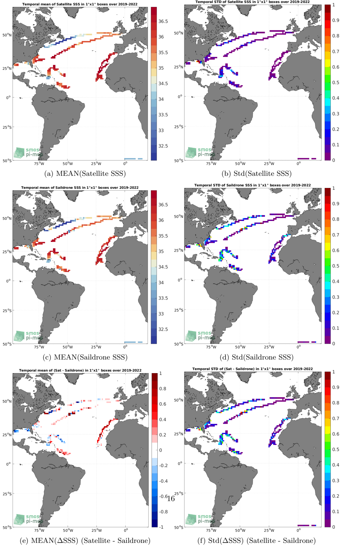
Figure 6: Temporal mean (left) and Std (right) of SSS from SMAP SSS L4 OI v2 - Monthly (IPRC) (top), Saildrone (middle), and of \Delta SSS (Satellite - Saildrone). Only match-up pairs are used to generate these maps.
