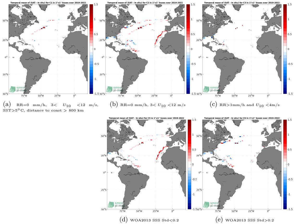
Figure 12: Temporal mean gridded over spatial boxes of size 1^\circ \times 1^\circ of \Delta SSS (SMAP SSS L4 OI v2 - Monthly (IPRC) - Saildrone) for 5 different subdatasets corresponding to:RR=0 mm/h, 3 < U_{10} < 12 m/s, SST >5^\circ\text{C} , distance to coast > 800 km (a), RR=0 mm/h, 3 < U_{10} < 12 m/s (b), RR >1 mm/h and U_{10} < 4 m/s (c), WOA2013 SSS Std <0.2 (d), WOA2013 SSS Std >0.2 (e).
