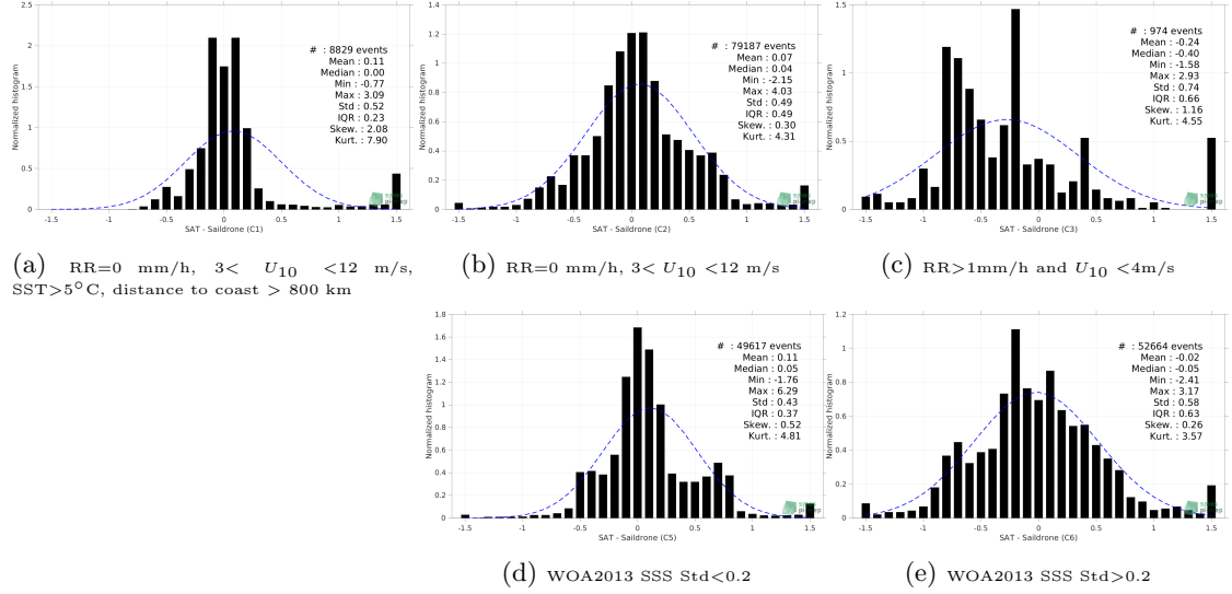
Figure 13: Normalized histogram of \Delta SSS (SMAP SSS L4 OI v2 - Monthly (IPRC) - Sairdron) for 5 different subdatasets corresponding to: RR=0 mm/h, 3 < U_{10} < 12 m/s, SST > 5°C, distance to coast > 800 km (a), RR=0 mm/h, 3 < U_{10} < 12 m/s (b), RR > 1mm/h and U_{10} < 4 m/s (c), WOA2013 SSS Std < 0.2 (d), WOA2013 SSS Std > 0.2 (e).
