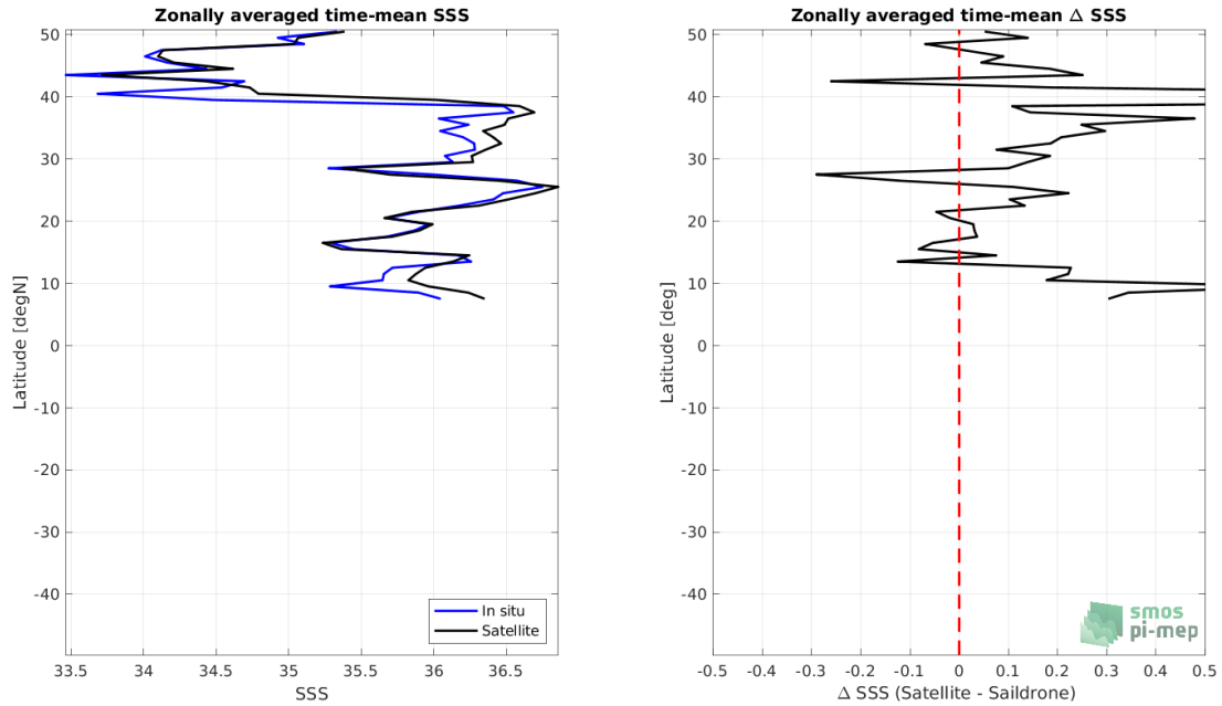
Figure 8: Left panel: Zonal mean SSS from SMAP SSS L4 OI v2 - Monthly (IPRC) satellite product (black) and from Sairdron (blue). Right panel: Zonal mean of \Delta SSS (Satellite - Sairdron) for all the collected Pi-MEP match-up pairs estimated over the full satellite product period.
