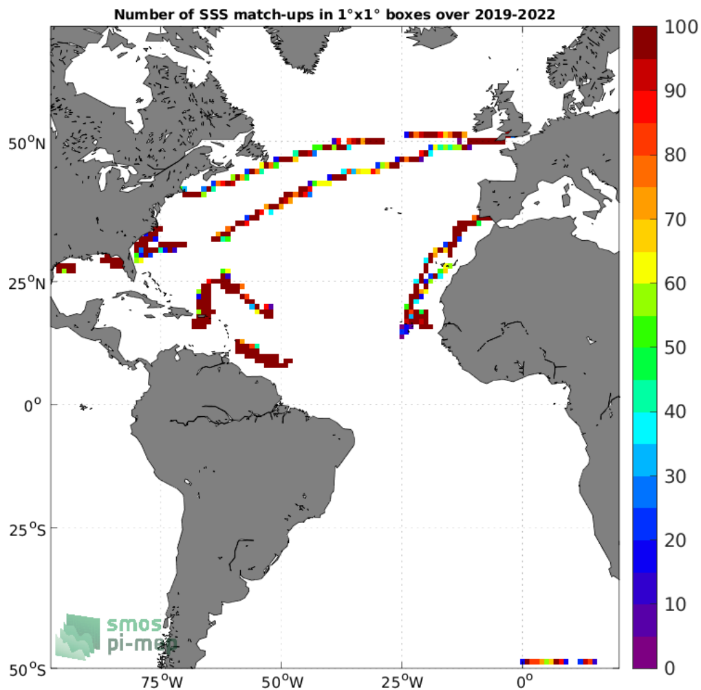
Figure 4: Number of SSS match-ups between Saildrone SSS and the SMAP SSS L4 OI v2 - Monthly (IPRC) SSS product for the Atlantic Ocean Pi-MEP region over 1°x1° boxes and for the full satellite product period.
