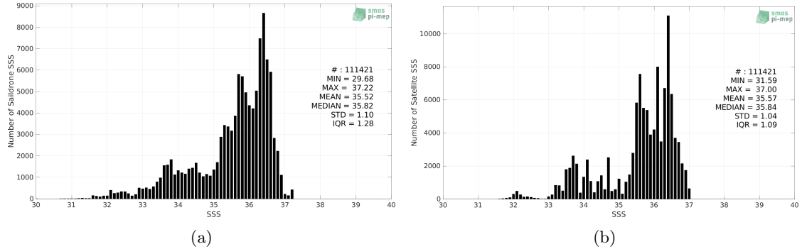
Figure 2: Histograms of SSS from Saildrone (a) and SMAP SSS L4 OI v2 - Monthly (IPRC) (b) considering all match-up pairs per bins of 0.1 over the Atlantic Ocean Pi-MEP region and for the full satellite product period.
