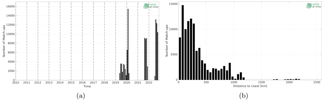
Figure 1: Number of match-ups between Saildrone and SMAP SSS L4 OI v2 - Monthly (IPRC) SSS as a function of time (a) and as function of the distance to coast (b) over the Atlantic Ocean Pi-MEP region and for the full satellite product period.
