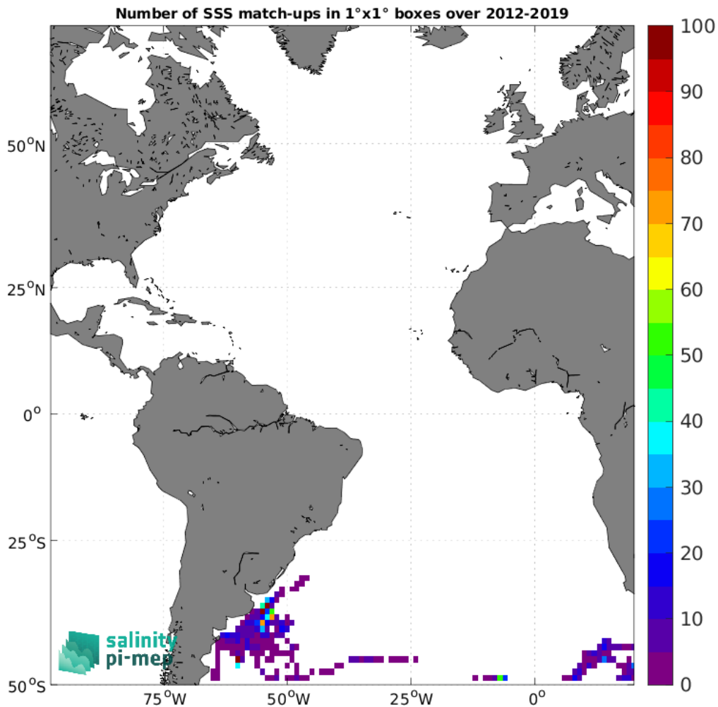
Figure 4: Number of SSS match-ups between Marine mammals SSS and the SMAP SSS L4 OI v2 - Monthly (IPRC) SSS product for the Atlantic Ocean Pi-MEP region over 1°×1° boxes and for the full satellite product period.
