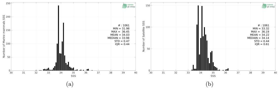
Figure 2: Histograms of SSS from Marine mammals (a) and SMAP SSS L4 OI v2 - Monthly (IPRC) (b) considering all match-up pairs per bins of 0.1 over the Atlantic Ocean Pi-MEP region and for the full satellite product period.
