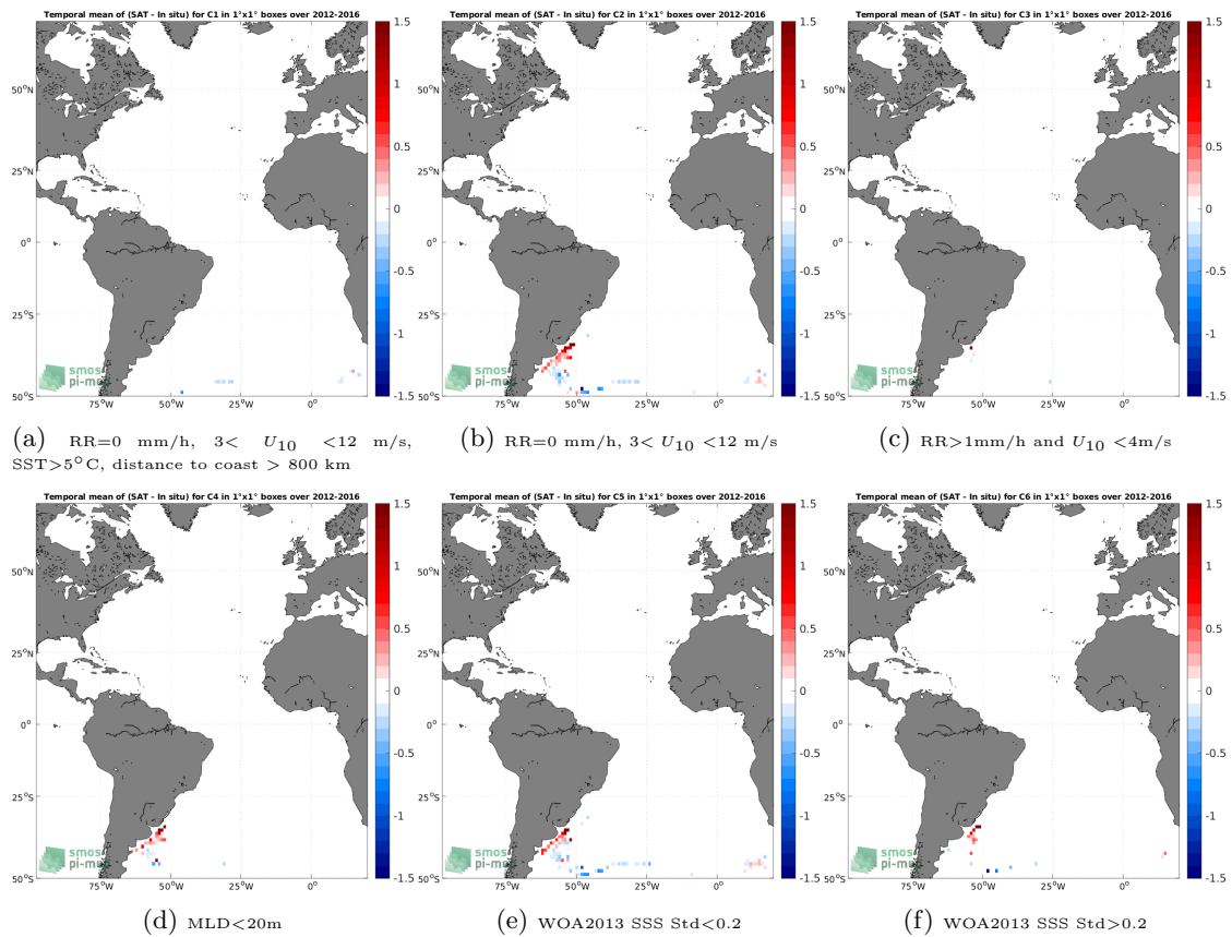
Figure 12: Temporal mean gridded over spatial boxes of size 1^\circ \times 1^\circ of \Delta SSS (SMAP SSS L4 OI v2 - Monthly (IPRC) - Marine mammals) for 6 different subdatasets corresponding to:RR=0 mm/h, 3 < U_{10} < 12 m/s, SST > 5^\circ\text{C} , distance to coast > 800 km (a), RR=0 mm/h, 3 < U_{10} < 12 m/s (b), RR > 1 mm/h and U_{10} < 4 m/s (c),MLD < 20 m (d),WOA2013 SSS Std < 0.2 (e),WOA2013 SSS Std > 0.2 (f).
