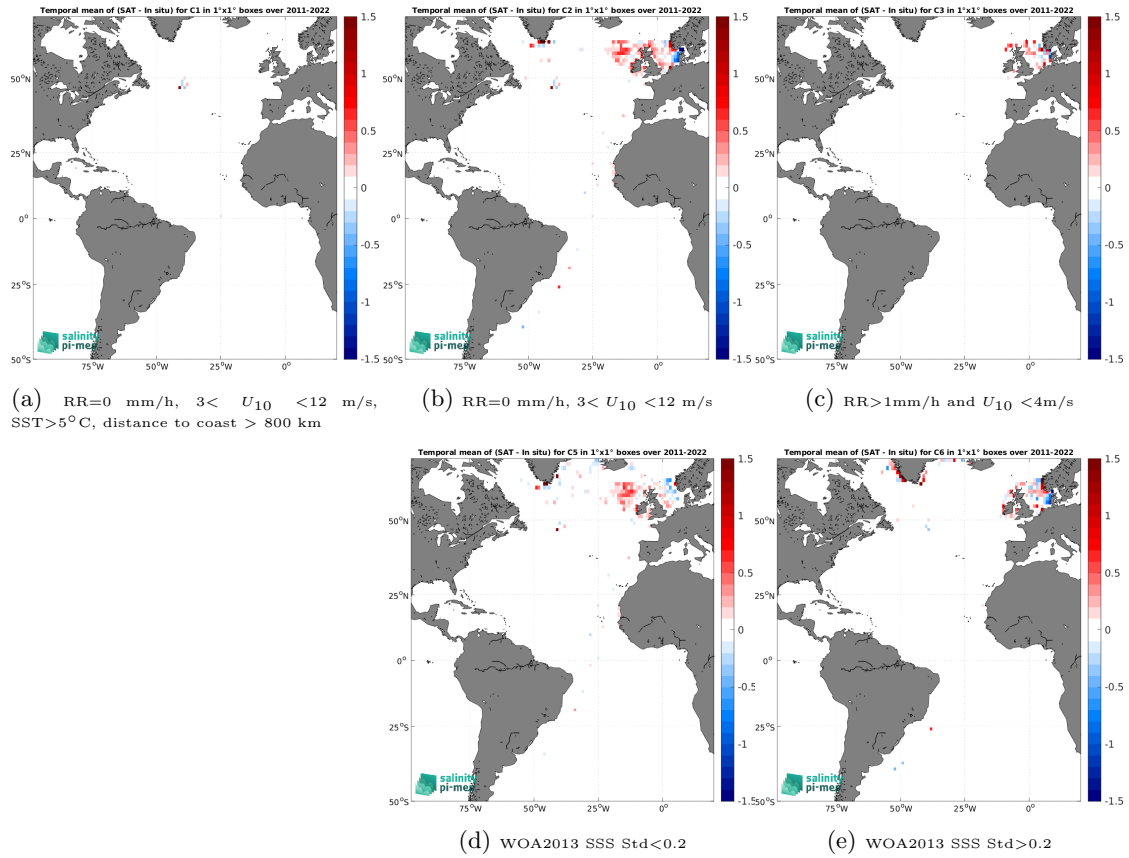
Figure 12: Temporal mean gridded over spatial boxes of size 1^\circ \times 1^\circ of \Delta SSS (SMAP SSS L4 OI v2 - Monthly (IPRC) - ICES) for 5 different subdatasets corresponding to:RR=0 mm/h, 3 < U_{10} < 12 m/s, SST >5^\circ\text{C} , distance to coast > 800 km (a), RR=0 mm/h, 3 < U_{10} < 12 m/s (b), RR >1 mm/h and U_{10} < 4 m/s (c), WOA2013 SSS Std <0.2 (d), WOA2013 SSS Std >0.2 (e).
