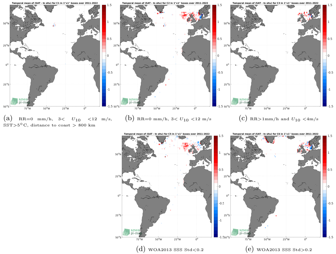
Figure 12: Temporal mean gridded over spatial boxes of size 1^\circ \times 1^\circ of \Delta SSS (SMAP SSS L4 OI v2 - Monthly (IPRC) - ICES) for 5 different subdatasets corresponding to:RR=0 mm/h, 3 < U_{10} < 12 m/s, SST >5^\circ\text{C} , distance to coast > 800 km (a), RR=0 mm/h, 3 < U_{10} < 12 m/s (b), RR >1 mm/h and U_{10} < 4 m/s (c), WOA2013 SSS Std <0.2 (d), WOA2013 SSS Std >0.2 (e).
