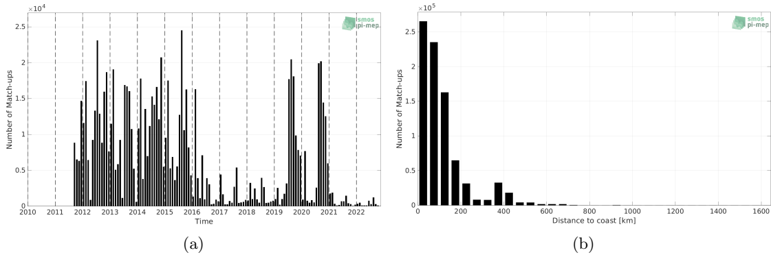
Figure 1: Number of match-ups between ICES and SMAP SSS L4 OI v2 - Monthly (IPRC) SSS as a function of time (a) and as function of the distance to coast (b) over the Atlantic Ocean Pi-MEP region and for the full satellite product period.
