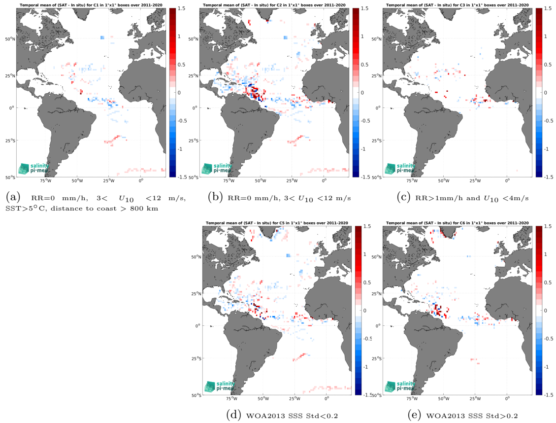
Figure 11: Temporal mean gridded over spatial boxes of size 1^\circ \times 1^\circ of \Delta SSS (SMAP SSS L4 OI v2 - Monthly (IPRC) - Surface drifters) for 5 different subdatasets corresponding to:RR=0 mm/h, 3 < U_{10} < 12 m/s, SST >5^\circ\text{C} , distance to coast > 800 km (a), RR=0 mm/h, 3 < U_{10} < 12 m/s (b), RR >1 mm/h and U_{10} < 4 m/s (c), WOA2013 SSS Std <0.2 (d), WOA2013 SSS Std >0.2 (e).
