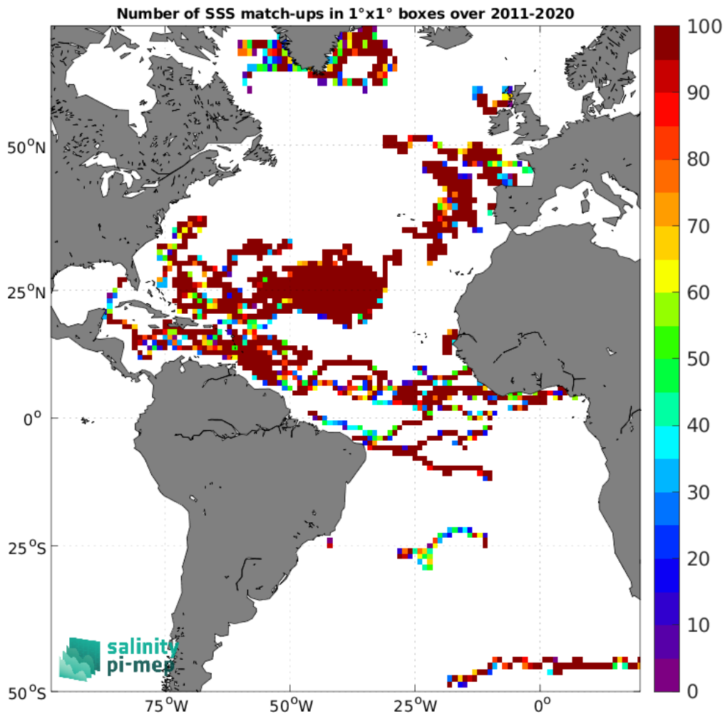
Figure 3: Number of SSS match-ups between Surface drifters SSS and the SMAP SSS L4 OI v2 - Monthly (IPRC) SSS product for the Atlantic Ocean Pi-MEP region over 1°x1° boxes and for the full satellite product period.
