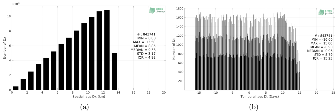
Figure 4: Histograms of the spatial (a) and temporal (b) lags between the location/time of the Surface drifters measurement and the date of the corresponding SMAP SSS L4 OI v2 - Monthly (IPRC) SSS pixel.
