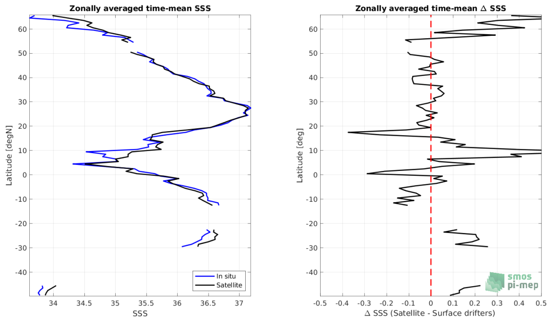
Figure 7: Left panel: Zonal mean SSS from SMAP SSS L4 OI v2 - Monthly (IPRC) satellite product (black) and from Surface drifters (blue). Right panel: Zonal mean of \Delta SSS (Satellite - Surface drifters) for all the collected Pi-MEP match-up pairs estimated over the full satellite product period.
