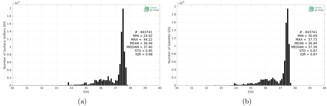
Figure 2: Histograms of SSS from Surface drifters (a) and SMAP SSS L4 OI v2 - Monthly (IPRC) (b) considering all match-up pairs per bins of 0.1 over the Atlantic Ocean Pi-MEP region and for the full satellite product period.
