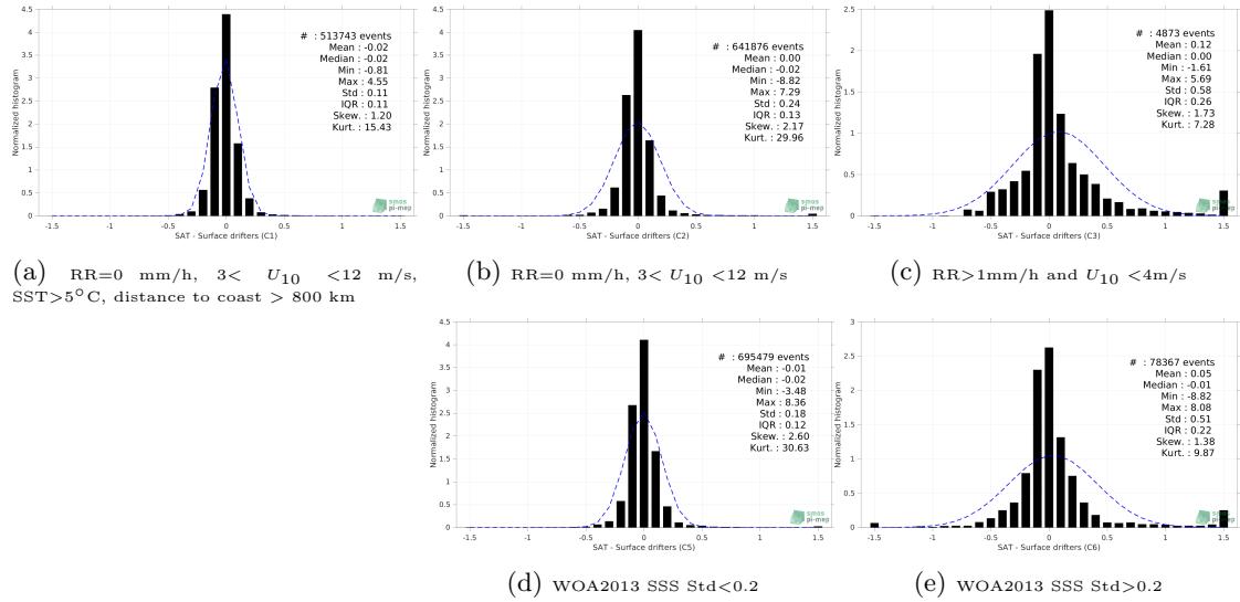
Figure 12: Normalized histogram of \Delta SSS (SMAP SSS L4 OI v2 - Monthly (IPRC) - Surface drifters) for 5 different subdatasets corresponding to: RR=0 mm/h, 3 < U_{10} < 12 m/s, SST>5°C, distance to coast > 800 km (a), RR=0 mm/h, 3 < U_{10} < 12 m/s (b), RR>1mm/h and U_{10} < 4 m/s (c), WOA2013 SSS Std<0.2 (d), WOA2013 SSS Std>0.2 (e).
