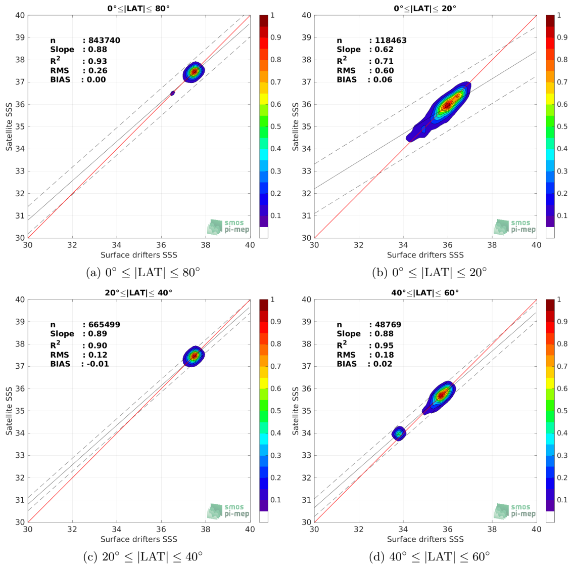
Figure 8: Contour maps of the concentration of SMAP SSS L4 OI v2 - Monthly (IPRC) SSS (y-axis) versus Surface drifters SSS (x-axis) at match-up pairs for different latitude bands. For each plot, the red line shows x=y . The black thin and dashed lines indicate a linear fit through the data cloud and the \pm 95\% confidence levels, respectively. The number match-up pairs n , the slope and R^2 coefficient of the linear fit, the root mean square (RMS) and the mean bias between satellite and in situ data are indicated for each latitude band in each plots.
