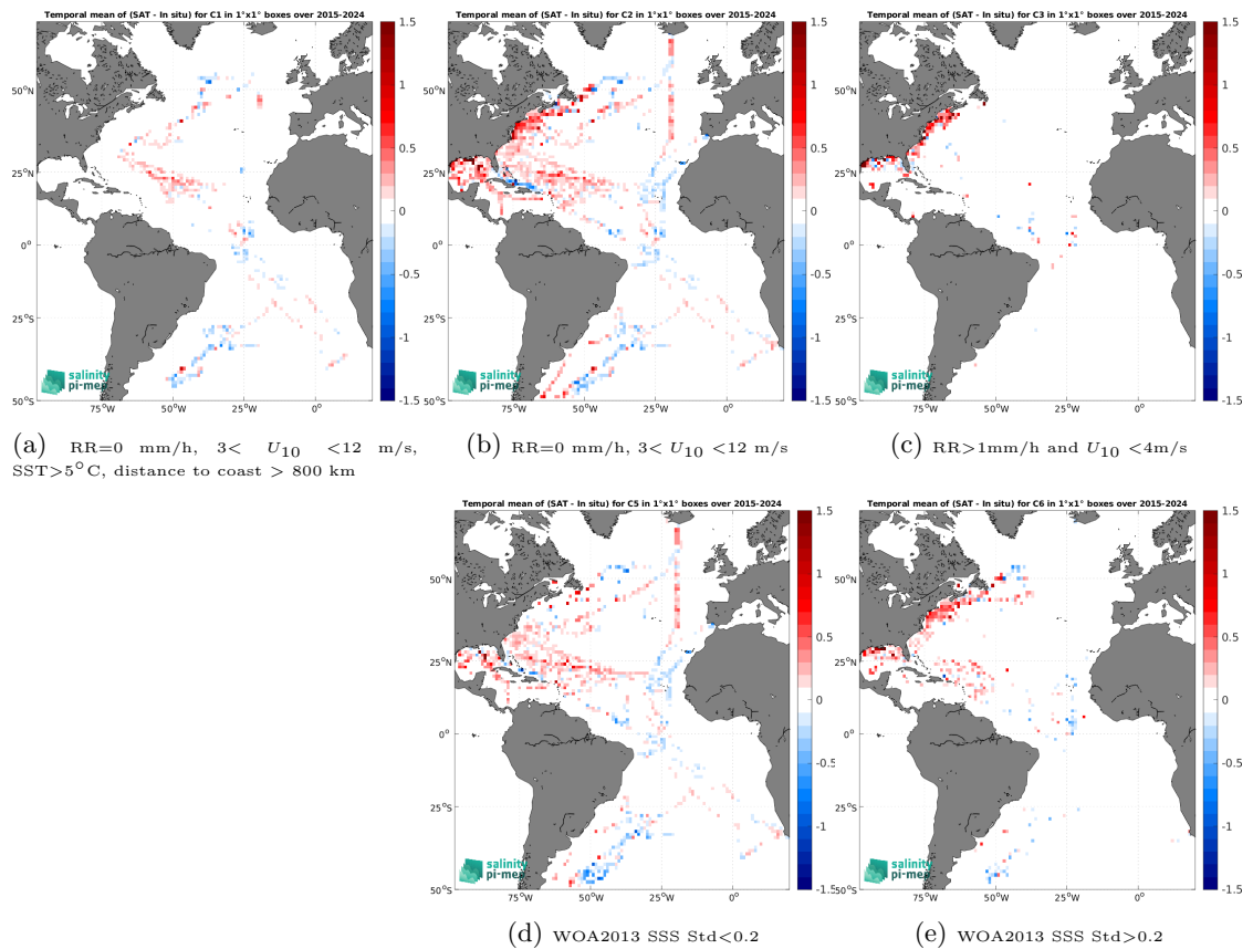
Figure 14: Temporal mean gridded over spatial boxes of size 1^\circ \times 1^\circ of \Delta SSS (SMAP SSS L3 v6 - 8-Day running (RSS) - TSG (SAMOS)) for 5 different subdatasets corresponding to:RR=0 mm/h, 3 < U_{10} < 12 m/s, SST>5°C, distance to coast > 800 km (a), RR=0 mm/h, 3 < U_{10} < 12 m/s (b), RR>1mm/h and U_{10} < 4 m/s (c), WOA2013 SSS Std<0.2 (d), WOA2013 SSS Std>0.2 (e).
