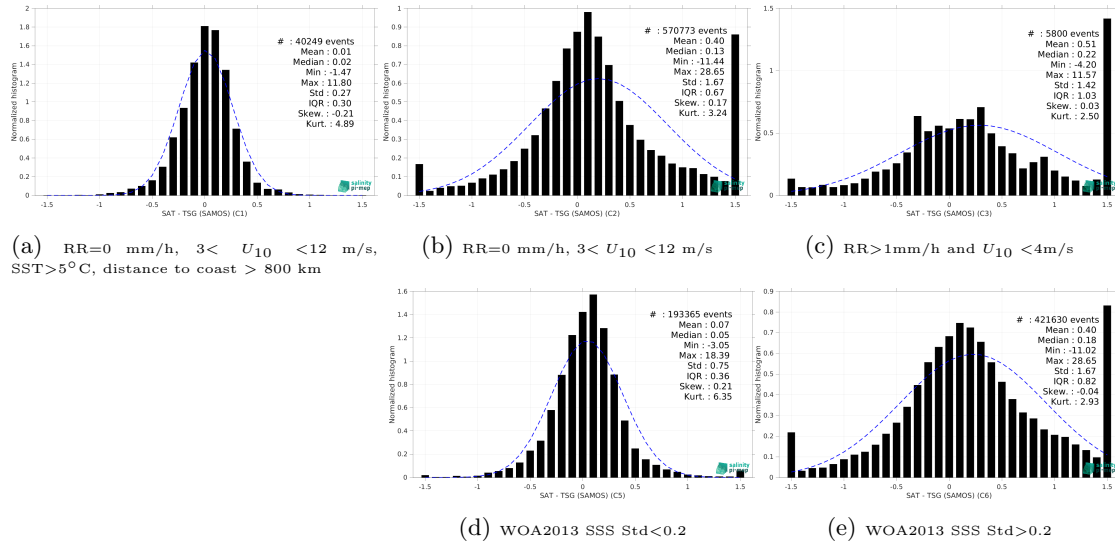
Figure 15: Normalized histogram of \Delta SSS (SMAP SSS L3 v6 - 8-Day running (RSS) - TSG (SAMOS)) for 5 different subdatasets corresponding to: RR=0 mm/h, 3 < U_{10} < 12 m/s, SST > 5°C, distance to coast > 800 km (a), RR=0 mm/h, 3 < U_{10} < 12 m/s (b), RR > 1mm/h and U_{10} < 4 m/s (c), WOA2013 SSS Std < 0.2 (d), WOA2013 SSS Std > 0.2 (e).
