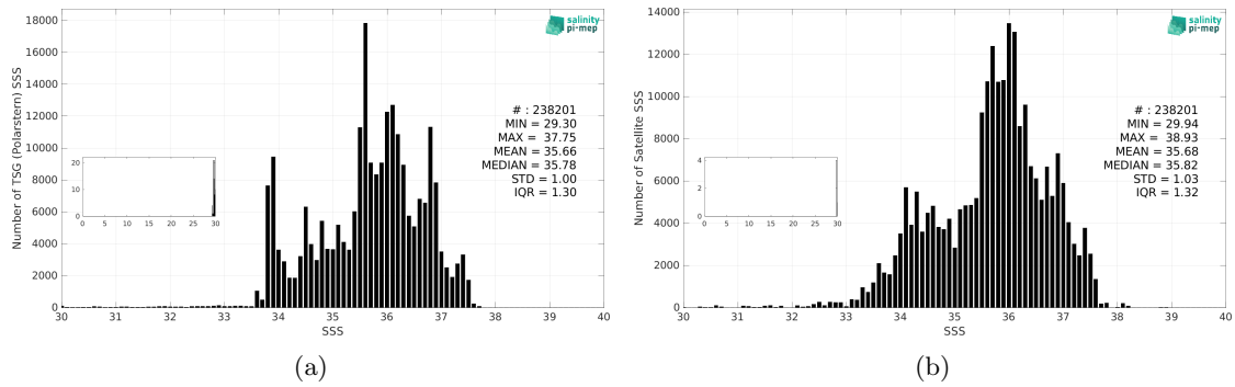
Figure 3: Histograms of SSS from TSG (Polarstern) (a) and SMAP SSS L3 v6 - 8-Day running (RSS) (b) considering all match-up pairs per bins of 0.1 over the Atlantic Ocean Pi-MEP region and for the full satellite product period.
