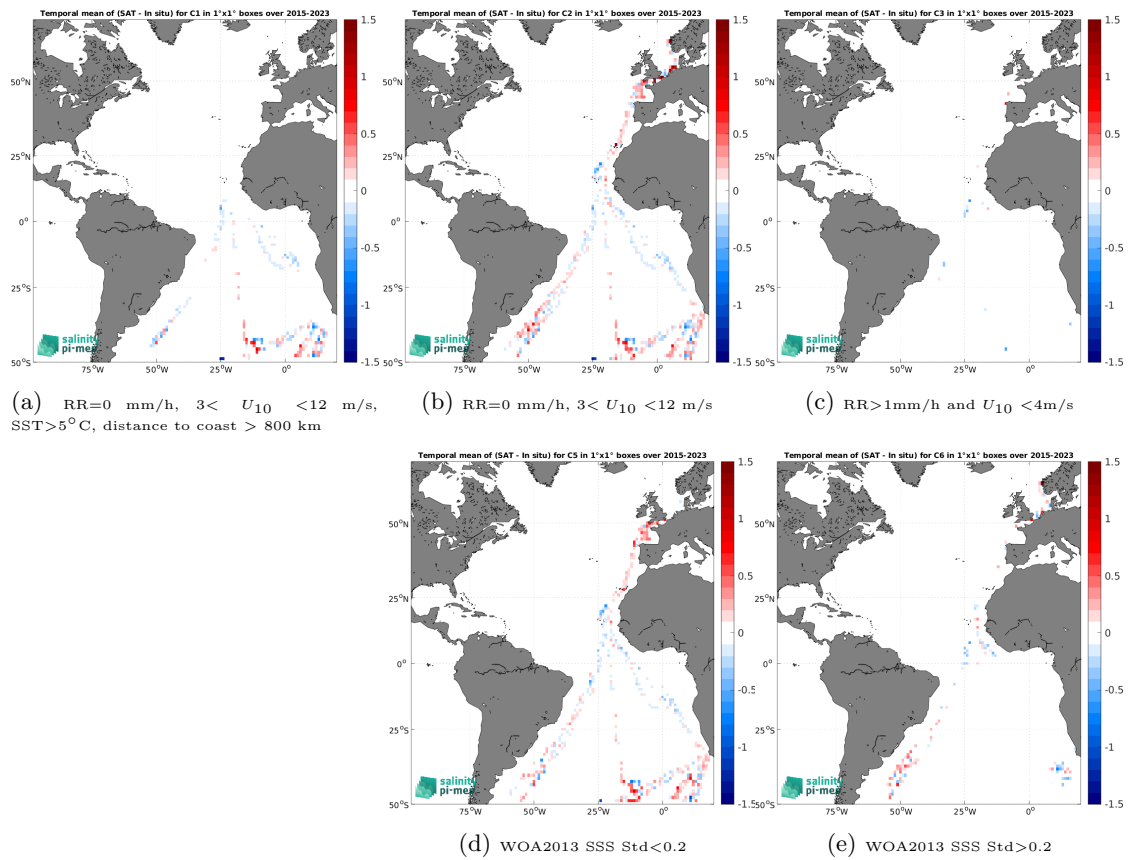
Figure 14: Temporal mean gridded over spatial boxes of size 1^\circ \times 1^\circ of \Delta\text{SSS} (SMAP SSS L3 v6 - 8-Day running (RSS) - TSG (Polarstern)) for 5 different subdatasets corresponding to:RR=0 mm/h, 3 < U_{10} < 12 m/s, SST >5^\circ\text{C} , distance to coast > 800 km (a), RR=0 mm/h, 3 < U_{10} < 12 m/s (b), RR >1 mm/h and U_{10} < 4 m/s (c), WOA2013 SSS Std <0.2 (d), WOA2013 SSS Std >0.2 (e).
