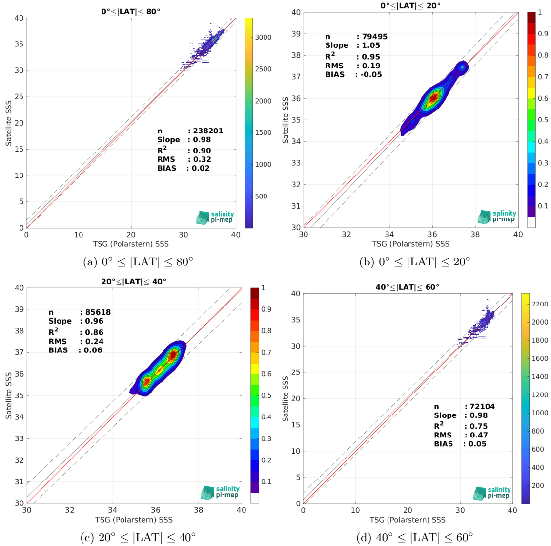
Figure 10: Contour maps of the concentration of SMAP SSS L3 v6 - 8-Day running (RSS) SSS (y-axis) versus TSG (Polarstern) SSS (x-axis) at match-up pairs for different latitude bands. For each plot, the red line shows x=y . The black thin and dashed lines indicate a linear fit through the data cloud and the \pm 95\% confidence levels, respectively. The number match-up pairs n , the slope and R^2 coefficient of the linear fit, the root mean square (RMS) and the mean bias between satellite and in situ data are indicated for each latitude band in each plots.
