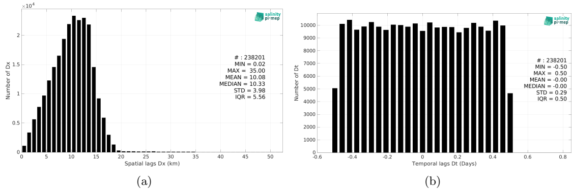
Figure 6: Histograms of the spatial (a) and temporal (b) lags between the location/time of the TSG (Polarstern) measurement and the date of the corresponding SMAP SSS L3 v6 - 8-Day running (RSS) SSS pixel.
