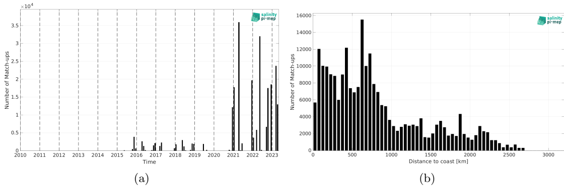
Figure 2: Number of match-ups between TSG (Polarstern) and SMAP SSS L3 v6 - 8-Day running (RSS) SSS as a function of time (a) and as function of the distance to coast (b) over the Atlantic Ocean Pi-MEP region and for the full satellite product period.
