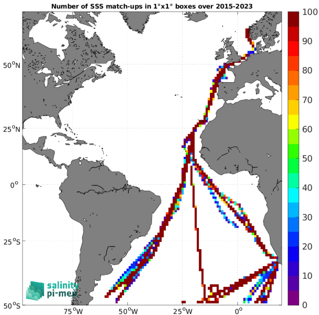
Figure 5: Number of SSS match-ups between TSG (Polarstern) SSS and the SMAP SSS L3 v6 - 8-Day running (RSS) SSS product for the Atlantic Ocean Pi-MEP region over 1^\circ \times 1^\circ boxes and for the full satellite product period.
