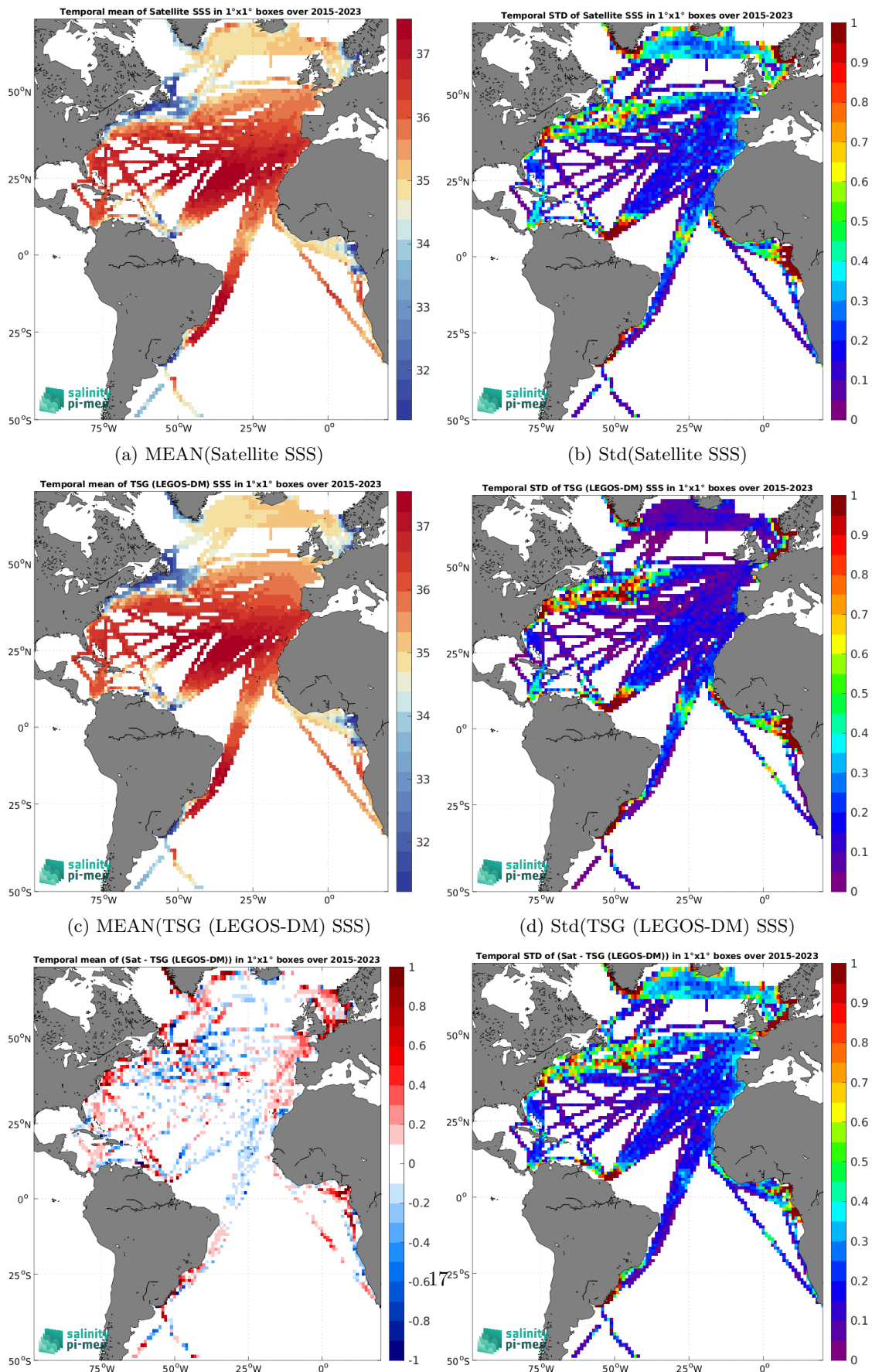
(e) MEAN( \Delta SSS) (Satellite - TSG (LEGOS-DM)) (f) Std( \Delta SSS) (Satellite - TSG (LEGOS-DM)) Figure 7: Temporal mean (left) and Std (right) of SSS from SMAP SSS L3 v6 - 8-Day running (RSS) (top), TSG (LEGOS-DM) (middle), and of \Delta SSS (Satellite - TSG (LEGOS-DM)). Only match-up pairs are used to generate these maps.
