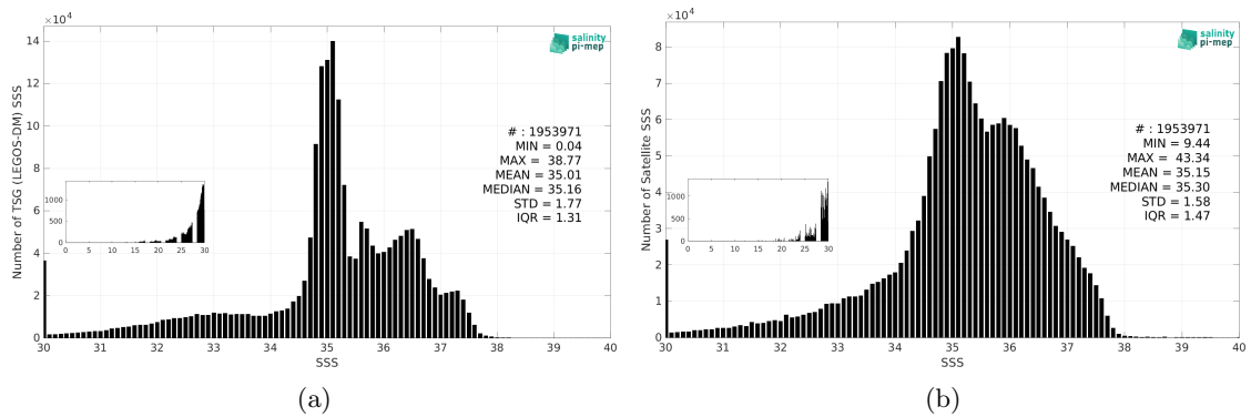
Figure 3: Histograms of SSS from TSG (LEGOS-DM) (a) and SMAP SSS L3 v6 - 8-Day running (RSS) (b) considering all match-up pairs per bins of 0.1 over the Atlantic Ocean Pi-MEP region and for the full satellite product period.
