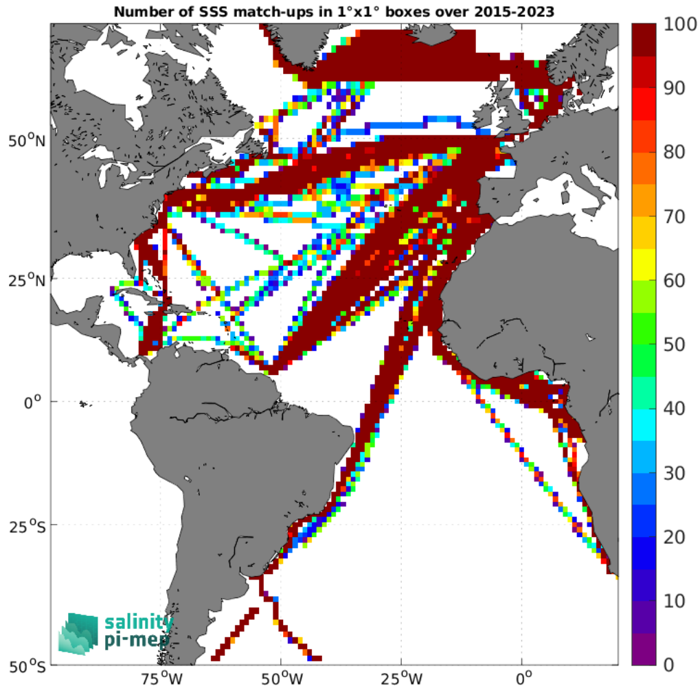
Figure 5: Number of SSS match-ups between TSG (LEGOS-DM) SSS and the SMAP SSS L3 v6 - 8-Day running (RSS) SSS product for the Atlantic Ocean Pi-MEP region over 1^\circ \times 1^\circ boxes and for the full satellite product period.
