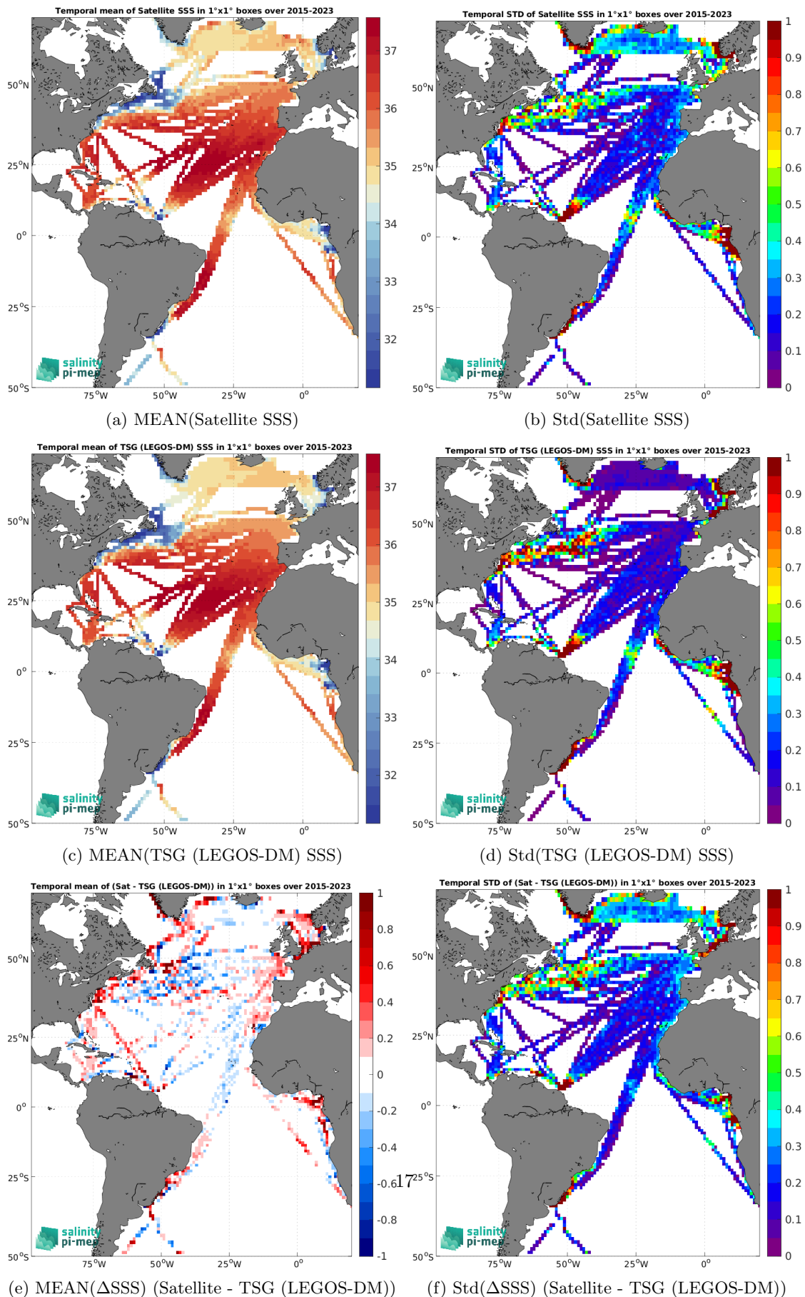
Figure 7: Temporal mean (left) and Std (right) of SSS from SMAP SSS L3 v6 - 8-Day running (RSS) (top), TSG (LEGOS-DM) (middle), and of \Delta SSS (Satellite - TSG (LEGOS-DM)). Only match-up pairs are used to generate these maps.
