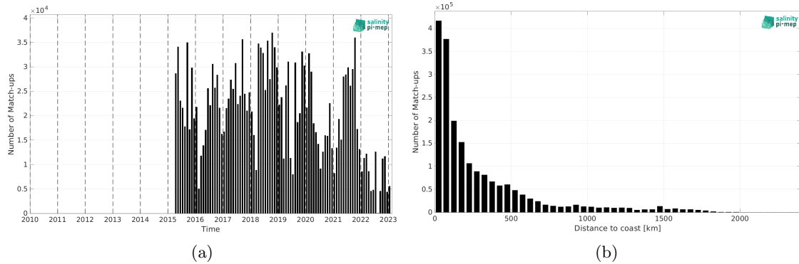
Figure 2: Number of match-ups between TSG (LEGOS-DM) and SMAP SSS L3 v6 - 8-Day running (RSS) SSS as a function of time (a) and as function of the distance to coast (b) over the Atlantic Ocean Pi-MEP region and for the full satellite product period.
