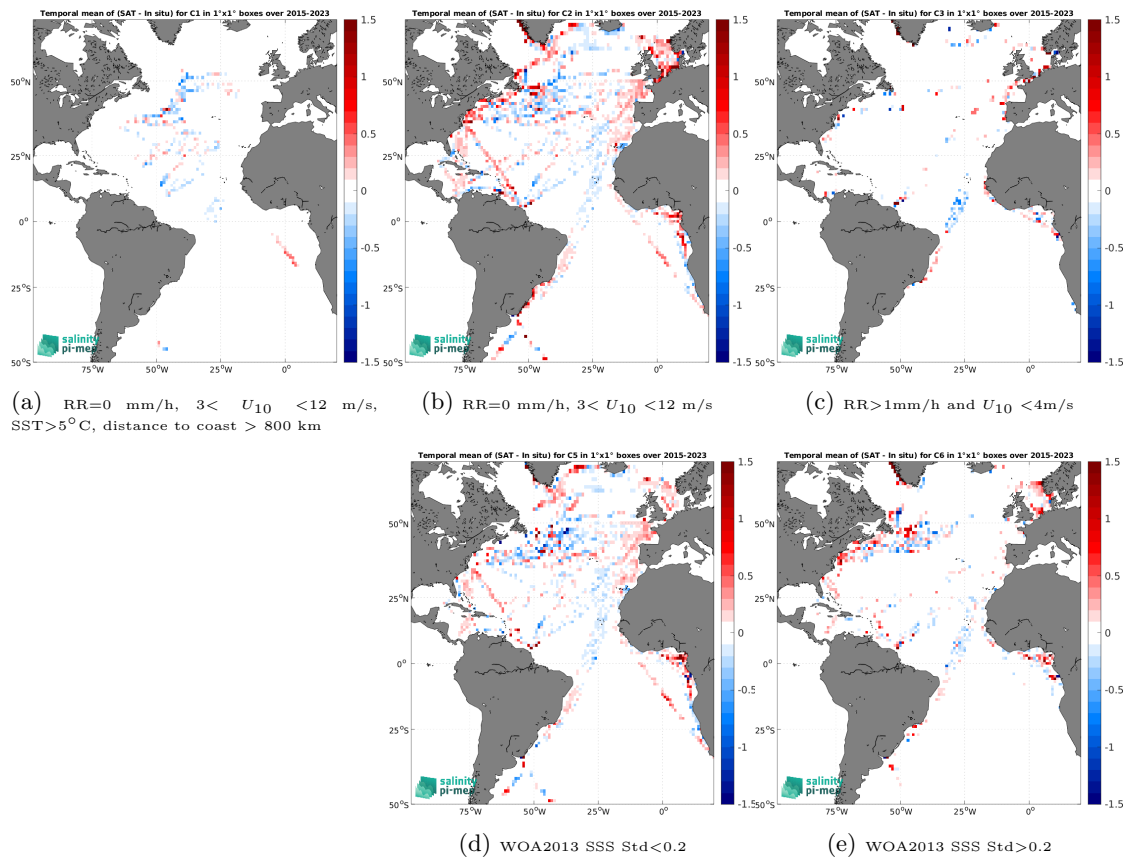
Figure 14: Temporal mean gridded over spatial boxes of size 1^\circ \times 1^\circ of \Delta\text{SSS} (SMAP SSS L3 v6 - 8-Day running (RSS) - TSG (LEGOS-DM)) for 5 different subdatasets corresponding to:RR=0 mm/h, 3 < U_{10} < 12 m/s, SST>5°C, distance to coast > 800 km (a), RR=0 mm/h, 3 < U_{10} < 12 m/s (b), RR>1mm/h and U_{10} < 4 m/s (c), WOA2013 SSS Std<0.2 (d), WOA2013 SSS Std>0.2 (e).
