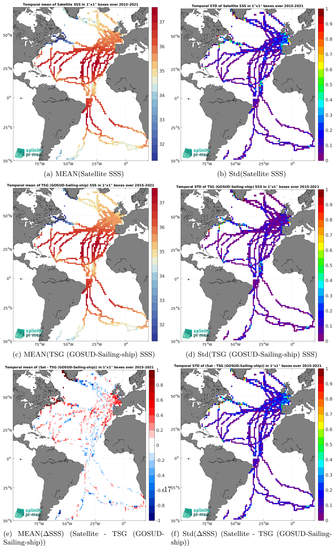
Figure 7: Temporal mean (left) and Std (right) of SSS from SMAP SSS L3 v6 - 8-Day running (RSS) (top), TSG (GOSUD-Sailing-ship) (middle), and of \Delta SSS (Satellite - TSG (GOSUD-Sailing-ship)). Only match-up pairs are used to generate these maps.
