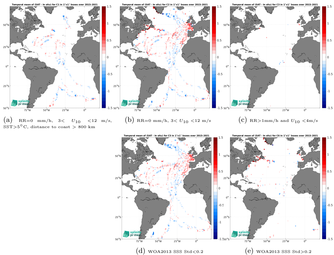
Figure 14: Temporal mean gridded over spatial boxes of size 1^\circ \times 1^\circ of \Delta SSS (SMAP SSS L3 v6 - 8-Day running (RSS) - TSG (GOSUD-Sailing-ship)) for 5 different subdatasets corresponding to:RR=0 mm/h, 3 < U_{10} < 12 m/s, SST >5^\circ\text{C} , distance to coast > 800 km (a), RR=0 mm/h, 3 < U_{10} < 12 m/s (b), RR >1 mm/h and U_{10} < 4 m/s (c), WOA2013 SSS Std <0.2 (d), WOA2013 SSS Std >0.2 (e).
