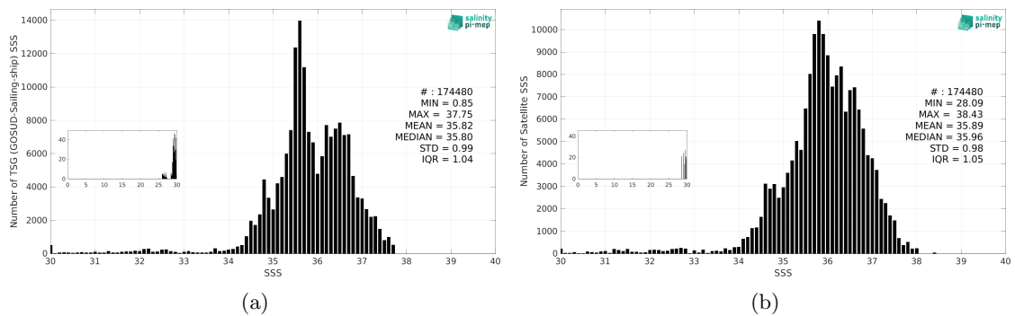
Figure 3: Histograms of SSS from TSG (GOSUD-Sailing-ship) (a) and SMAP SSS L3 v6 - 8-Day running (RSS) (b) considering all match-up pairs per bins of 0.1 over the Atlantic Ocean Pi-MEP region and for the full satellite product period.
