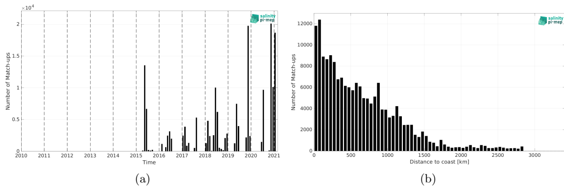
Figure 2: Number of match-ups between TSG (GOSUD-Sailing-ship) and SMAP SSS L3 v6 - 8-Day running (RSS) SSS as a function of time (a) and as function of the distance to coast (b) over the Atlantic Ocean Pi-MEP region and for the full satellite product period.
