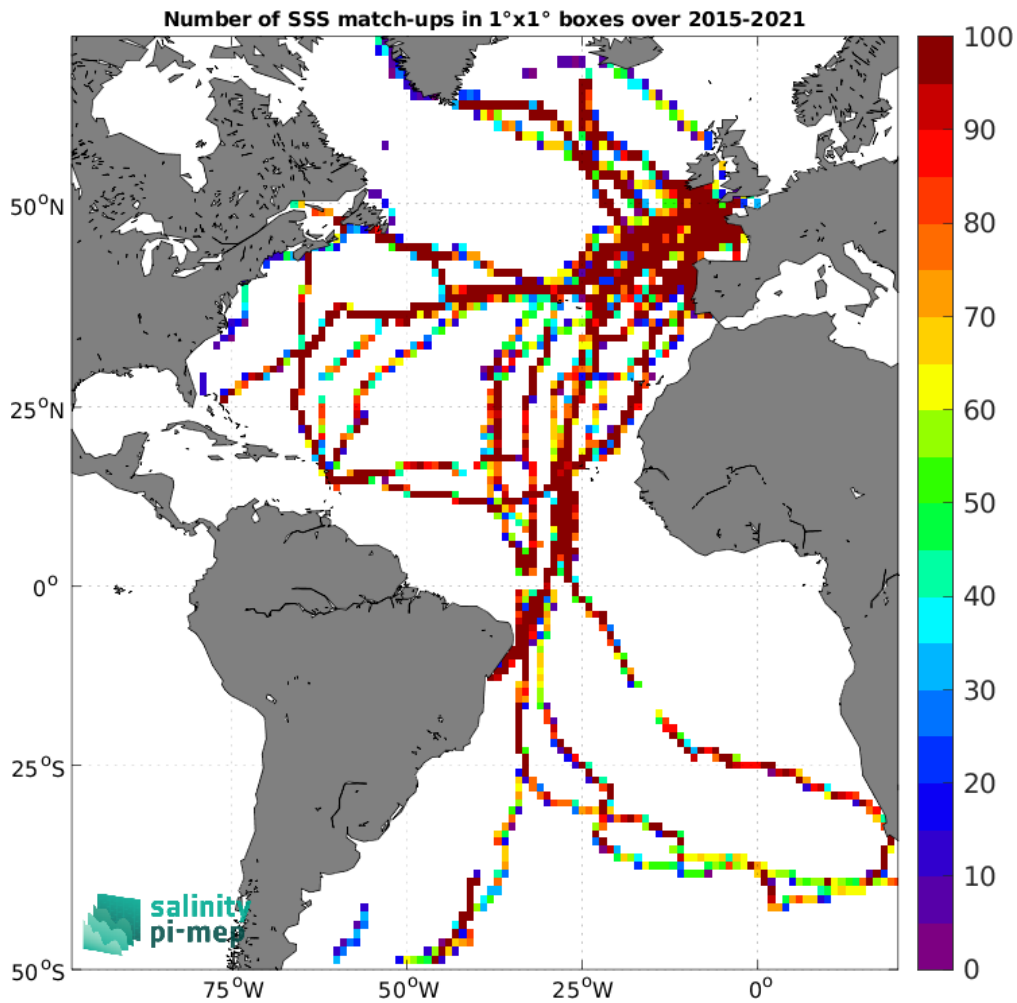
Figure 5: Number of SSS match-ups between TSG (GOSUD-Sailing-ship) SSS and the SMAP SSS L3 v6 - 8-Day running (RSS) SSS product for the Atlantic Ocean Pi-MEP region over 1^\circ \times 1^\circ boxes and for the full satellite product period.
