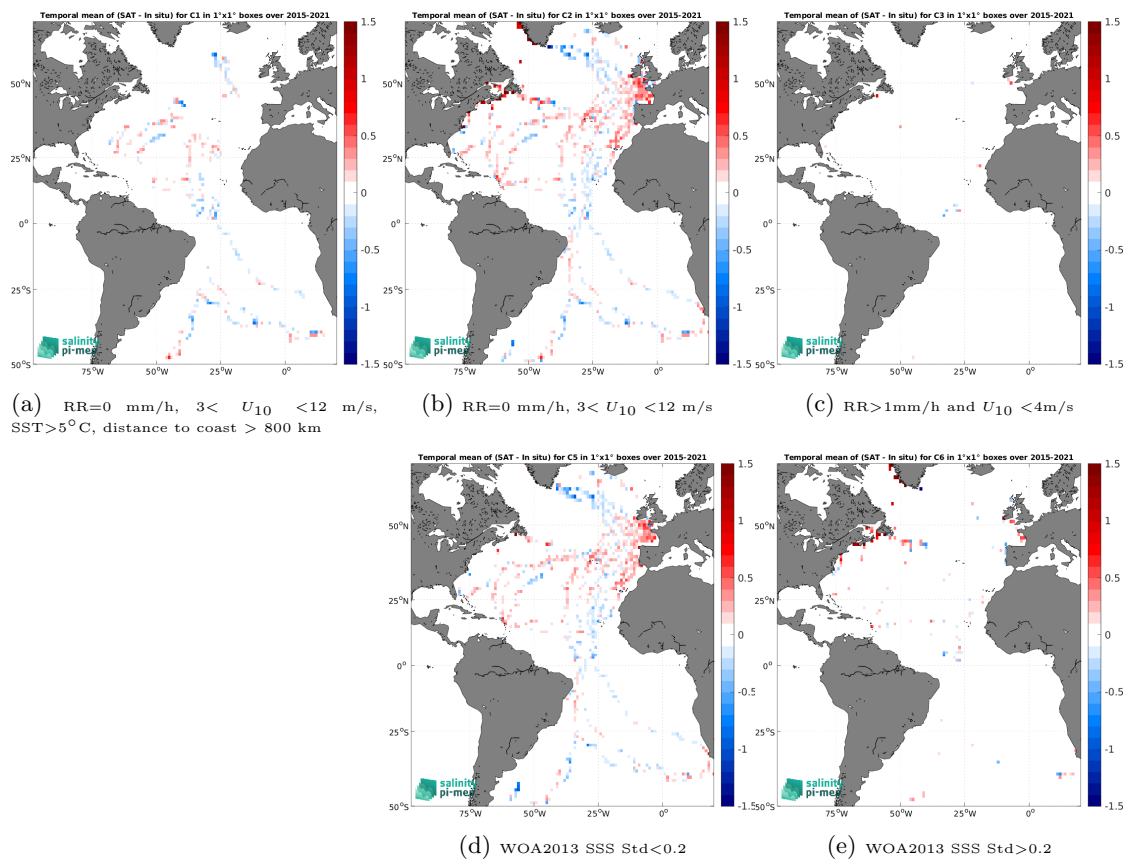
Figure 14: Temporal mean gridded over spatial boxes of size 1^\circ \times 1^\circ of \Delta\text{SSS} (SMAP SSS L3 v6 - 8-Day running (RSS) - TSG (GOSUD-Sailing-ship)) for 5 different subdatasets corresponding to:RR=0 mm/h, 3 < U_{10} < 12 m/s, SST >5^\circ\text{C} , distance to coast > 800 km (a), RR=0 mm/h, 3 < U_{10} < 12 m/s (b), RR >1 mm/h and U_{10} < 4 m/s (c), WOA2013 SSS Std <0.2 (d), WOA2013 SSS Std >0.2 (e).
