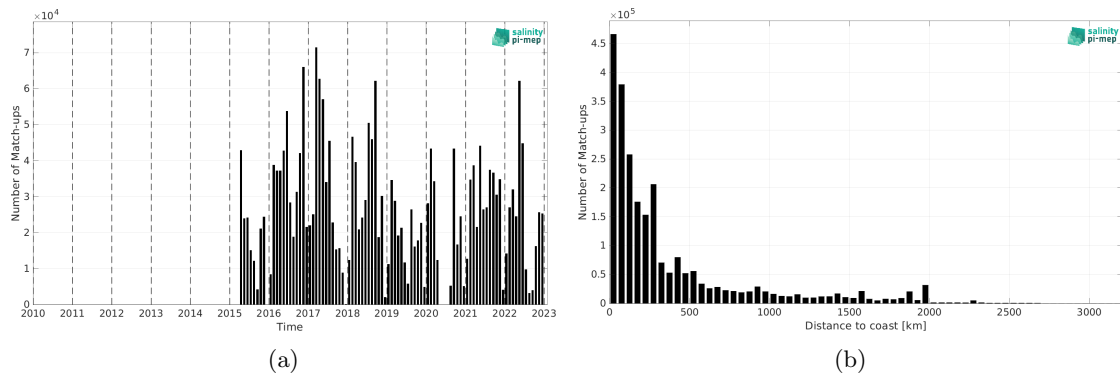
Figure 2: Number of match-ups between TSG (GOSUD-Research-vessel) and SMAP SSS L3 v6 - 8-Day running (RSS) SSS as a function of time (a) and as function of the distance to coast (b) over the Atlantic Ocean Pi-MEP region and for the full satellite product period.
