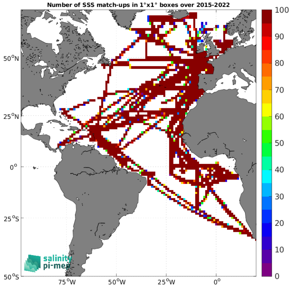
Figure 5: Number of SSS match-ups between TSG (GOSUD-Research-vessel) SSS and the SMAP SSS L3 v6 - 8-Day running (RSS) SSS product for the Atlantic Ocean Pi-MEP region over 1^\circ \times 1^\circ boxes and for the full satellite product period.
