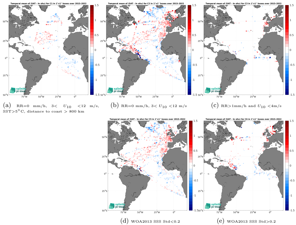
Figure 14: Temporal mean gridded over spatial boxes of size 1^\circ \times 1^\circ of \Delta\text{SSS} (SMAP SSS L3 v6 - 8-Day running (RSS) - TSG (GOSUD-Research-vessel)) for 5 different subdatasets corresponding to:RR=0 mm/h, 3 < U_{10} < 12 m/s, SST >5^\circ\text{C} , distance to coast > 800 km (a), RR=0 mm/h, 3 < U_{10} < 12 m/s (b), RR >1 mm/h and U_{10} < 4 m/s (c), WOA2013 SSS Std <0.2 (d), WOA2013 SSS Std >0.2 (e).
