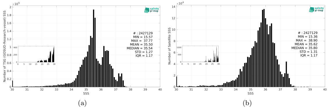
Figure 3: Histograms of SSS from TSG (GOSUD-Research-vessel) (a) and SMAP SSS L3 v6 - 8-Day running (RSS) (b) considering all match-up pairs per bins of 0.1 over the Atlantic Ocean Pi-MEP region and for the full satellite product period.
