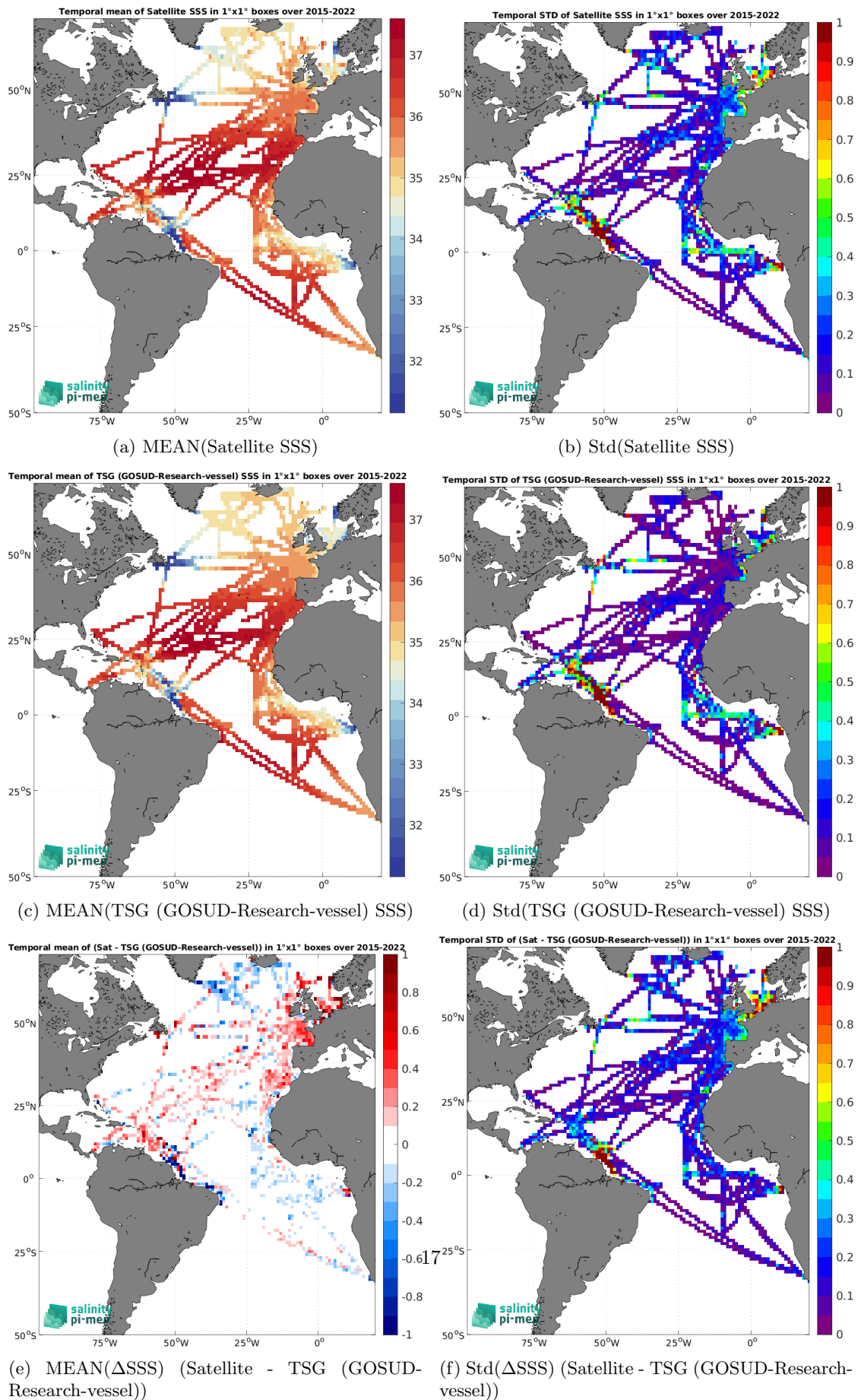
Figure 7: Temporal mean (left) and Std (right) of SSS from SMAP SSS L3 v6 - 8-Day running (RSS) (top), TSG (GOSUD-Research-vessel) (middle), and of \Delta SSS (Satellite - TSG (GOSUD-Research-vessel)). Only match-up pairs are used to generate these maps.
