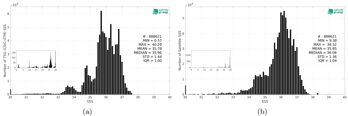
Figure 3: Histograms of SSS from TSG (CSIC-UTM) (a) and SMAP SSS L3 v6 - 8-Day running (RSS) (b) considering all match-up pairs per bins of 0.1 over the Atlantic Ocean Pi-MEP region and for the full satellite product period.
