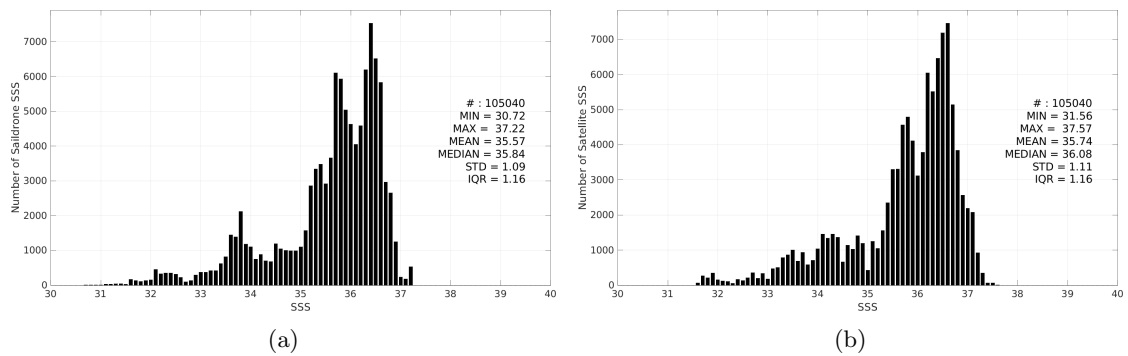
Figure 3: Histograms of SSS from Saildrone (a) and SMAP SSS L3 v6 - 8-Day running (RSS) (b) considering all match-up pairs per bins of 0.1 over the Atlantic Ocean Pi-MEP region and for the full satellite product period.
