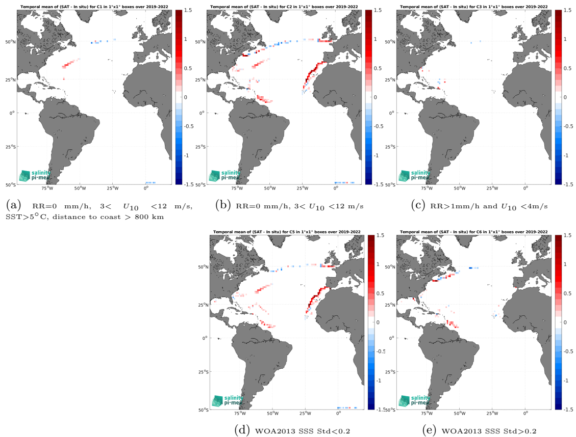
Figure 14: Temporal mean gridded over spatial boxes of size 1^\circ \times 1^\circ of \Delta SSS (SMAP SSS L3 v6 - 8-Day running (RSS) - Saildrone) for 5 different subdatasets corresponding to:RR=0 mm/h, 3 < U_{10} < 12 m/s, SST >5^\circ\text{C} , distance to coast > 800 km (a), RR=0 mm/h, 3 < U_{10} < 12 m/s (b), RR >1 mm/h and U_{10} < 4 m/s (c), WOA2013 SSS Std <0.2 (d), WOA2013 SSS Std >0.2 (e).
