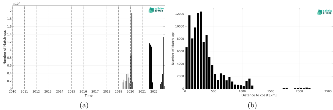
Figure 2: Number of match-ups between Saildrone and SMAP SSS L3 v6 - 8-Day running (RSS) SSS as a function of time (a) and as function of the distance to coast (b) over the Atlantic Ocean Pi-MEP region and for the full satellite product period.
