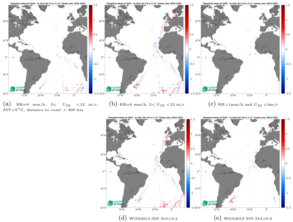
Figure 14: Temporal mean gridded over spatial boxes of size 1^\circ \times 1^\circ of \Delta\text{SSS} (SMAP SSS L3 v6 - Monthly (RSS) - TSG (Polarstern)) for 5 different subdatasets corresponding to:RR=0 mm/h, 3 < U_{10} < 12 m/s, SST>5°C, distance to coast > 800 km (a), RR=0 mm/h, 3 < U_{10} < 12 m/s (b), RR>1mm/h and U_{10} < 4 m/s (c), WOA2013 SSS Std<0.2 (d), WOA2013 SSS Std>0.2 (e).
