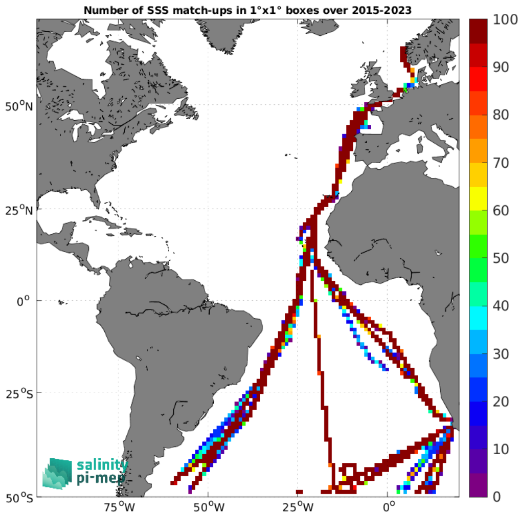
Figure 5: Number of SSS match-ups between TSG (Polarstern) SSS and the SMAP SSS L3 v6 - Monthly (RSS) SSS product for the Atlantic Ocean Pi-MEP region over 1°×1° boxes and for the full satellite product period.
