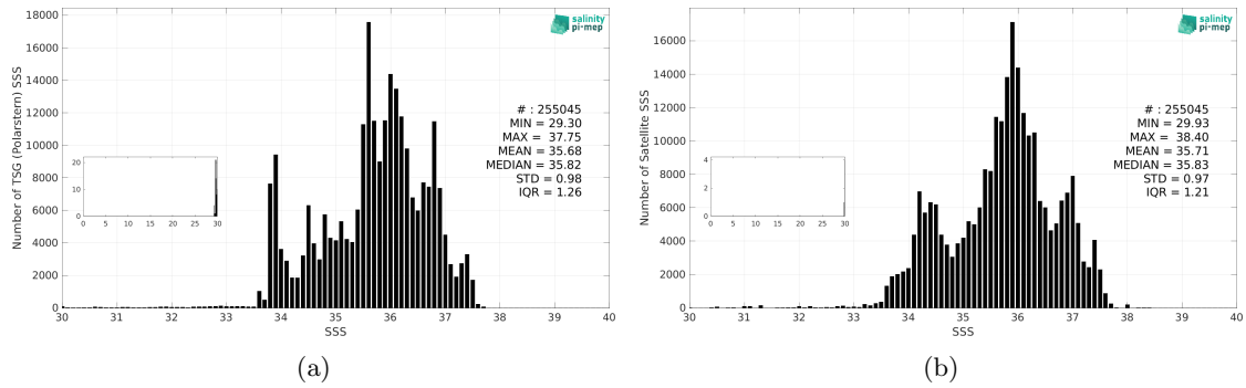
Figure 3: Histograms of SSS from TSG (Polarstern) (a) and SMAP SSS L3 v6 - Monthly (RSS) (b) considering all match-up pairs per bins of 0.1 over the Atlantic Ocean Pi-MEP region and for the full satellite product period.
