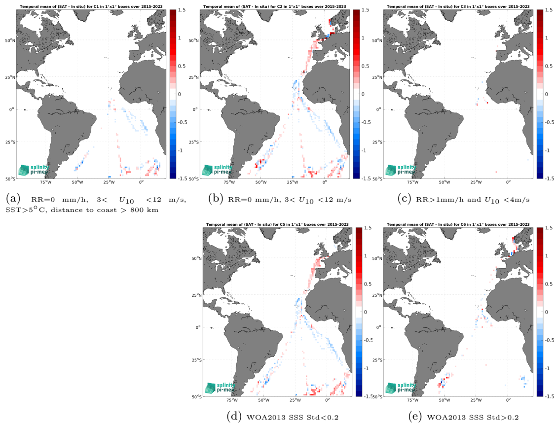
Figure 14: Temporal mean gridded over spatial boxes of size 1^\circ \times 1^\circ of \Delta\text{SSS} (SMAP SSS L3 v6 - Monthly (RSS) - TSG (Polarstern)) for 5 different subdatasets corresponding to:RR=0 mm/h, 3 < U_{10} < 12 m/s, SST>5°C, distance to coast > 800 km (a), RR=0 mm/h, 3 < U_{10} < 12 m/s (b), RR>1mm/h and U_{10} < 4 m/s (c), WOA2013 SSS Std<0.2 (d), WOA2013 SSS Std>0.2 (e).
