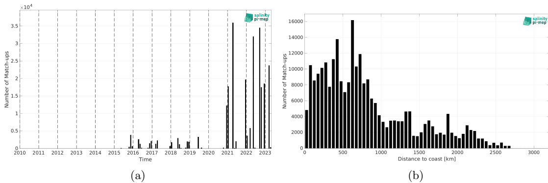
Figure 2: Number of match-ups between TSG (Polarstern) and SMAP SSS L3 v6 - Monthly (RSS) SSS as a function of time (a) and as function of the distance to coast (b) over the Atlantic Ocean Pi-MEP region and for the full satellite product period.
