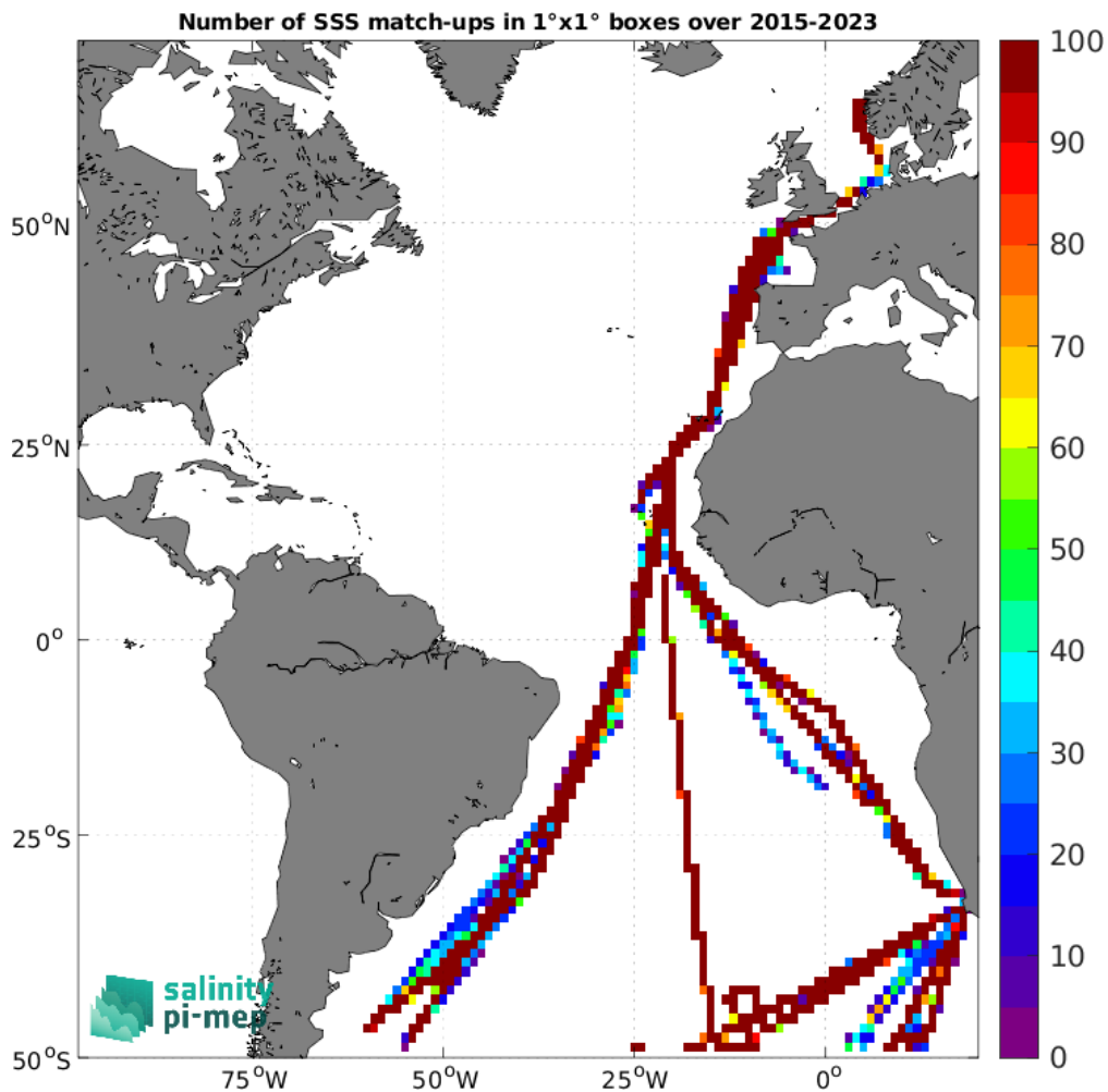
Figure 5: Number of SSS match-ups between TSG (Polarstern) SSS and the SMAP SSS L3 v6 - Monthly (RSS) SSS product for the Atlantic Ocean Pi-MEP region over 1^\circ \times 1^\circ boxes and for the full satellite product period.
