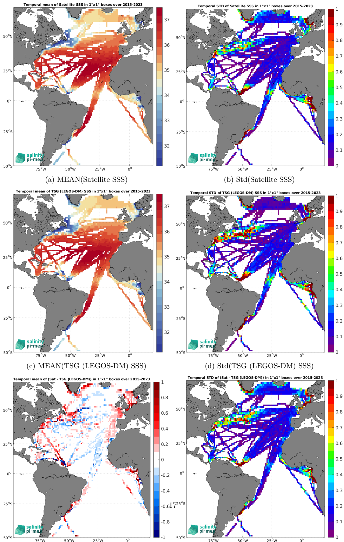
(e) MEAN( \Delta SSS) (Satellite - TSG (LEGOS-DM)) (f) Std( \Delta SSS) (Satellite - TSG (LEGOS-DM)) Figure 7: Temporal mean (left) and Std (right) of SSS from SMAP SSS L3 v6 - Monthly (RSS) (top), TSG (LEGOS-DM) (middle), and of \Delta SSS (Satellite - TSG (LEGOS-DM)). Only match-pairs are used to generate these maps.
