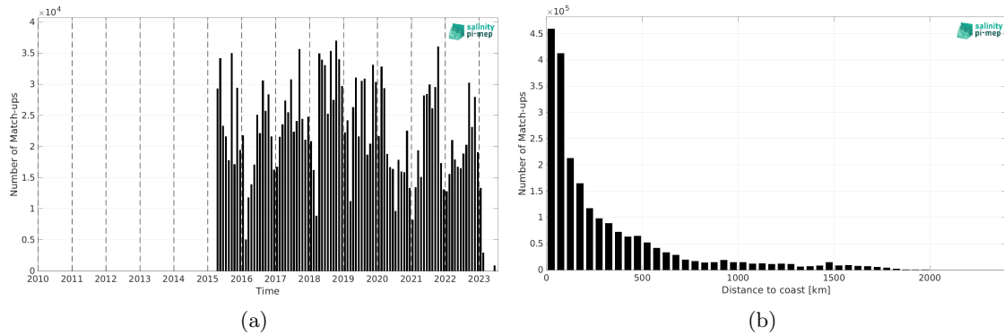
Figure 2: Number of match-ups between TSG (LEGOS-DM) and SMAP SSS L3 v6 - Monthly (RSS) SSS as a function of time (a) and as function of the distance to coast (b) over the Atlantic Ocean Pi-MEP region and for the full satellite product period.
