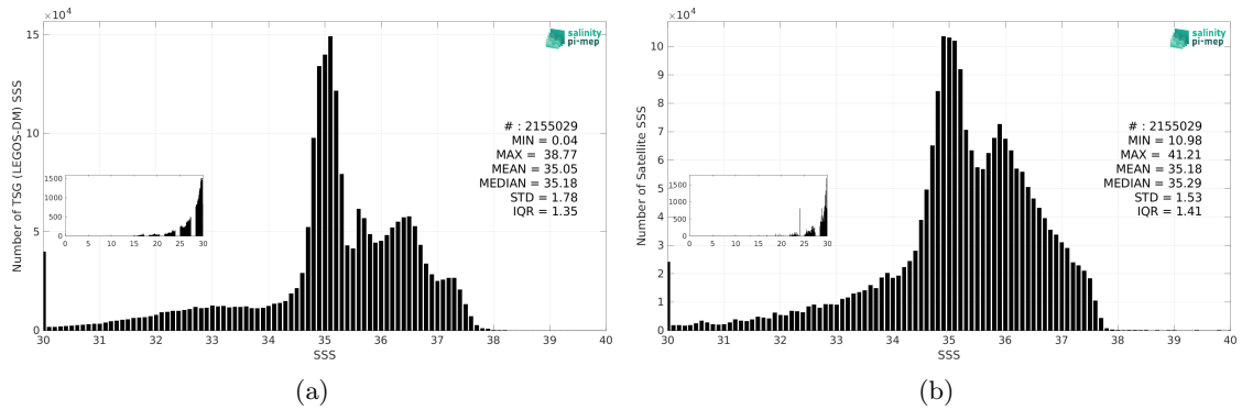
Figure 3: Histograms of SSS from TSG (LEGOS-DM) (a) and SMAP SSS L3 v6 - Monthly (RSS) (b) considering all match-up pairs per bins of 0.1 over the Atlantic Ocean Pi-MEP region and for the full satellite product period.
