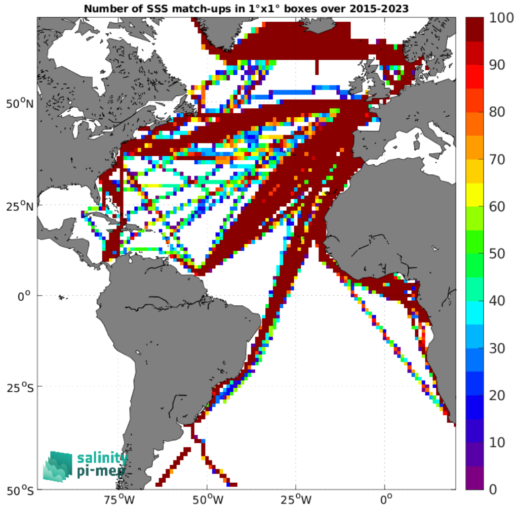
Figure 5: Number of SSS match-ups between TSG (LEGOS-DM) SSS and the SMAP SSS L3 v6 - Monthly (RSS) SSS product for the Atlantic Ocean Pi-MEP region over 1^\circ \times 1^\circ boxes and for the full satellite product period.
