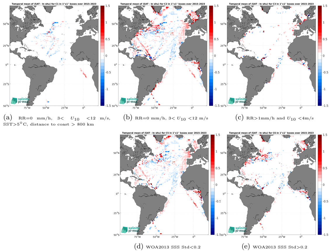
Figure 14: Temporal mean gridded over spatial boxes of size 1^\circ \times 1^\circ of \Delta\text{SSS} (SMAP SSS L3 v6 - Monthly (RSS) - TSG (LEGOS-DM)) for 5 different subdatasets corresponding to:RR=0 mm/h, 3 < U_{10} < 12 m/s, SST>5°C, distance to coast > 800 km (a), RR=0 mm/h, 3 < U_{10} < 12 m/s (b), RR>1mm/h and U_{10} < 4 m/s (c), WOA2013 SSS Std<0.2 (d), WOA2013 SSS Std>0.2 (e).
