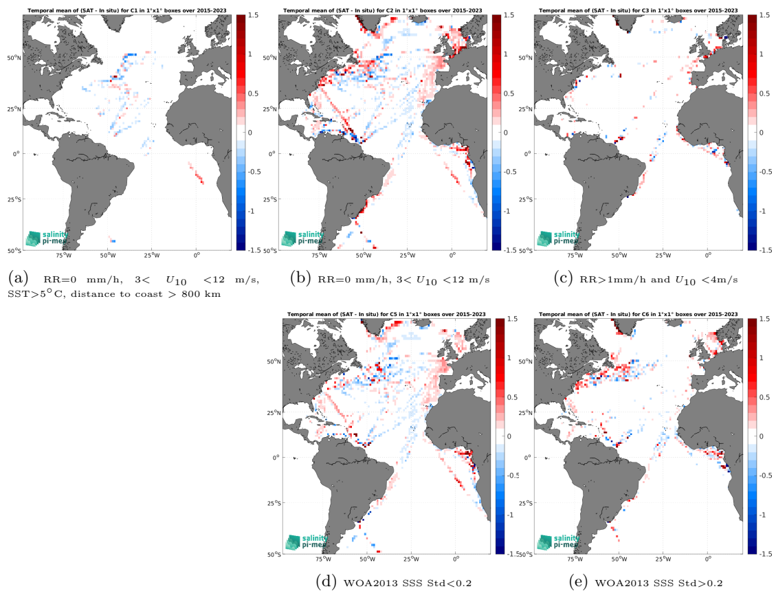
Figure 14: Temporal mean gridded over spatial boxes of size 1^\circ \times 1^\circ of \Delta\text{SSS} (SMAP SSS L3 v6 - Monthly (RSS) - TSG (LEGOS-DM)) for 5 different subdatasets corresponding to:RR=0 mm/h, 3 < U_{10} < 12 m/s, SST>5°C, distance to coast > 800 km (a), RR=0 mm/h, 3 < U_{10} < 12 m/s (b), RR>1mm/h and U_{10} < 4 m/s (c), WOA2013 SSS Std<0.2 (d), WOA2013 SSS Std>0.2 (e).
