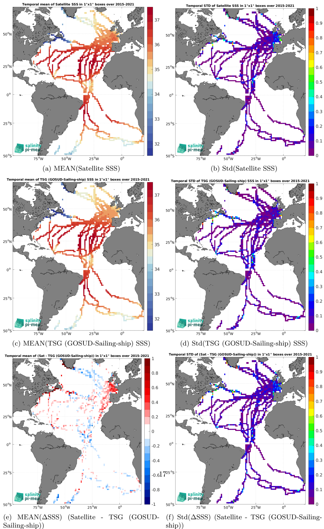
Figure 7: Temporal mean (left) and Std (right) of SSS from SMAP SSS L3 v6 - Monthly (RSS) (top), TSG (GOSUD-Sailing-ship) (middle), and of \Delta\text{SSS} (Satellite - TSG (GOSUD-Sailing-ship)). Only match-up pairs are used to generate these maps.
