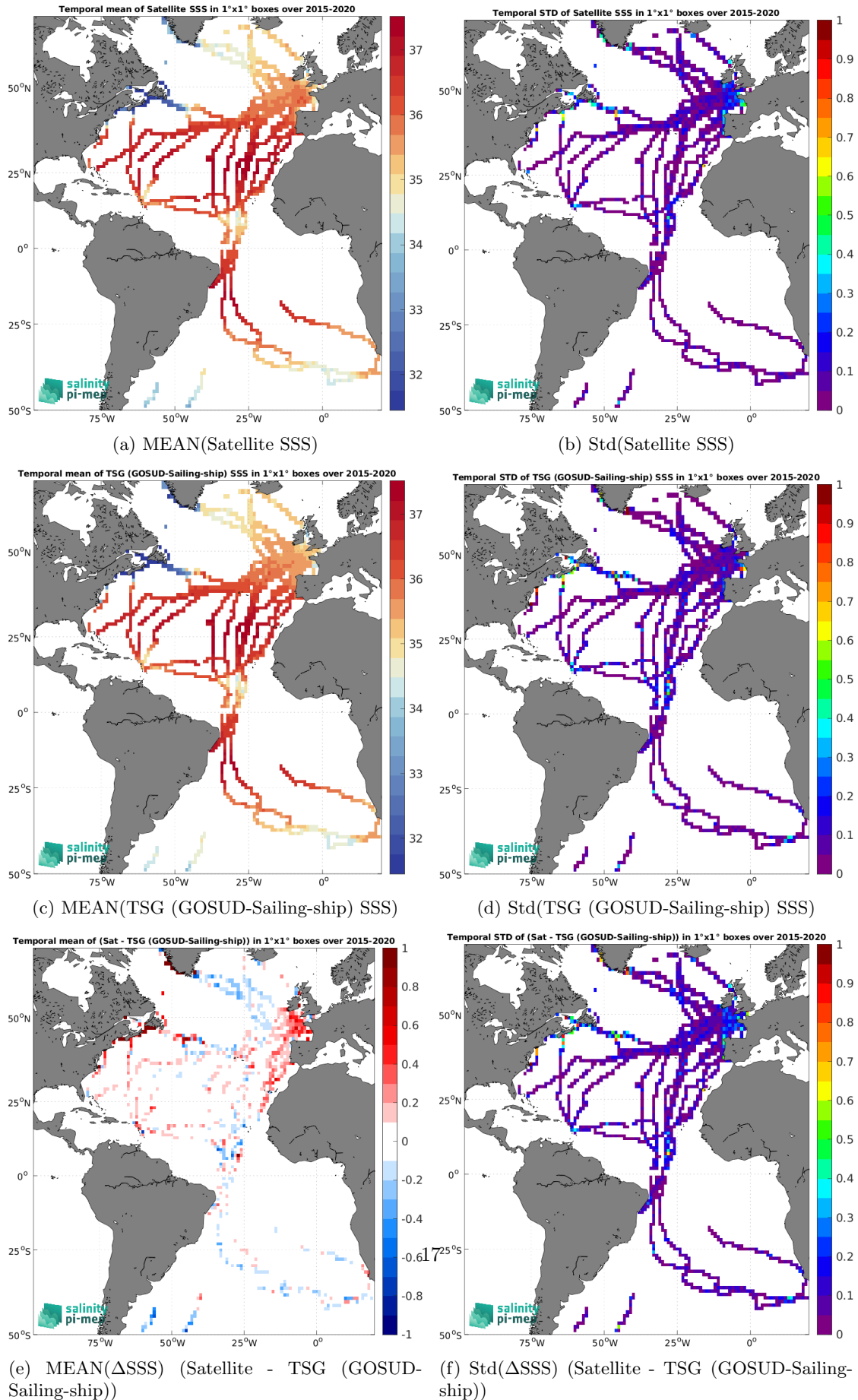
Figure 7: Temporal mean (left) and Std (right) of SSS from SMAP SSS L3 v6 - Monthly (RSS) (top), TSG (GOSUD-Sailing-ship) (middle), and of \Delta SSS (Satellite - TSG (GOSUD-Sailing-ship)). Only match-up pairs are used to generate these maps.
