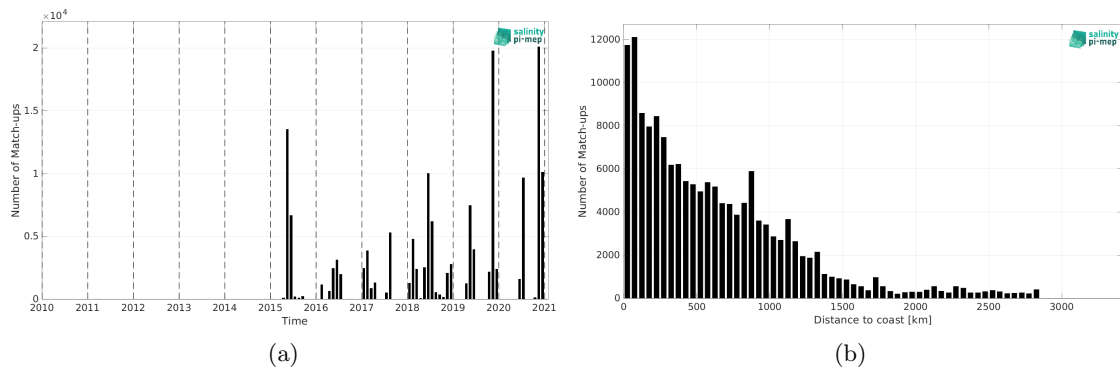
Figure 2: Number of match-ups between TSG (GOSUD-Sailing-ship) and SMAP SSS L3 v6 - Monthly (RSS) SSS as a function of time (a) and as function of the distance to coast (b) over the Atlantic Ocean Pi-MEP region and for the full satellite product period.
