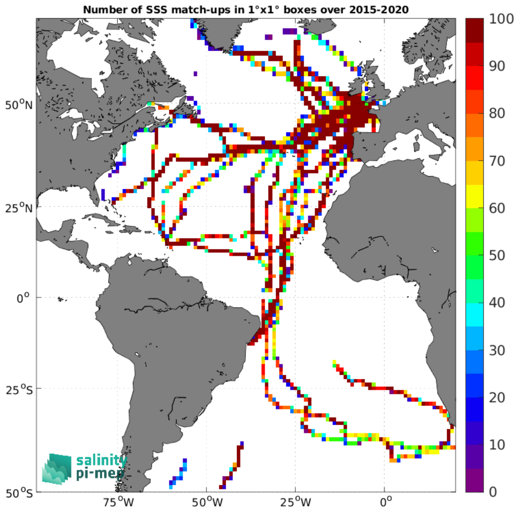
Figure 5: Number of SSS match-ups between TSG (GOSUD-Sailing-ship) SSS and the SMAP SSS L3 v6 - Monthly (RSS) SSS product for the Atlantic Ocean Pi-MEP region over 1^\circ \times 1^\circ boxes and for the full satellite product period.
