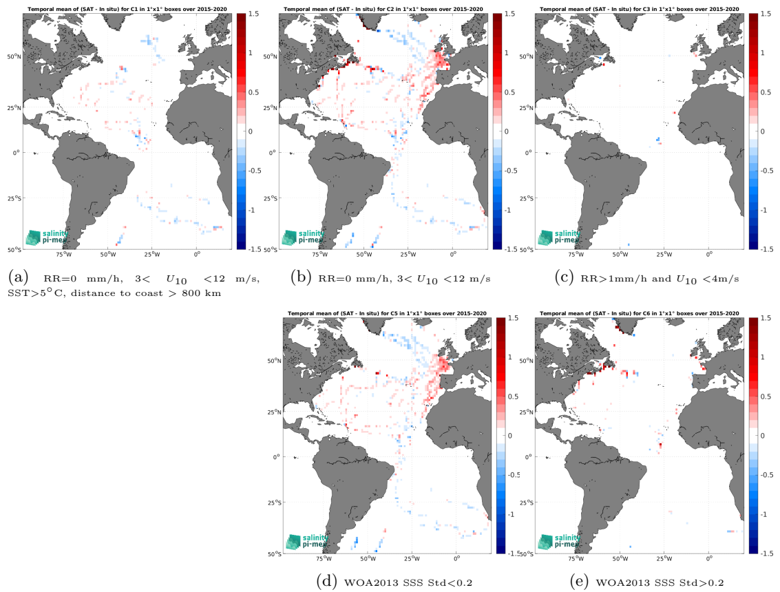
Figure 14: Temporal mean gridded over spatial boxes of size 1^\circ \times 1^\circ of \Delta\text{SSS} (SMAP SSS L3 v6 - Monthly (RSS) - TSG (GOSUD-Sailing-ship)) for 5 different subdatasets corresponding to:RR=0 mm/h, 3 < U_{10} < 12 m/s, SST>5°C, distance to coast > 800 km (a), RR=0 mm/h, 3 < U_{10} < 12 m/s (b), RR>1mm/h and U_{10} < 4 m/s (c), WOA2013 SSS Std<0.2 (d), WOA2013 SSS Std>0.2 (e).
