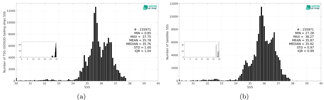
Figure 3: Histograms of SSS from TSG (GOSUD-Sailing-ship) (a) and SMAP SSS L3 v6 - Monthly (RSS) (b) considering all match-up pairs per bins of 0.1 over the Atlantic Ocean Pi-MEP region and for the full satellite product period.
