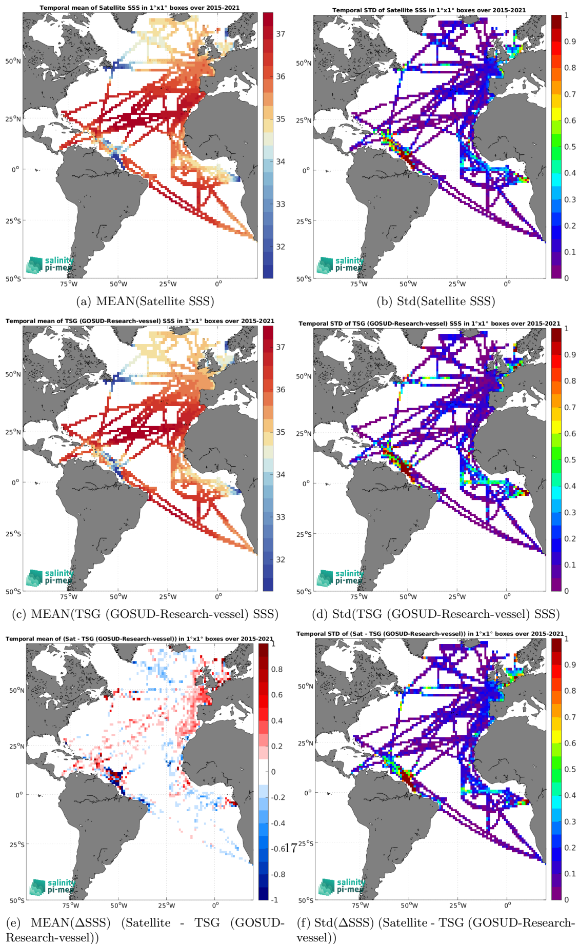
Figure 7: Temporal mean (left) and Std (right) of SSS from SMAP SSS L3 v6 - Monthly (RSS) (top), TSG (GOSUD-Research-vessel) (middle), and of \Delta SSS (Satellite - TSG (GOSUD-Research-vessel)). Only match-up pairs are used to generate these maps.
