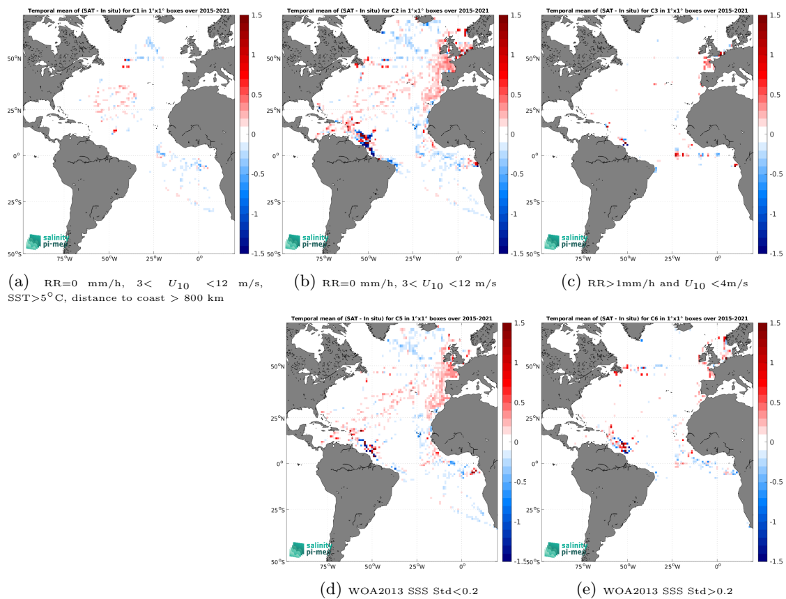
Figure 14: Temporal mean gridded over spatial boxes of size 1^\circ \times 1^\circ of \Delta\text{SSS} (SMAP SSS L3 v6 - Monthly (RSS) - TSG (GOSUD-Research-vessel)) for 5 different subdatasets corresponding to:RR=0 mm/h, 3 < U_{10} < 12 m/s, SST >5^\circ\text{C} , distance to coast > 800 km (a), RR=0 mm/h, 3 < U_{10} < 12 m/s (b), RR >1 mm/h and U_{10} < 4 m/s (c), WOA2013 SSS Std <0.2 (d), WOA2013 SSS Std >0.2 (e).
