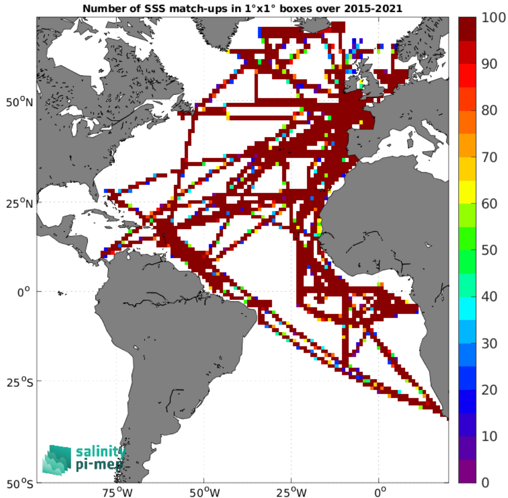
Figure 5: Number of SSS match-ups between TSG (GOSUD-Research-vessel) SSS and the SMAP SSS L3 v6 - Monthly (RSS) SSS product for the Atlantic Ocean Pi-MEP region over 1^\circ \times 1^\circ boxes and for the full satellite product period.
