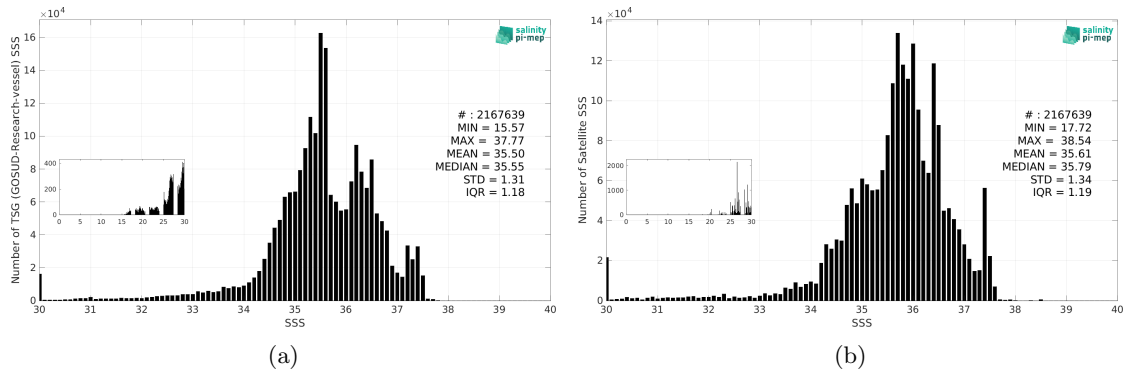
Figure 3: Histograms of SSS from TSG (GOSUD-Research-vessel) (a) and SMAP SSS L3 v6 - Monthly (RSS) (b) considering all match-up pairs per bins of 0.1 over the Atlantic Ocean Pi-MEP region and for the full satellite product period.
