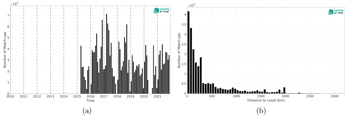
Figure 2: Number of match-ups between TSG (GOSUD-Research-vessel) and SMAP SSS L3 v6 - Monthly (RSS) SSS as a function of time (a) and as function of the distance to coast (b) over the Atlantic Ocean Pi-MEP region and for the full satellite product period.
