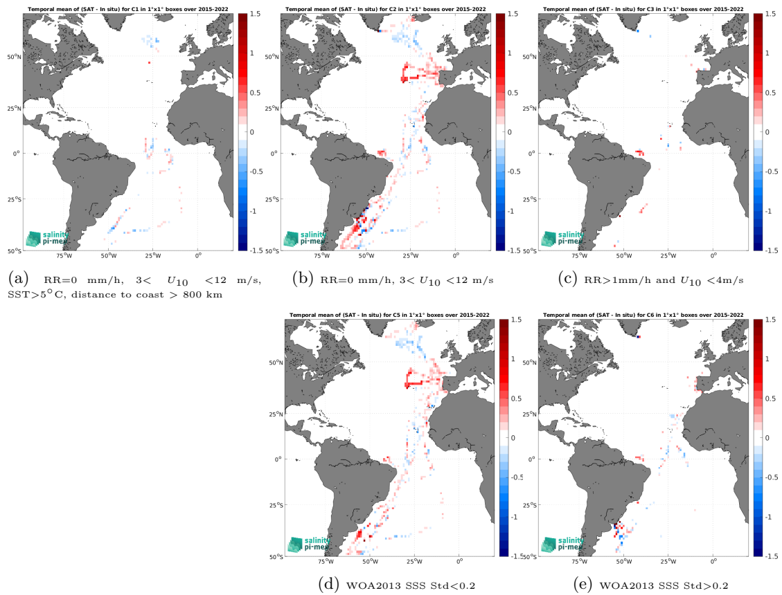
Figure 14: Temporal mean gridded over spatial boxes of size 1^\circ \times 1^\circ of \Delta\text{SSS} (SMAP SSS L3 v6 - Monthly (RSS) - TSG (CSIC-UTM)) for 5 different subdatasets corresponding to:RR=0 mm/h, 3 < U_{10} < 12 m/s, SST >5^\circ\text{C} , distance to coast > 800 km (a), RR=0 mm/h, 3 < U_{10} < 12 m/s (b), RR >1 mm/h and U_{10} < 4 m/s (c), WOA2013 SSS Std <0.2 (d), WOA2013 SSS Std >0.2 (e).
