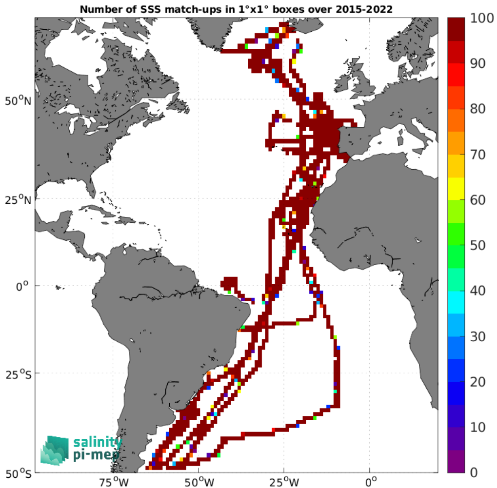
Figure 5: Number of SSS match-ups between TSG (CSIC-UTM) SSS and the SMAP SSS L3 v6 - Monthly (RSS) SSS product for the Atlantic Ocean Pi-MEP region over 1°×1° boxes and for the full satellite product period.
