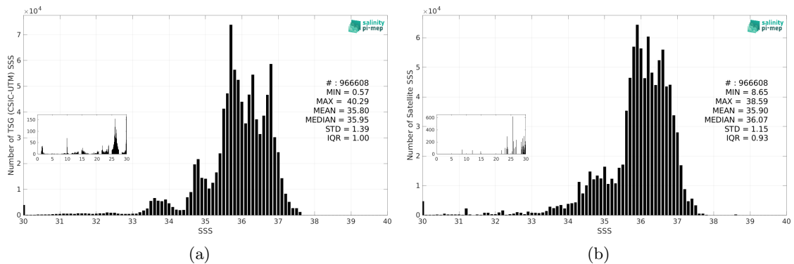
Figure 3: Histograms of SSS from TSG (CSIC-UTM) (a) and SMAP SSS L3 v6 - Monthly (RSS) (b) considering all match-up pairs per bins of 0.1 over the Atlantic Ocean Pi-MEP region and for the full satellite product period.
