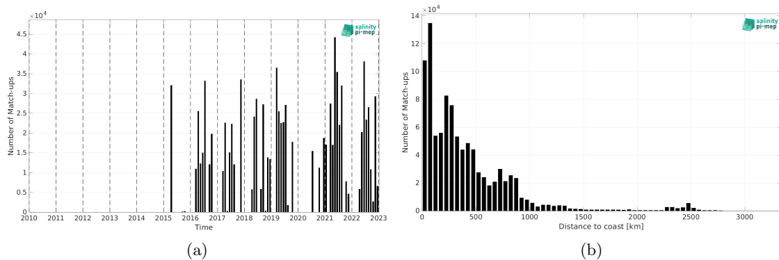
Figure 2: Number of match-ups between TSG (CSIC-UTM) and SMAP SSS L3 v6 - Monthly (RSS) SSS as a function of time (a) and as function of the distance to coast (b) over the Atlantic Ocean Pi-MEP region and for the full satellite product period.
