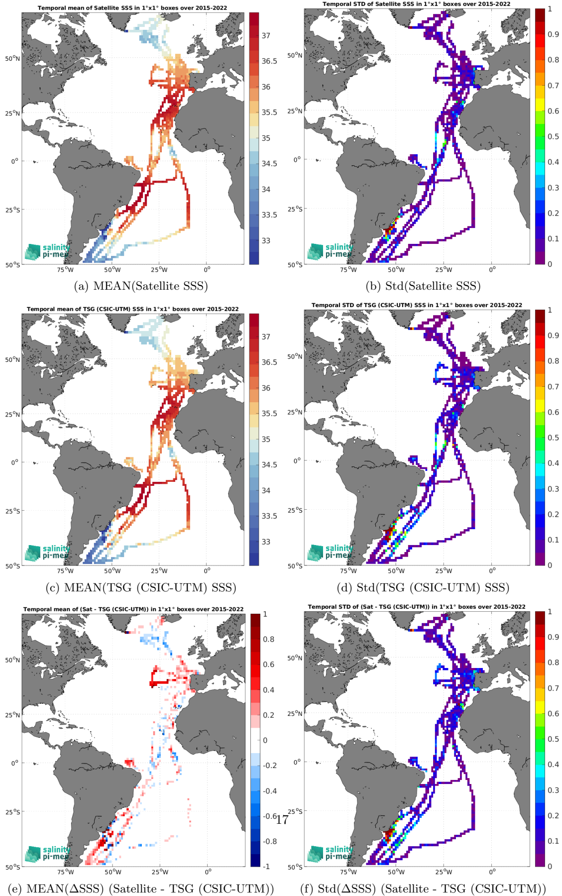
Figure 7: Temporal mean (left) and Std (right) of SSS from SMAP SSS L3 v6 - Monthly (RSS) (top), TSG (CSIC-UTM) (middle), and of \Delta SSS (Satellite - TSG (CSIC-UTM)). Only match-up pairs are used to generate these maps.
