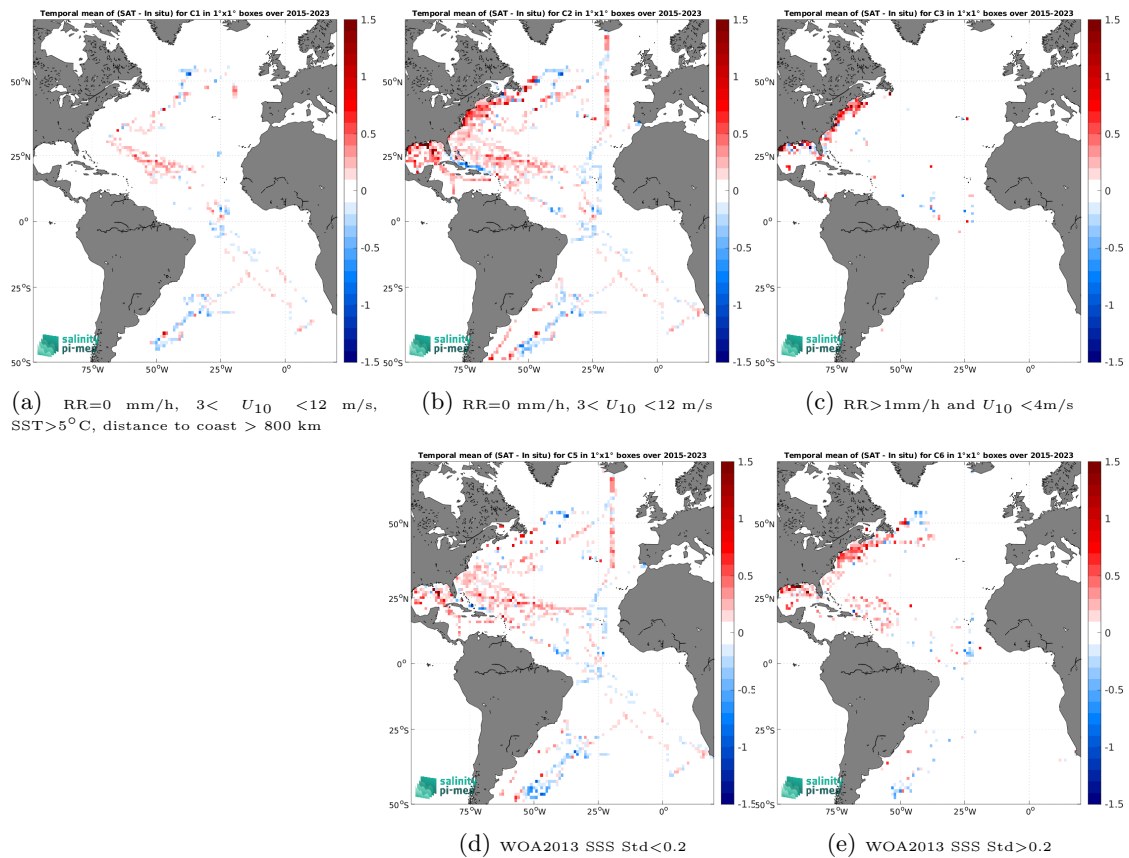
Figure 14: Temporal mean gridded over spatial boxes of size 1^\circ \times 1^\circ of \Delta\text{SSS} (SMAP SSS L3 v5.3 - 8-Day running (RSS) - TSG (SAMOS)) for 5 different subdatasets corresponding to:RR=0 mm/h, 3 < U_{10} < 12 m/s, SST>5°C, distance to coast > 800 km (a), RR=0 mm/h, 3 < U_{10} < 12 m/s (b), RR>1mm/h and U_{10} < 4 m/s (c), WOA2013 SSS Std<0.2 (d), WOA2013 SSS Std>0.2 (e).
