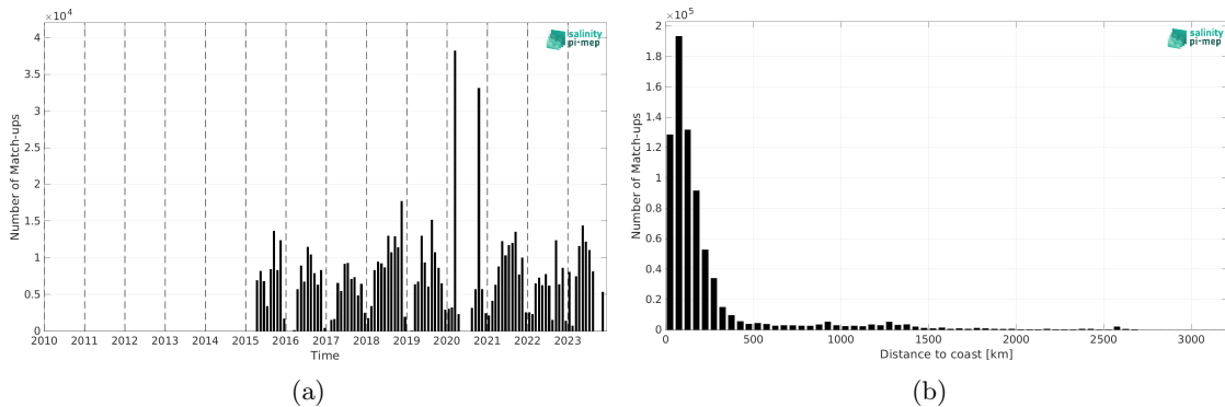
Figure 2: Number of match-ups between TSG (SAMOS) and SMAP SSS L3 v5.3 - 8-Day running (RSS) SSS as a function of time (a) and as function of the distance to coast (b) over the Atlantic Ocean Pi-MEP region and for the full satellite product period.
