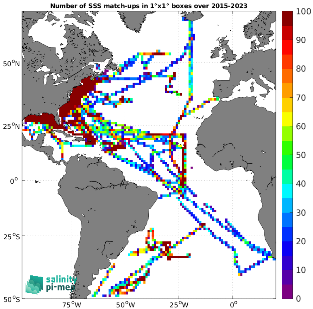
Figure 5: Number of SSS match-ups between TSG (SAMOS) SSS and the SMAP SSS L3 v5.3 - 8-Day running (RSS) SSS product for the Atlantic Ocean Pi-MEP region over 1^{\circ} \times 1^{\circ} boxes and for the full satellite product period.
