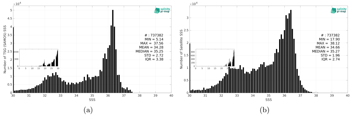
Figure 3: Histograms of SSS from TSG (SAMOS) (a) and SMAP SSS L3 v5.3 - 8-Day running (RSS) (b) considering all match-up pairs per bins of 0.1 over the Atlantic Ocean Pi-MEP region and for the full satellite product period.
