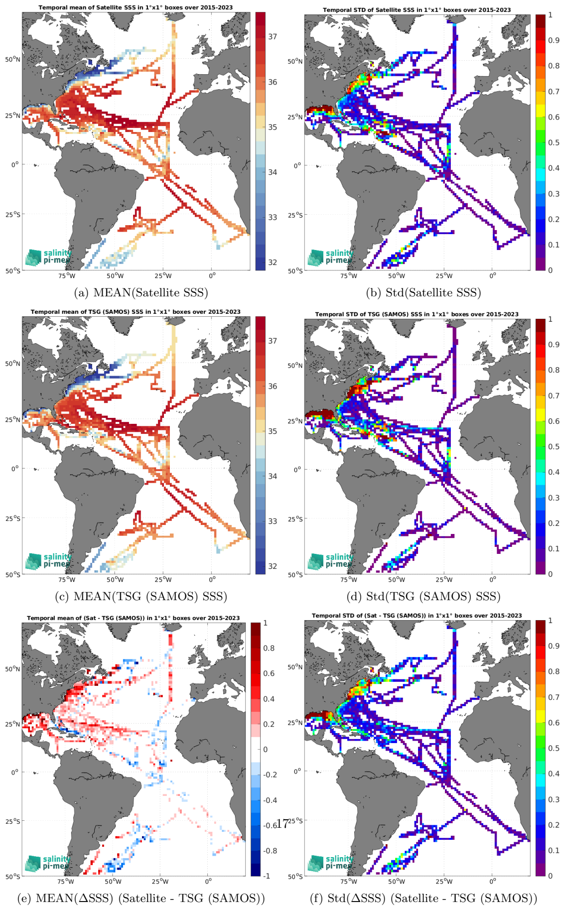
Figure 7: Temporal mean (left) and Std (right) of SSS from SMAP SSS L3 v5.3 - 8-Day running (RSS) (top), TSG (SAMOS) (middle), and of \Delta SSS (Satellite - TSG (SAMOS)). Only match-up pairs are used to generate these maps.
