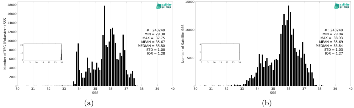
Figure 3: Histograms of SSS from TSG (Polarstern) (a) and SMAP SSS L3 v5.3 - 8-Day running (RSS) (b) considering all match-up pairs per bins of 0.1 over the Atlantic Ocean Pi-MEP region and for the full satellite product period.
