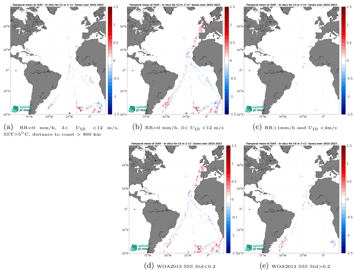
Figure 14: Temporal mean gridded over spatial boxes of size 1^\circ \times 1^\circ of \Delta\text{SSS} (SMAP SSS L3 v5.3 - 8-Day running (RSS) - TSG (Polarstern)) for 5 different subdatasets corresponding to:RR=0 mm/h, 3 < U_{10} < 12 m/s, SST >5^\circ\text{C} , distance to coast > 800 km (a), RR=0 mm/h, 3 < U_{10} < 12 m/s (b), RR >1 mm/h and U_{10} < 4 m/s (c), WOA2013 SSS Std <0.2 (d), WOA2013 SSS Std >0.2 (e).
