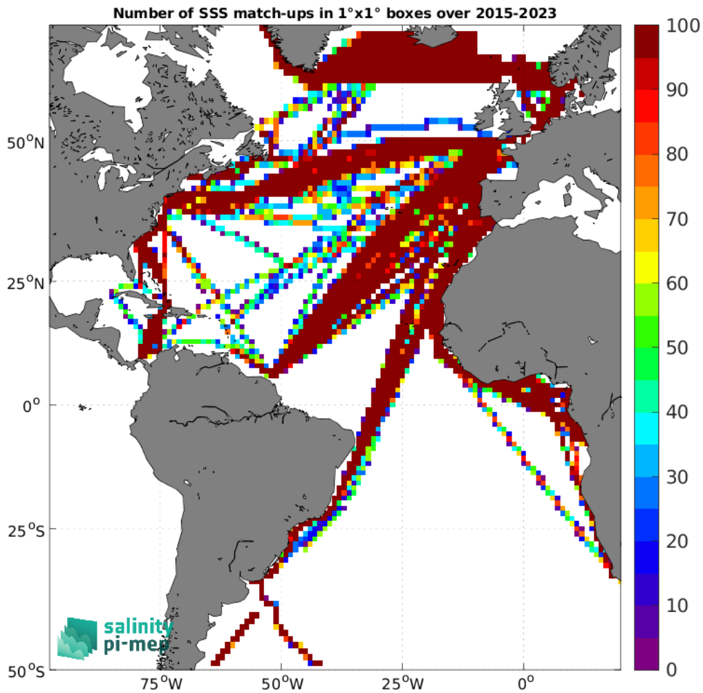
Figure 5: Number of SSS match-ups between TSG (LEGOS-DM) SSS and the SMAP SSS L3 v5.3 - 8-Day running (RSS) SSS product for the Atlantic Ocean Pi-MEP region over 1^\circ \times 1^\circ boxes and for the full satellite product period.
