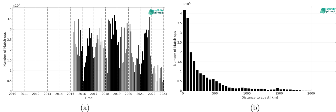
Figure 2: Number of match-ups between TSG (LEGOS-DM) and SMAP SSS L3 v5.3 - 8-Day running (RSS) SSS as a function of time (a) and as function of the distance to coast (b) over the Atlantic Ocean Pi-MEP region and for the full satellite product period.
