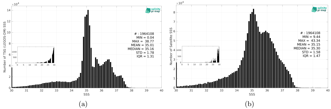
Figure 3: Histograms of SSS from TSG (LEGOS-DM) (a) and SMAP SSS L3 v5.3 - 8-Day running (RSS) (b) considering all match-up pairs per bins of 0.1 over the Atlantic Ocean Pi-MEP region and for the full satellite product period.
