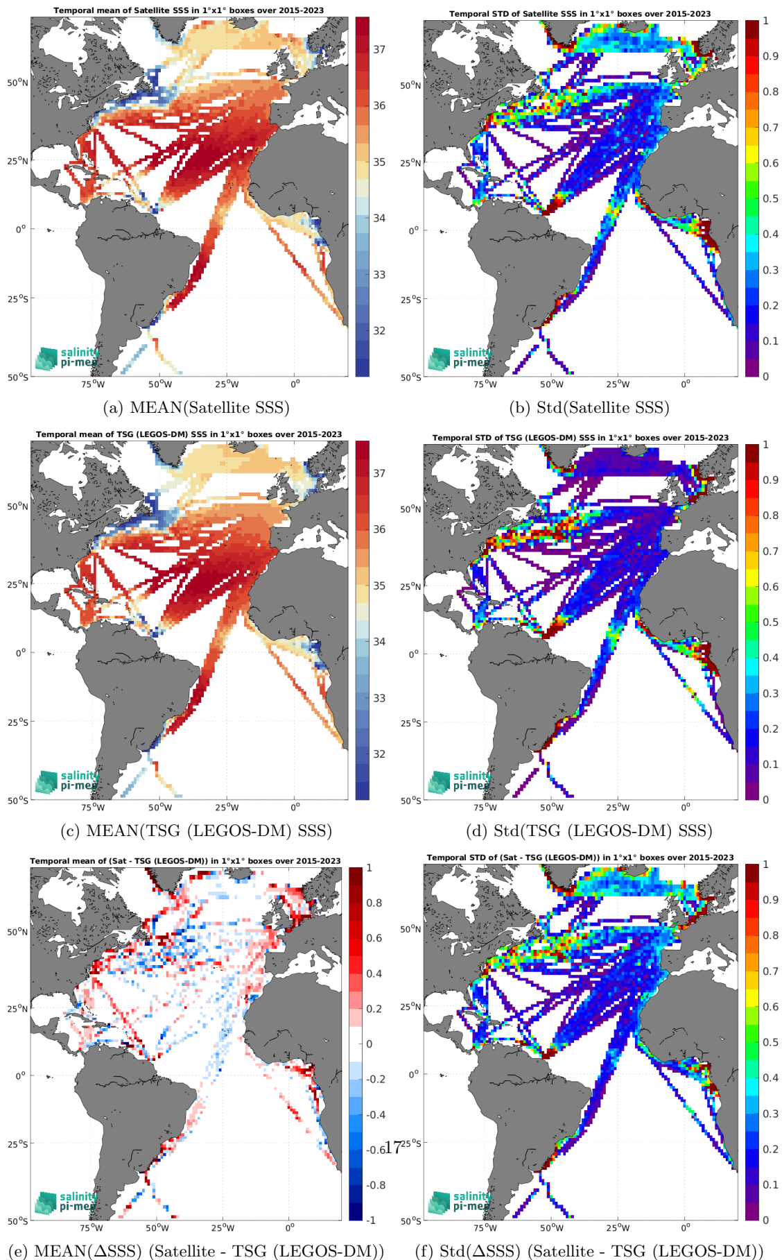
Figure 7: Temporal mean (left) and Std (right) of SSS from SMAP SSS L3 v5.3 - 8-Day running (RSS) (top), TSG (LEGOS-DM) (middle), and of \Delta SSS (Satellite - TSG (LEGOS-DM)). Only match-up pairs are used to generate these maps.
