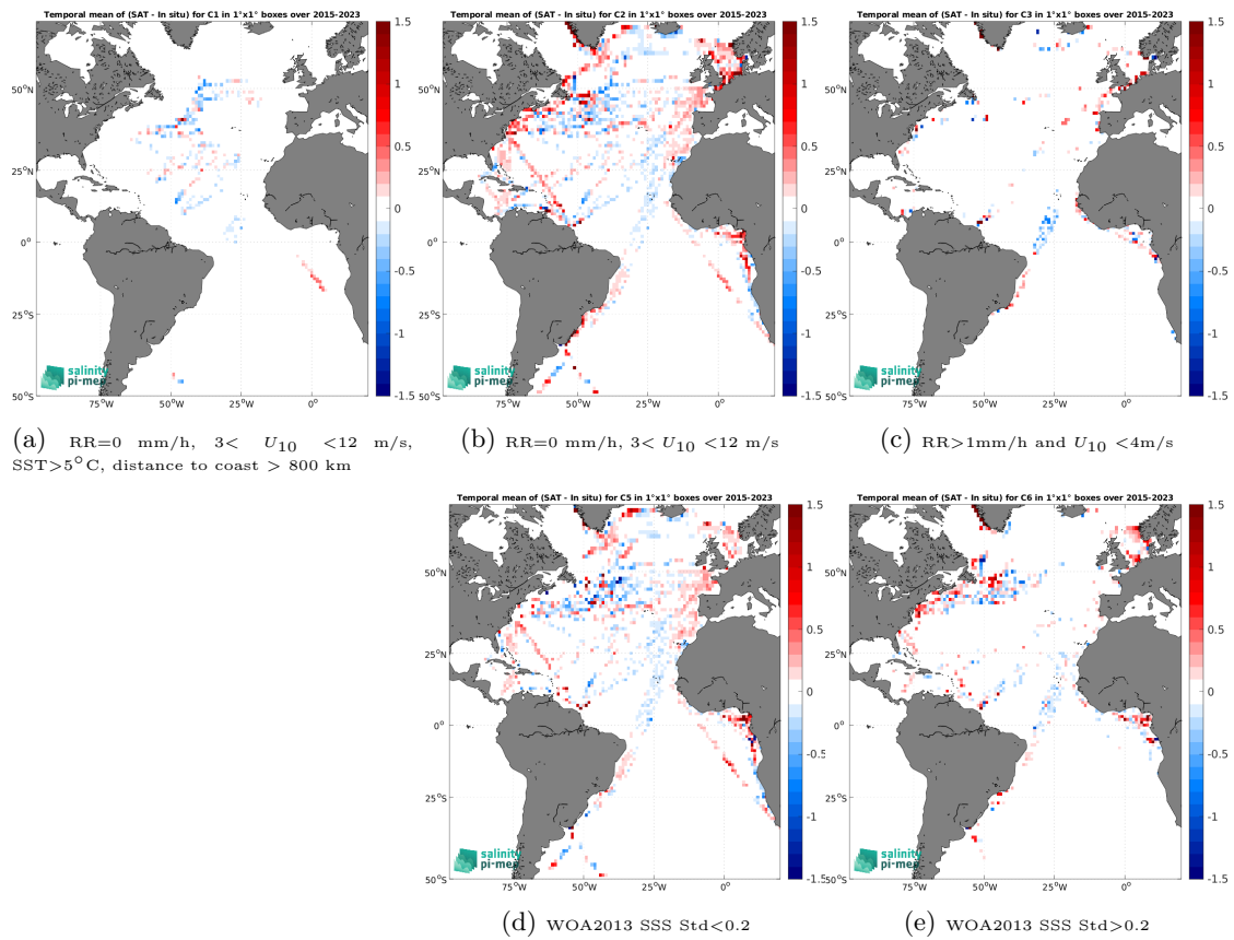
Figure 14: Temporal mean gridded over spatial boxes of size 1^\circ \times 1^\circ of \Delta\text{SSS} (SMAP SSS L3 v5.3 - 8-Day running (RSS) - TSG (LEGOS-DM)) for 5 different subdatasets corresponding to:RR=0 mm/h, 3 < U_{10} < 12 m/s, SST >5^\circ\text{C} , distance to coast > 800 km (a), RR=0 mm/h, 3 < U_{10} < 12 m/s (b), RR >1 mm/h and U_{10} < 4 m/s (c), WOA2013 SSS Std <0.2 (d), WOA2013 SSS Std >0.2 (e).
