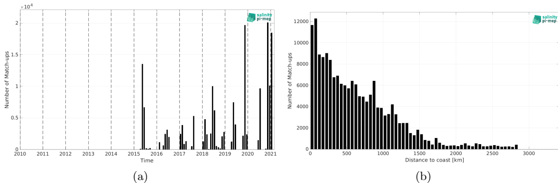
Figure 2: Number of match-ups between TSG (GOSUD-Sailing-ship) and SMAP SSS L3 v5.3 - 8-Day running (RSS) SSS as a function of time (a) and as function of the distance to coast (b) over the Atlantic Ocean Pi-MEP region and for the full satellite product period.
