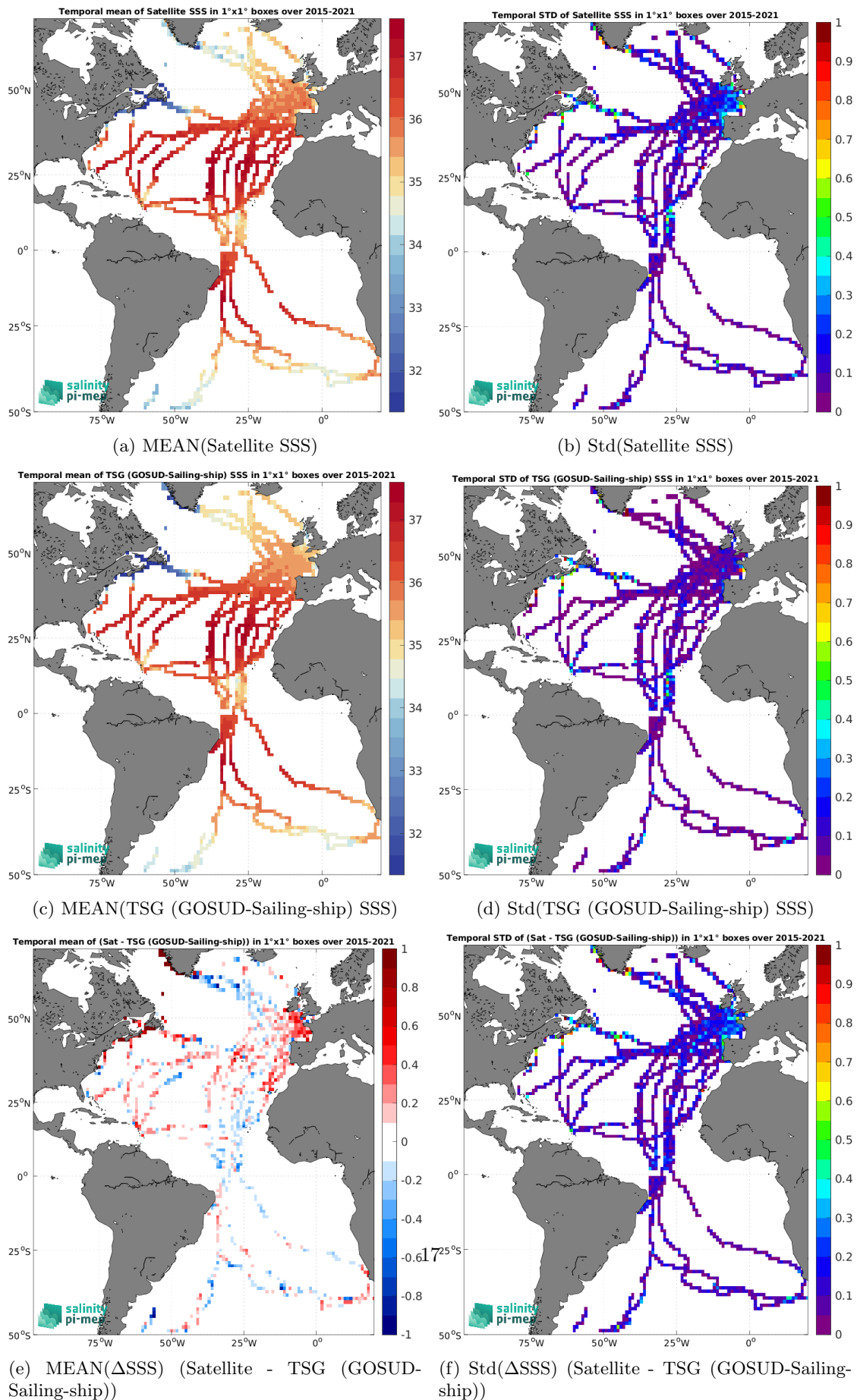
Figure 7: Temporal mean (left) and Std (right) of SSS from SMAP SSS L3 v5.3 - 8-Day running (RSS) (top), TSG (GOSUD-Sailing-ship) (middle), and of \Delta SSS (Satellite - TSG (GOSUD-Sailing-ship)). Only match-up pairs are used to generate these maps.
