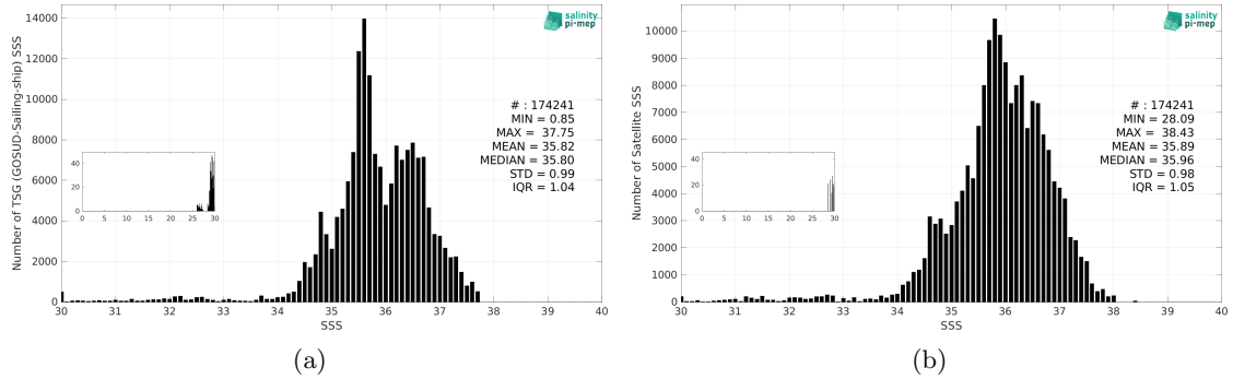
Figure 3: Histograms of SSS from TSG (GOSUD-Sailing-ship) (a) and SMAP SSS L3 v5.3 - 8-Day running (RSS) (b) considering all match-up pairs per bins of 0.1 over the Atlantic Ocean Pi-MEP region and for the full satellite product period.
