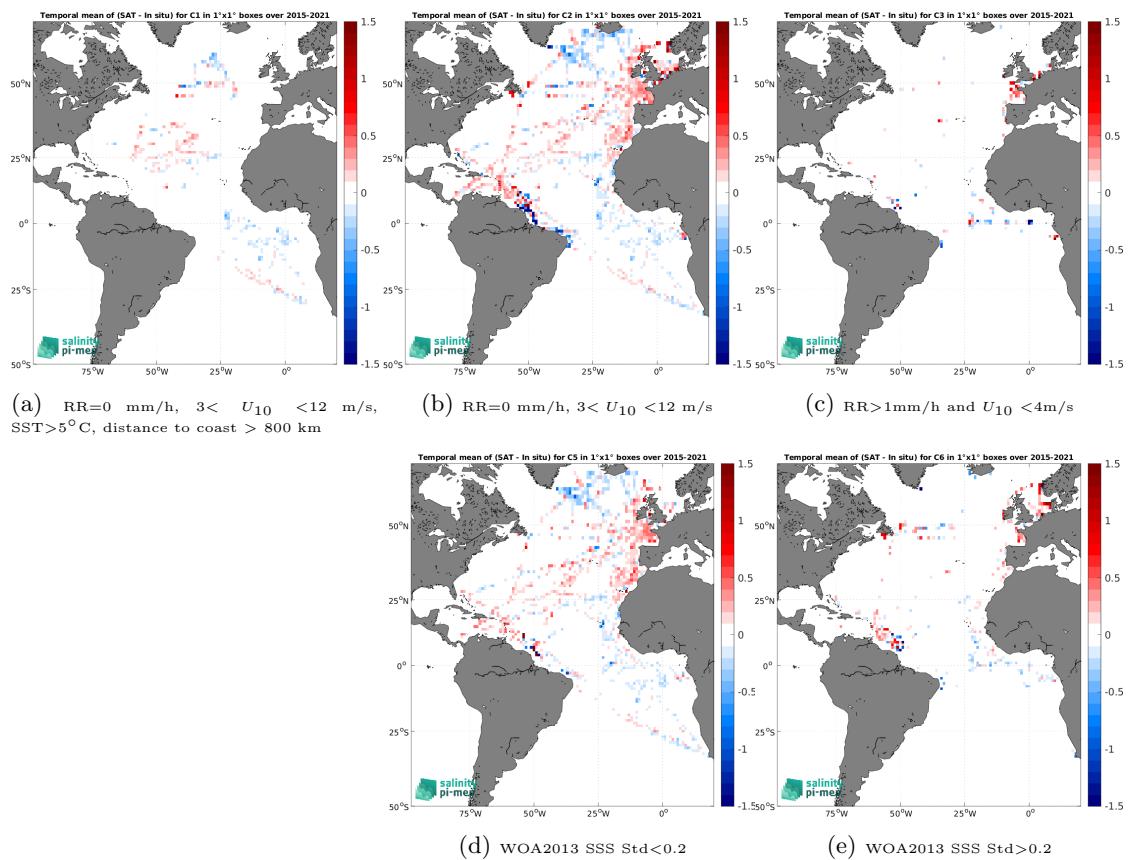
Figure 14: Temporal mean gridded over spatial boxes of size 1^\circ \times 1^\circ of \Delta\text{SSS} (SMAP SSS L3 v5.3 - 8-Day running (RSS) - TSG (GOSUD-Research-vessel)) for 5 different subdatasets corresponding to:RR=0 mm/h, 3 < U_{10} < 12 m/s, SST>5°C, distance to coast > 800 km (a), RR=0 mm/h, 3 < U_{10} < 12 m/s (b), RR>1mm/h and U_{10} < 4 m/s (c), WOA2013 SSS Std<0.2 (d), WOA2013 SSS Std>0.2 (e).
