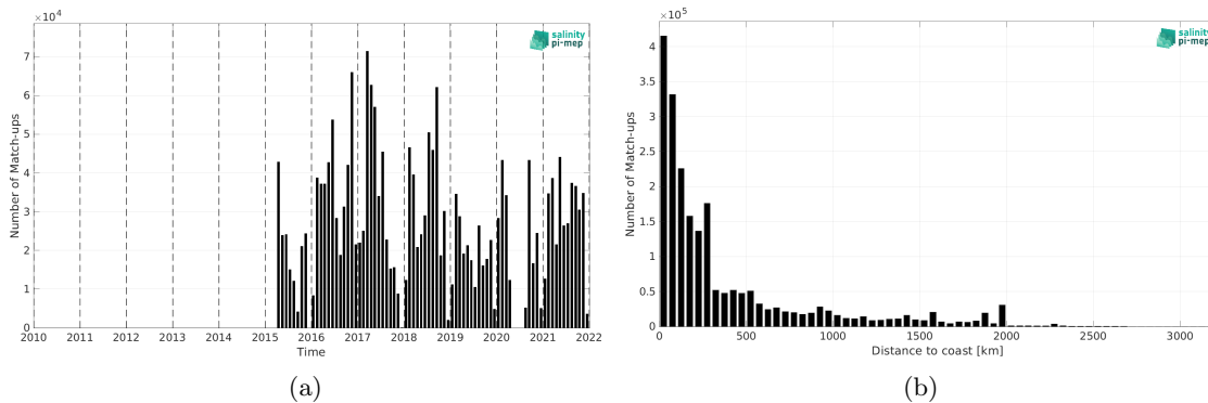
Figure 2: Number of match-ups between TSG (GOSUD-Research-vessel) and SMAP SSS L3 v5.3 - 8-Day running (RSS) SSS as a function of time (a) and as function of the distance to coast (b) over the Atlantic Ocean Pi-MEP region and for the full satellite product period.
