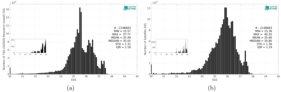
Figure 3: Histograms of SSS from TSG (GOSUD-Research-vessel) (a) and SMAP SSS L3 v5.3 - 8-Day running (RSS) (b) considering all match-up pairs per bins of 0.1 over the Atlantic Ocean Pi-MEP region and for the full satellite product period.
