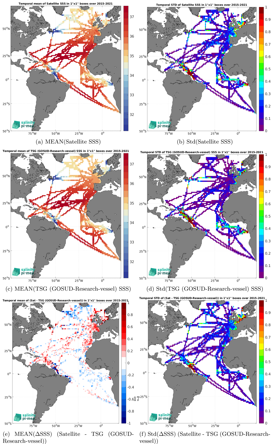
Figure 7: Temporal mean (left) and Std (right) of SSS from SMAP SSS L3 v5.3 - 8-Day running (RSS) (top), TSG (GOSUD-Research-vessel) (middle), and of \Delta SSS (Satellite - TSG (GOSUD-Research-vessel)). Only match-up pairs are used to generate these maps.
