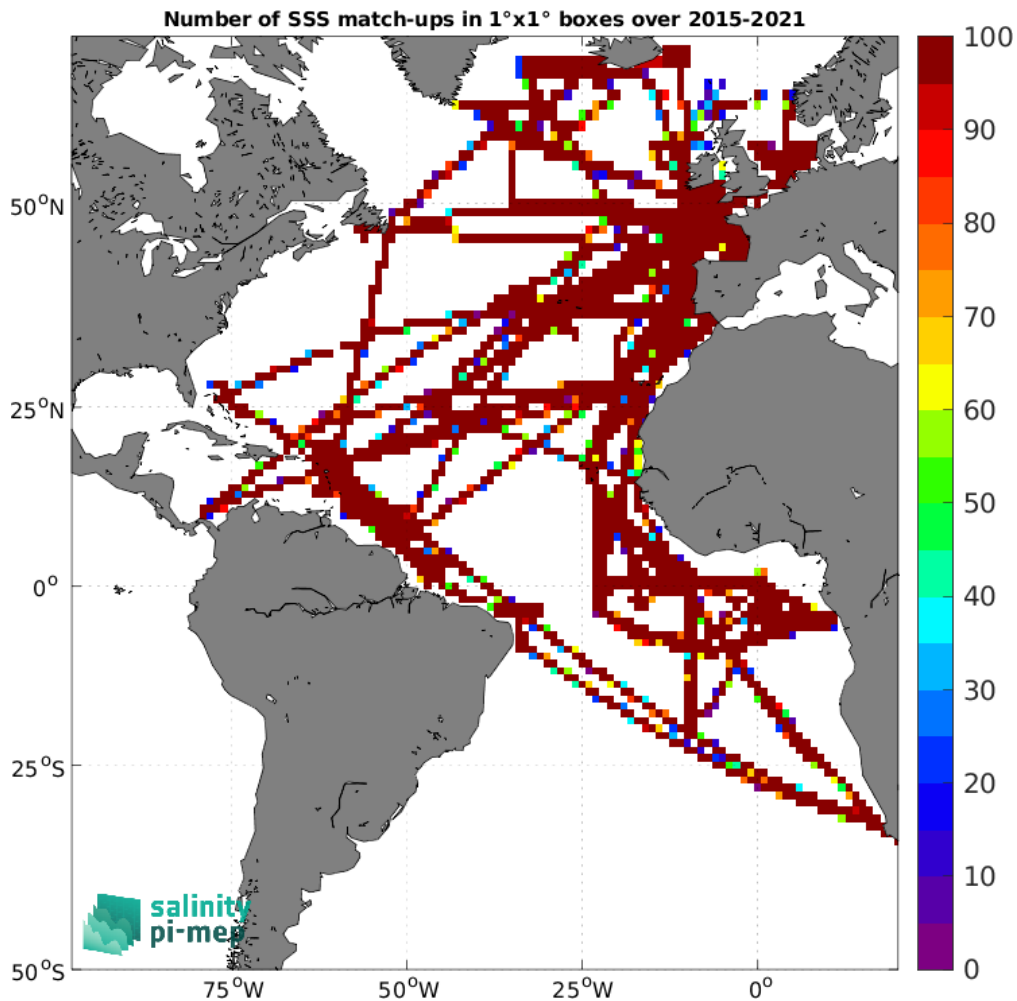
Figure 5: Number of SSS match-ups between TSG (GOSUD-Research-vessel) SSS and the SMAP SSS L3 v5.3 - 8-Day running (RSS) SSS product for the Atlantic Ocean Pi-MEP region over 1^\circ \times 1^\circ boxes and for the full satellite product period.
